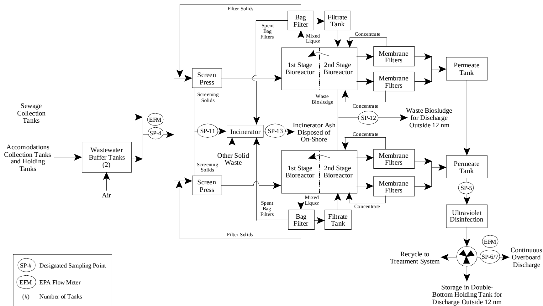
Figure 2-2. Hamworthy Treatment System, Island Princess
