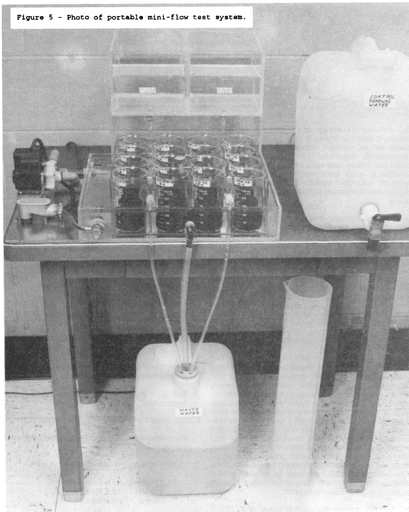
Figure B.1 Portable table top STIR system described in Benoit et al. (1993).
