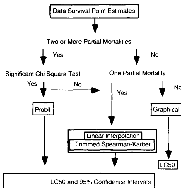
Figure 14.8 Decision tree for analysis of point estimate data.
