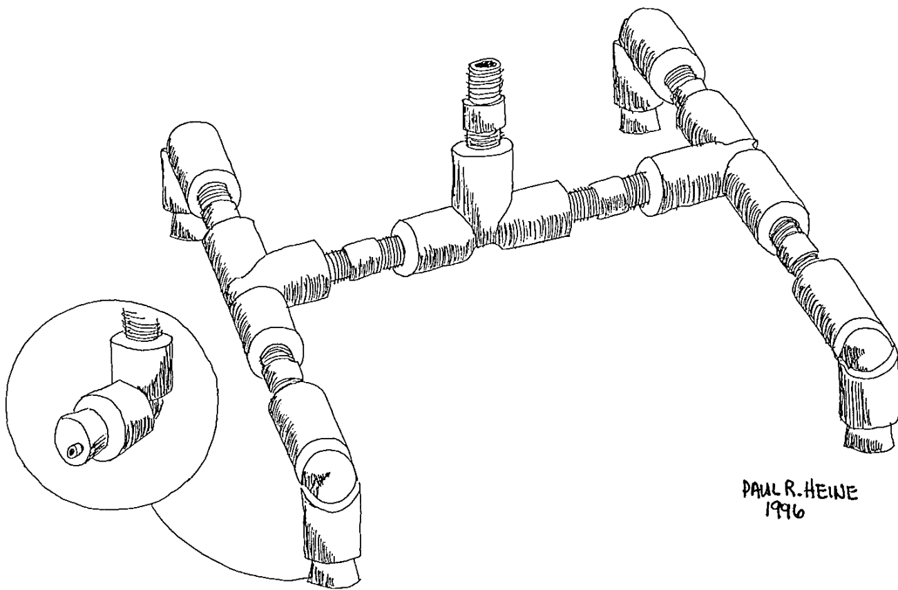
Figure A.5. Diagram of in-line flow splitter used to deliver overlying water in the sediment exposures of Lumbriculus variegatus (Brunson et al., 1998).
