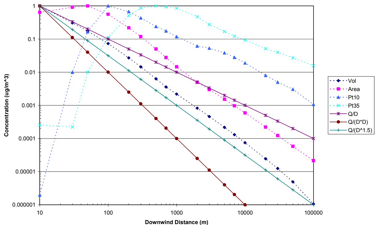
Figure 6. Concentration vs. Downwind Distance for AERMOD Annual Averages
