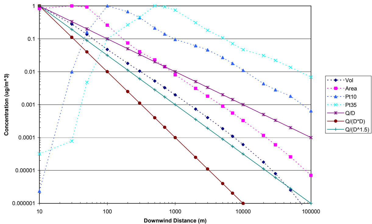
Figure 8. Concentration vs. Downwind Distance for AERMOD 24-hr Averages - Radial 9
