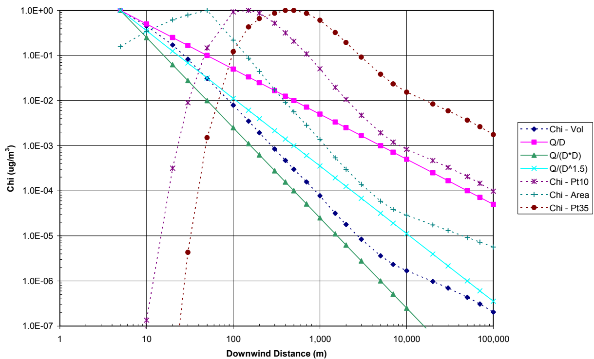
Figure 2. Chi vs. Downwind Distance - Convective Conditions
