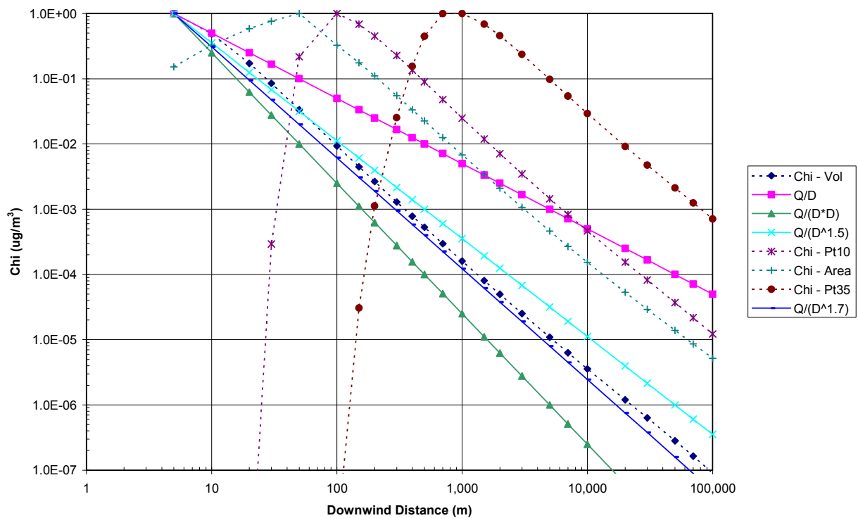
Figure 4. Concentration vs. Downwind Distance for AERMOD 1-hr Averages
