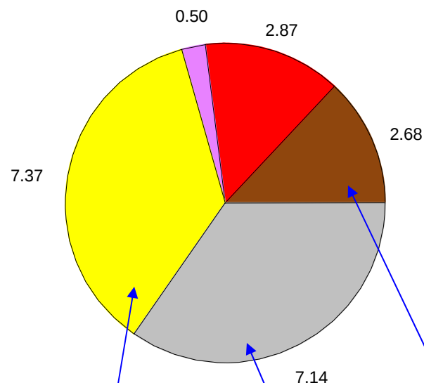
Dearborn airs_site_code=261630033 year=2003
