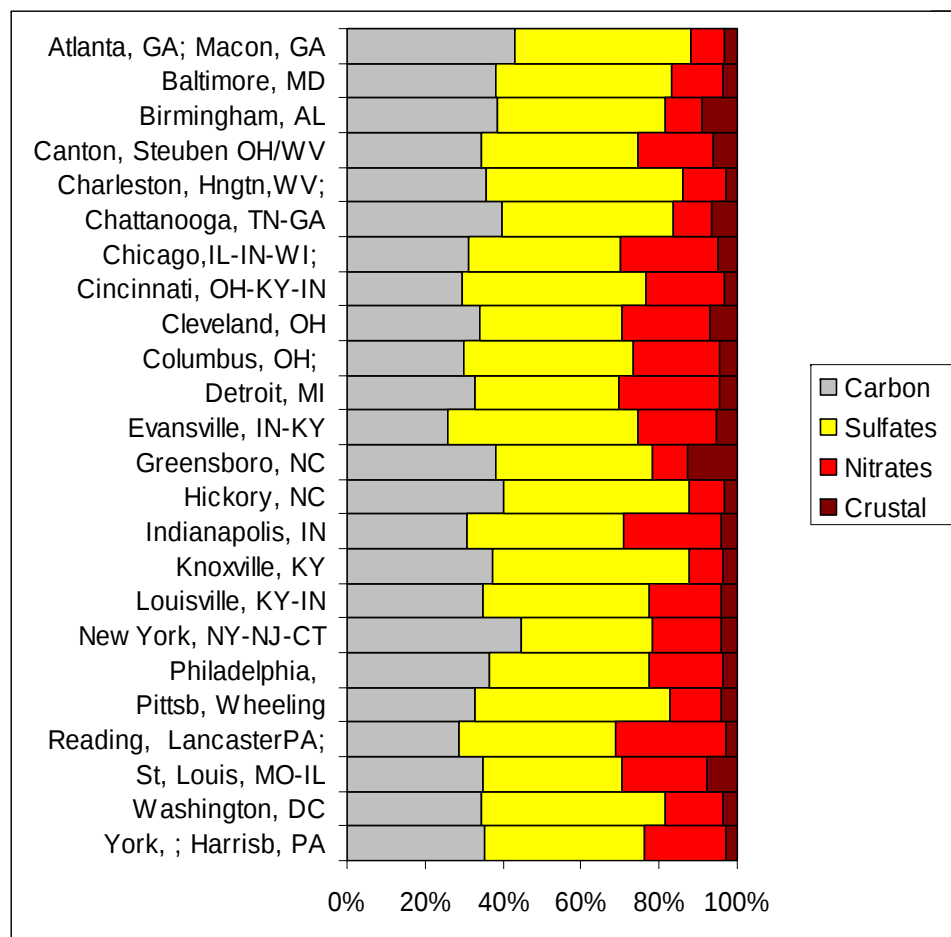
Estimated PM2.5 Composition
