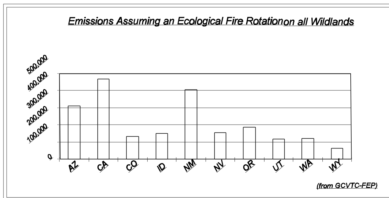
Figure 1: Emissions predicted for 10 states in the west if fire were to occur at historic frequencies in existing vegetation.
