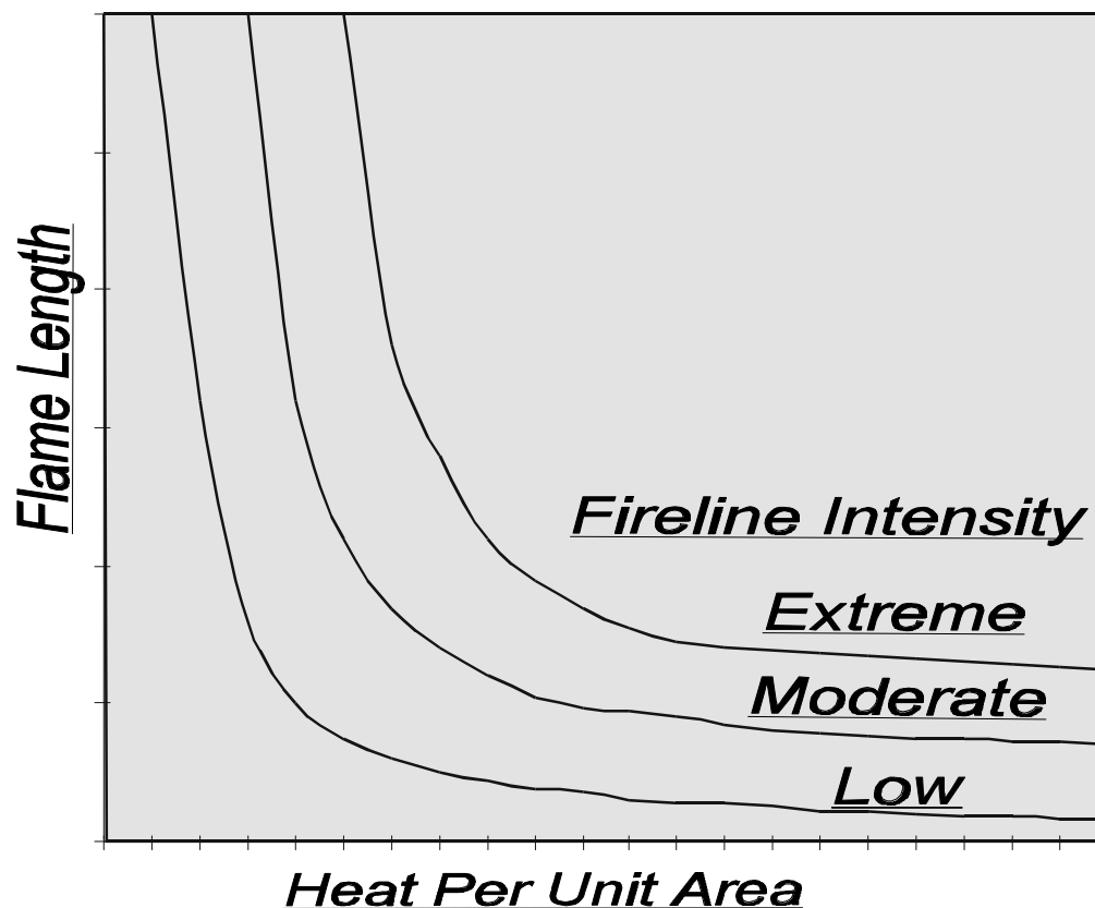
Figure 3: Fire behavior or fireline intensity is related to rate of spread, heat per unit area, and flame length.
