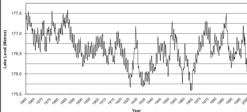
Figure 3. Actual water levels for Lakes Huron and Michigan. IGLD-International Great Lakes Datum. Zero for IGLD is Rimouski, Quebec, at the mouth of the St. Lawrence River. Water level elevations in the Great Lakes/St. Lawrence River system are measured above water level at this site.
