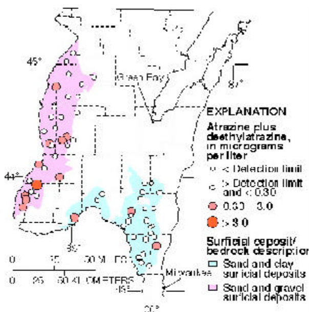
Figure 2. Atrazine concentrations in shallow groundwater were highest in areas with the most permeable surficial deposits.
