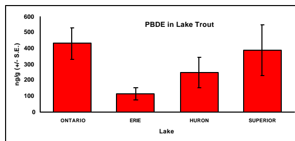
Figure 9. PBDE Levels in Great Lakes Lake Trout (1997) (ng/g per lipid weight \pm S.E., whole fish, age 6+ yrs)
