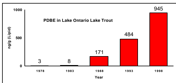
Figure 8. PBDE Trends in Lake Ontario Lake Trout (ng/g lipid weight \pm S.E., whole fish, age 6+ yrs)
