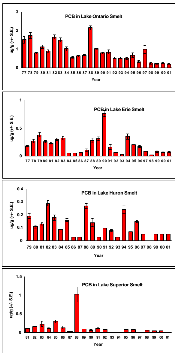
Figure 3. Total PCB Levels in Great Lakes Rainbow Smelt (1977-2001). (Canadian data \mu\text{g/g} wet weight \pm S.E., whole fish)
