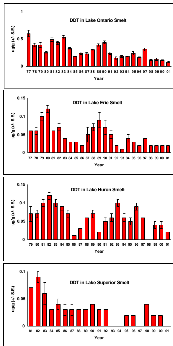
Figure 4. Total DDT Levels in Great Lakes Rainbow Smelt (1977-2001). (Canadian data \mu\text{g/g} wet weight \pm S.E., whole fish)
