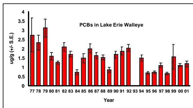
Figure 6. Total PCB Levels in Lake Erie Walleye (1977-2001). (Canadian data ug/g wet weight +/- S.E., ages 4+ - 6+)
