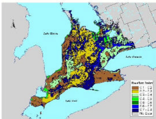
Figure 1. Base Flow Index based on geology
