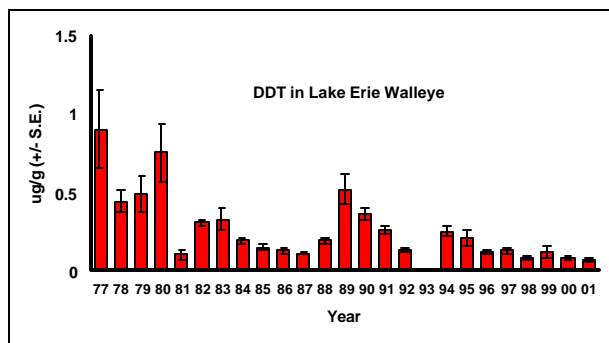
Figure 7. Total DDT Levels in Lake Erie Walleye (1977-2001). (Canadian data ug/g wet weight +/- S.E., ages 4+ - 6+)
