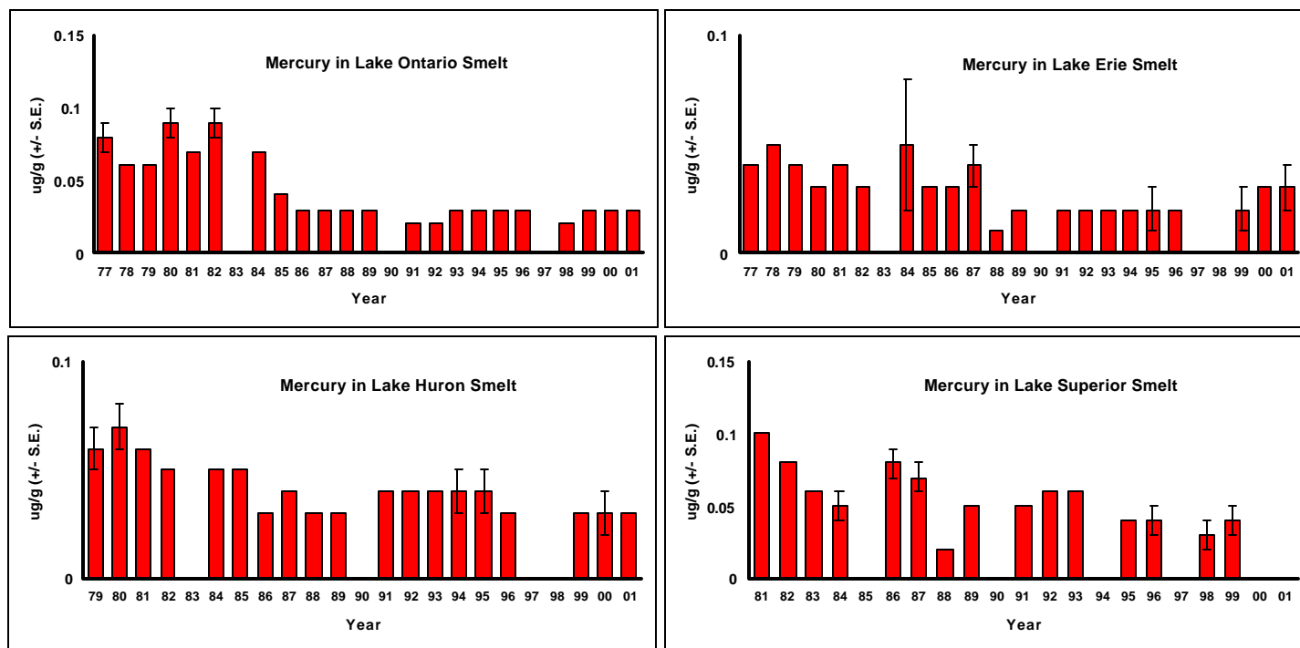
Figure 5. Total Mercury Levels in Great Lakes Rainbow Smelt (1977-2001). (Canadian data ug/g wet weight +/- S.E., whole fish)
