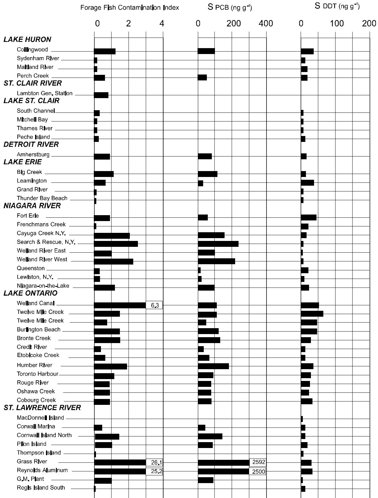
Figure 20 Forage Fish Contamination Index (FFCI) for young-of-the-year spottail shiners in the Great Lakes in 1993 or 1994, with relative contributions from PCBs and DDT. Wildlife Risk Level =1.
