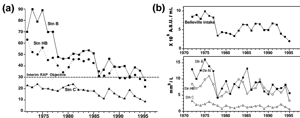
Figure 19 Phosphorus Concentrations in the Bay of Quinte
