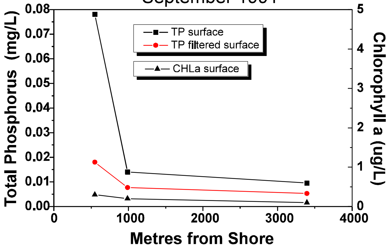
Figure 11 Phosphorus Gradient in Lake Ontario
