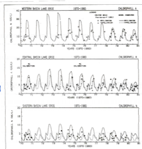
FIG. 10. Comparison of model predicted and 1970 to 1980 observed mean chlorophyll a - western, central, and eastern basins of Lake Erie.
