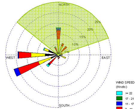
Jefferson Elementary School Composite Hourly Windrose on Sample Days (Sep. 28, 2009-Dec. 9, 2009)
