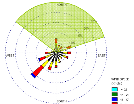
Jefferson Elementary School Composite Hourly Windrose Across Sampling Period (Aug. 23 - Dec. 9, 2009)
