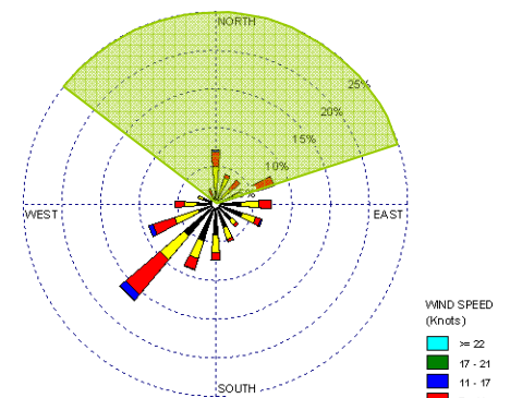
Jefferson Elementary School Composite Hourly Windrose Across Sampling Period (Aug. 23, 2009-Dec. 9, 2009)
