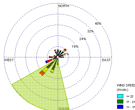
South Allegheny Middle/High School Composite Hourly Windrose on Sample Days (Aug. 5, 2009-Nov. 30, 2009)
