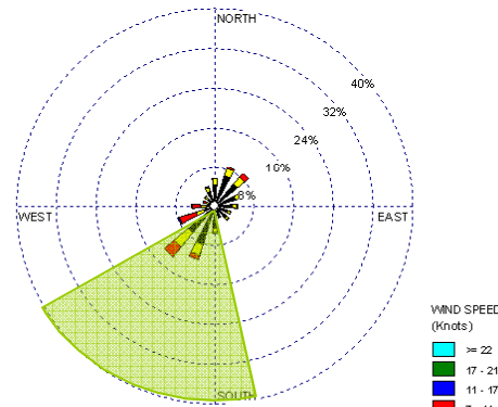
South Allegheny Middle/High School Composite Hourly Windrose Across Sampling Period (Aug. 5, 2009-Nov. 30, 2009)
