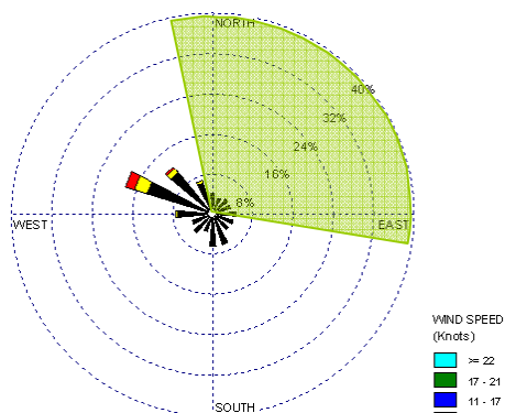
Clairton Educational Center Composite Hourly Windrose Across Sampling Period (Sep. 4, 2009-Dec. 21, 2009)
