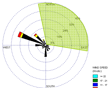
Clairton Educational Center Composite Hourly Windrose on Sample Days (Sep. 22, 2009-Nov. 21, 2009)
