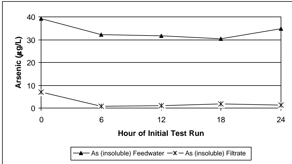
Figure 4-3. Insoluble Arsenic Concentrations For Initial Testing Period (no coagulation chemicals) (April 11, 2000)
