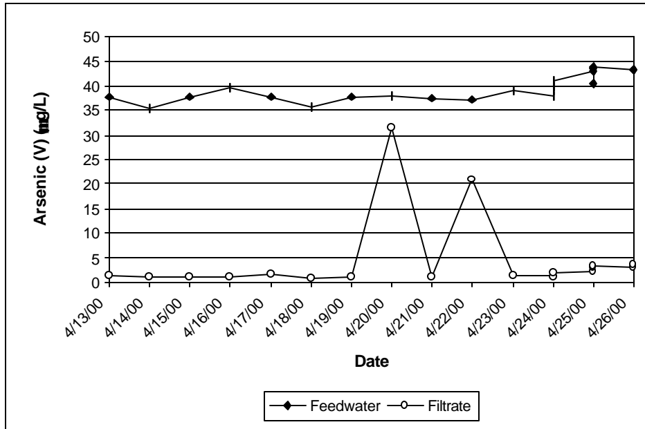
Figure 4-15. Arsenic (V) vs. Time (April 12 – April 26, 2000)
