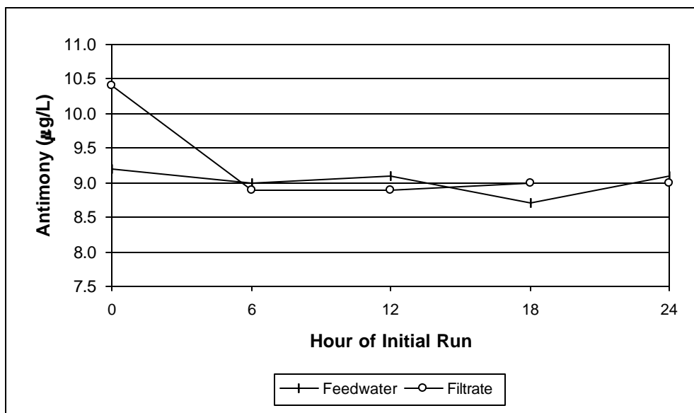
Figure 4-4. Antimony Concentration vs. Time (no coagulant chemicals) (April 11, 2000)
