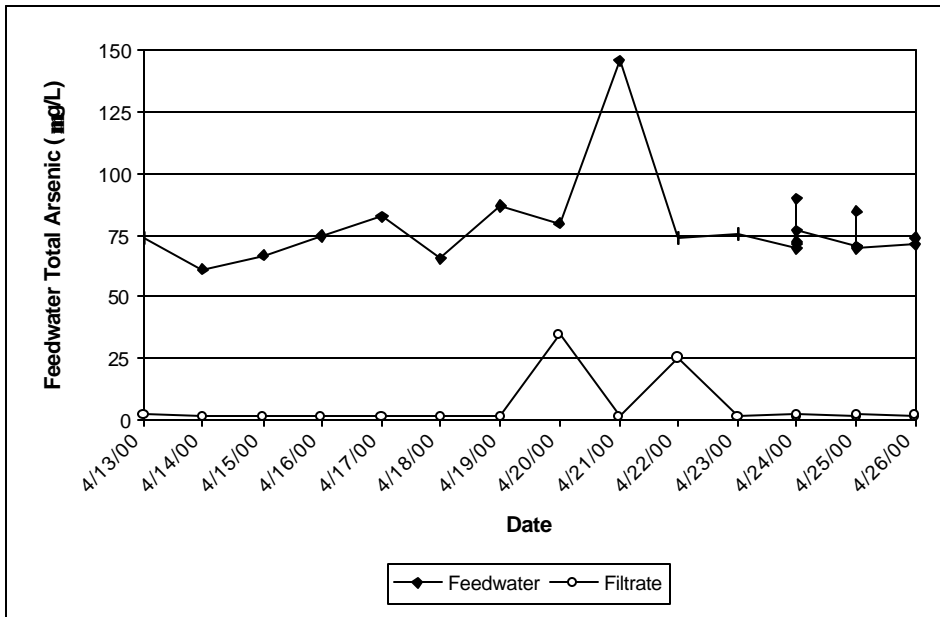
Figure 4-12. Total Arsenic vs. Time (April 12 – April 26, 2000)
