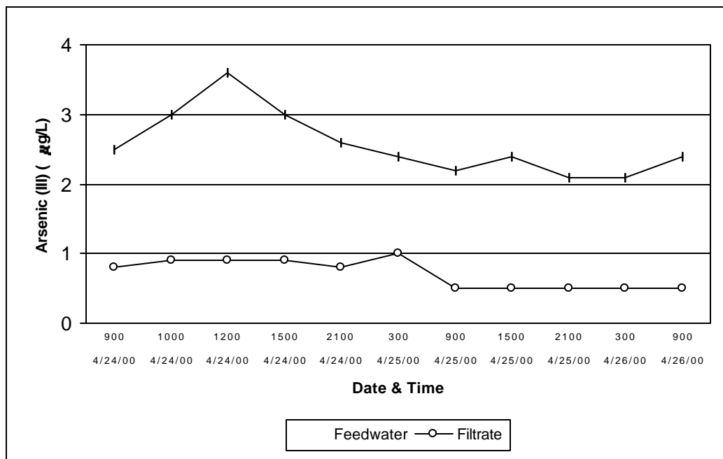
Figure 4-19. Task 4 Arsenic (III) vs. Time (April 24 – April 26, 2000)
