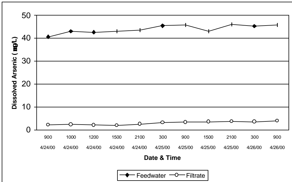
Figure 4-18. Task 4 Dissolved Arsenic vs. Time (April 24 – April 26, 2000)
