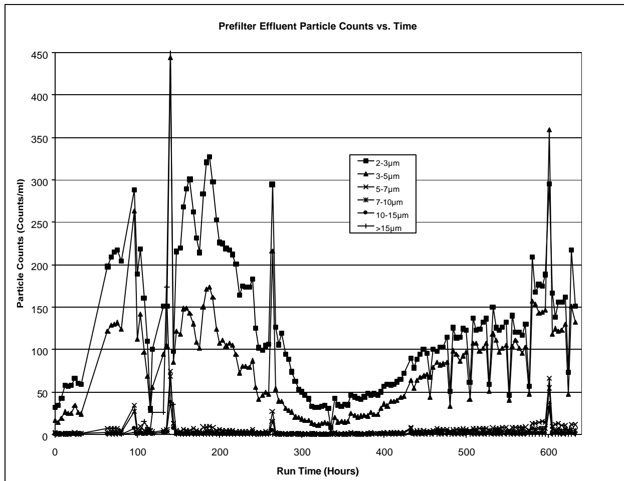
Figure 4-3. Four Hour Prefilter Effluent Particle Counts
