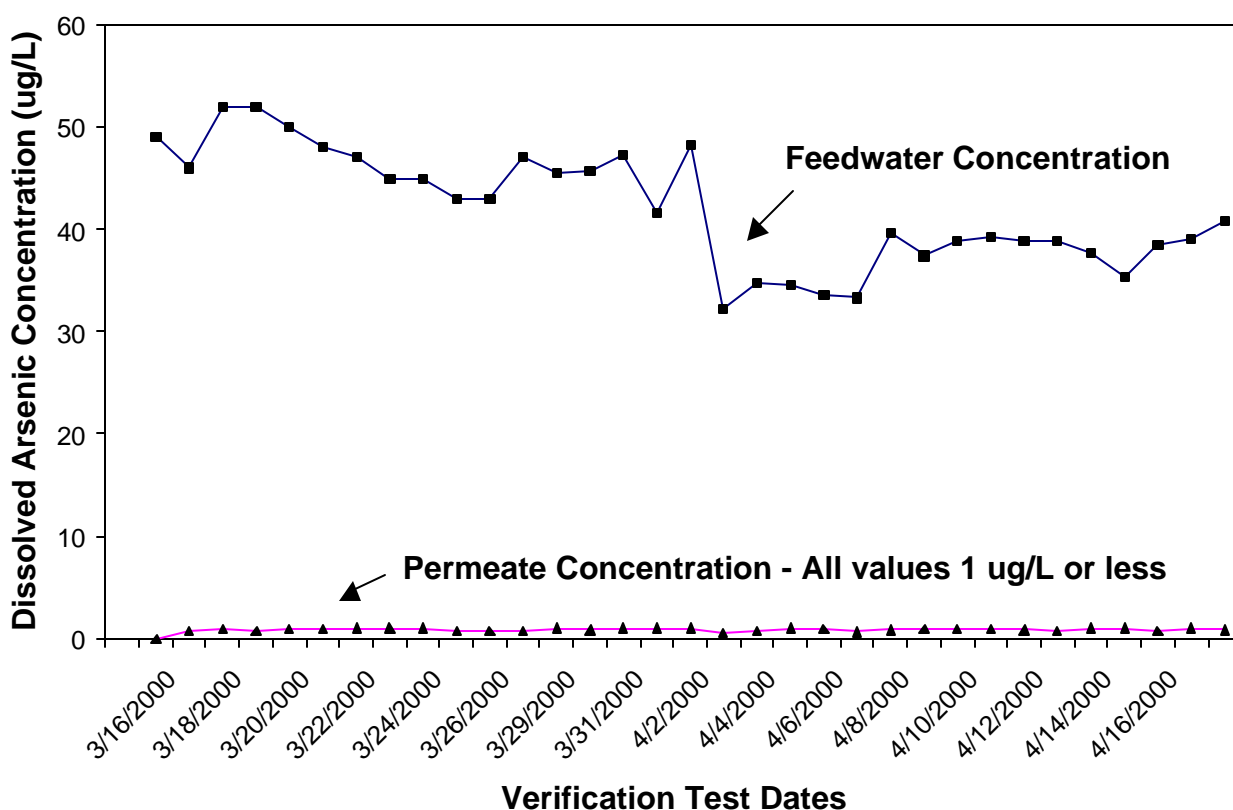
Figure 4-4: Dissolved Arsenic Concentration vs. Time (Data from likely mislabeled containers are not included in this figure)
