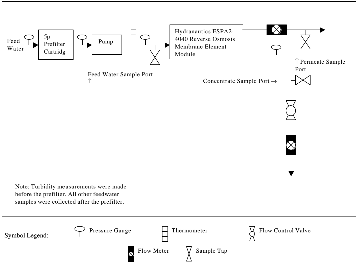
Figure 2-4: Process Flow Diagram
