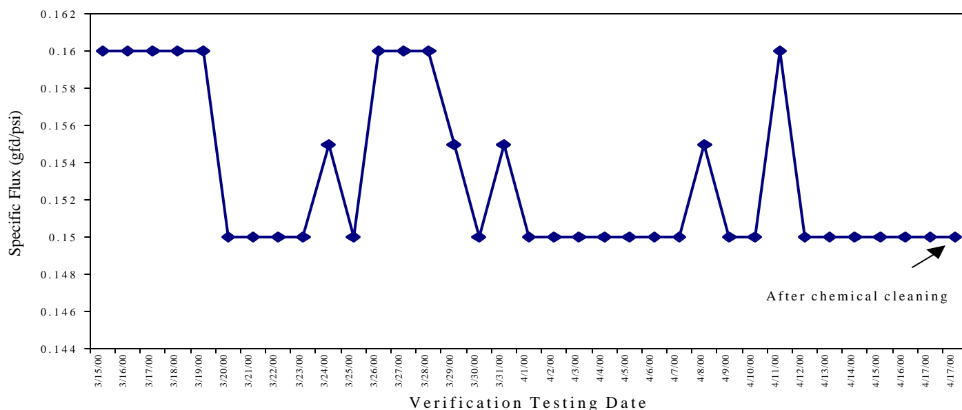
Figure 4-1: Variation of Average Specific Flux Data vs. Time
