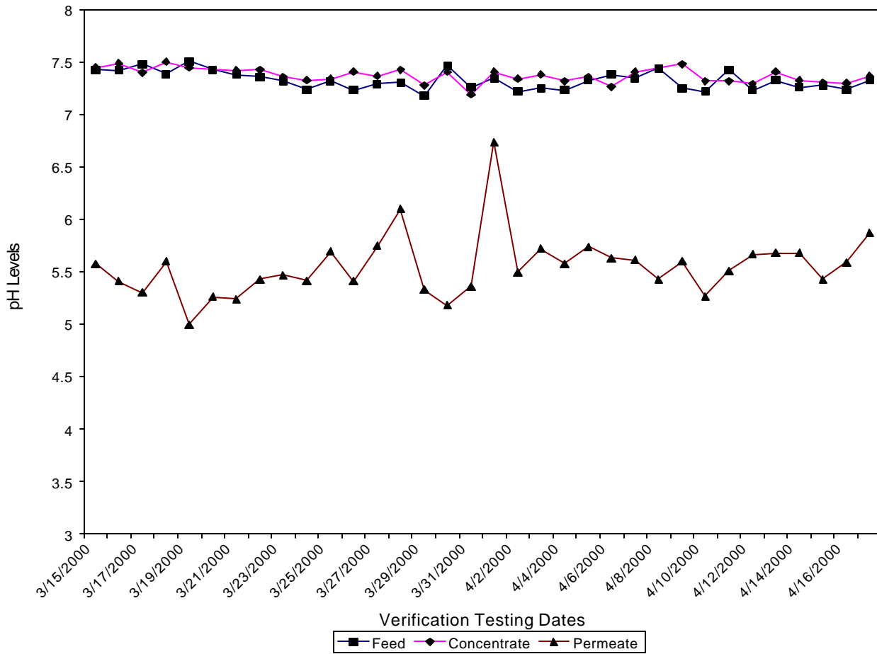
Figure 4-8: pH Concentrations over Testing Period
