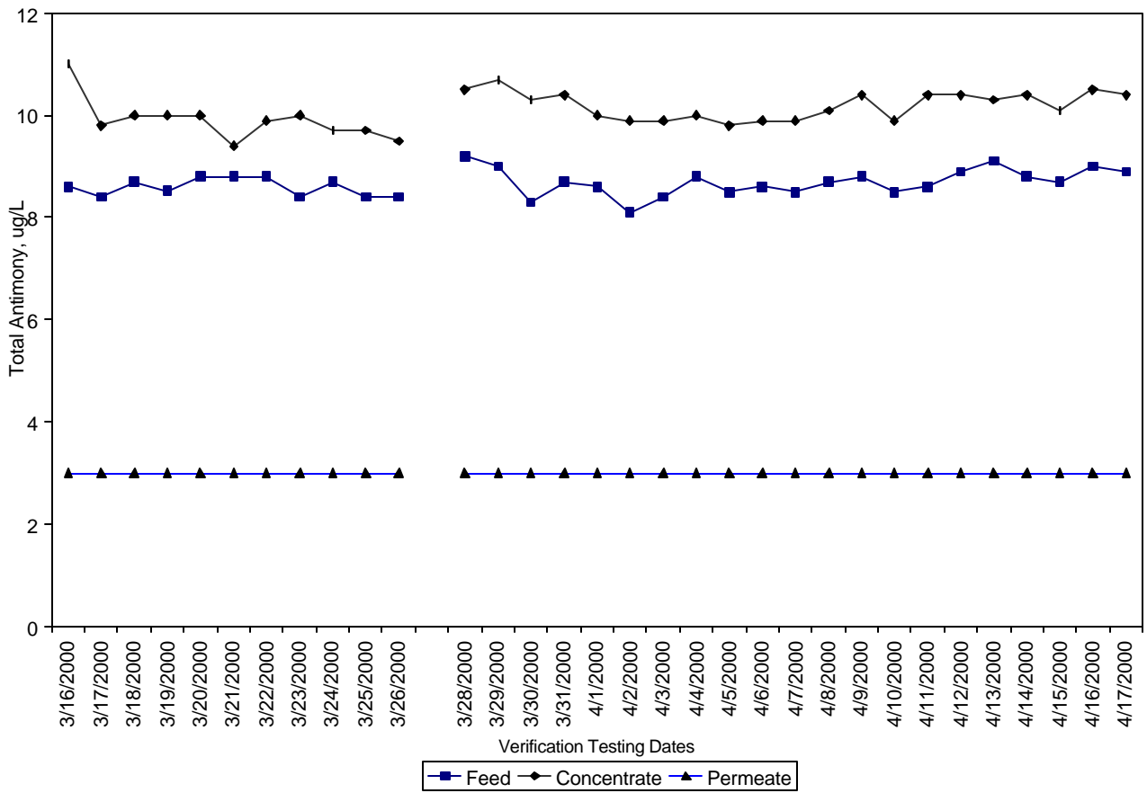
Figure 4-7: Antimony Concentration vs. Time
