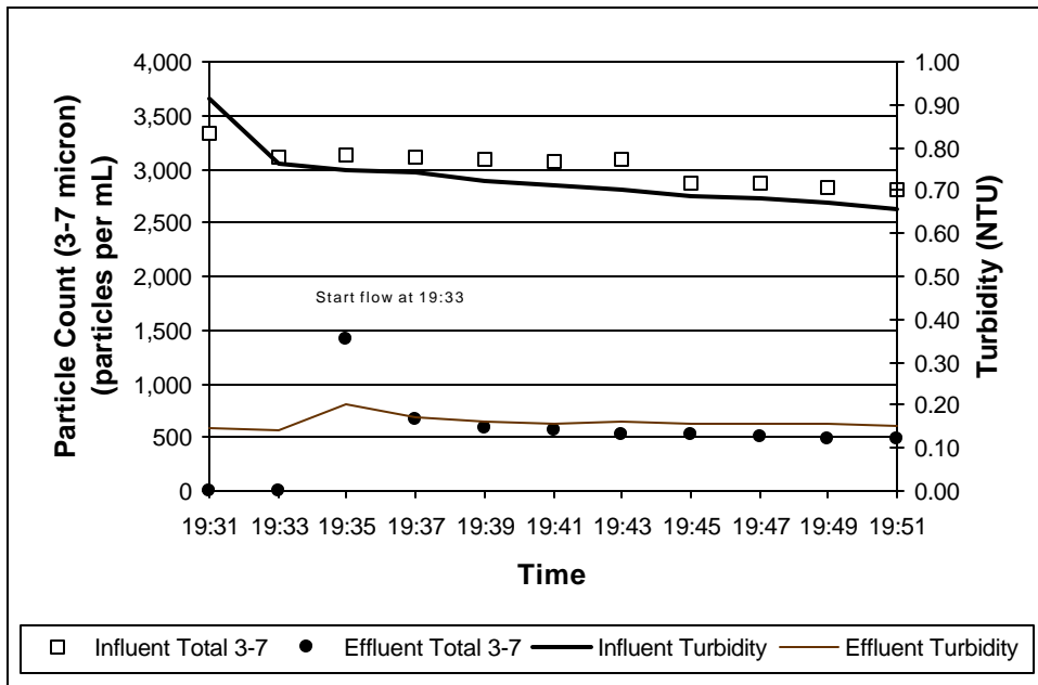
Figure 4-8. Turbidity and 3-7 \mu m Particle Count Stop/Start During Protozoa Challenge #1
