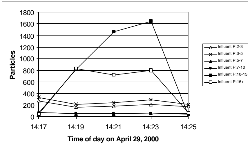
Figure 4-13. Verification of 15 mm Influent Particles
