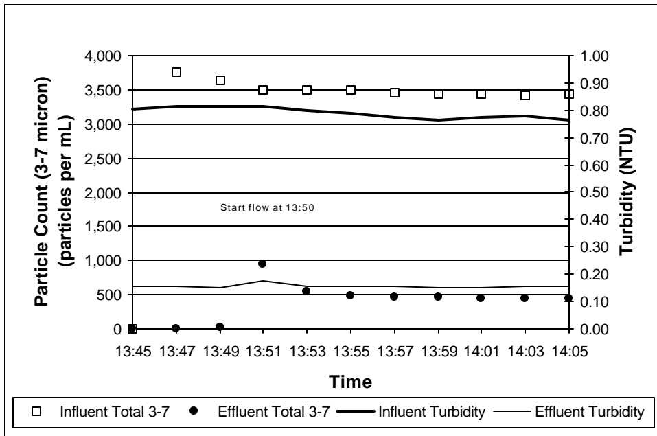
Figure 4-9. Turbidity and 3-7 \mu m Particle Count Stop/Start During Protozoa Challenge #2
