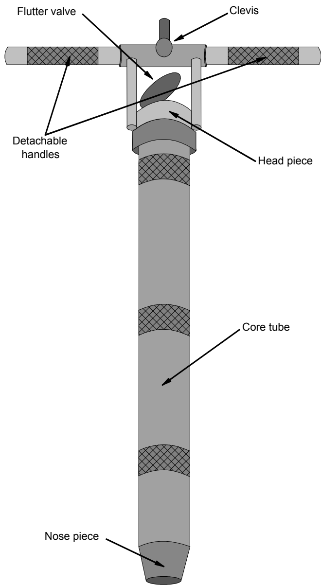
Figure 5-1. Hand Corer.
