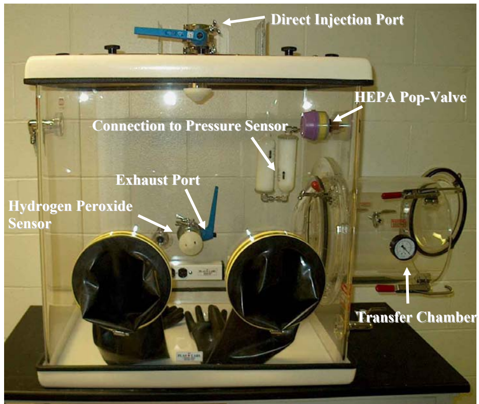
Figure 3-2. Overview of Plas-Labs Compact Glove Box Modifications
