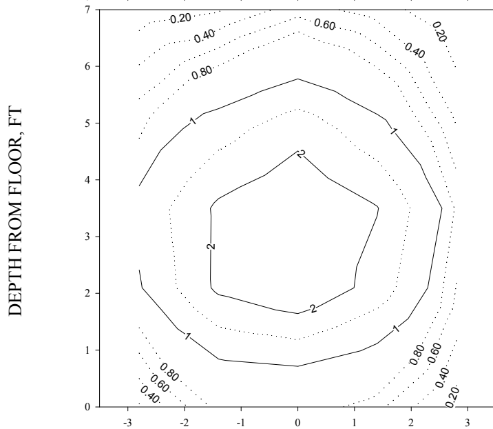
Figure 6-5: Comparison Of Original And Repeat Testing—Non-Dimensional Concentration Distribution For The 10 HP Mixer At 1.25 ft/sec Flume Velocity
