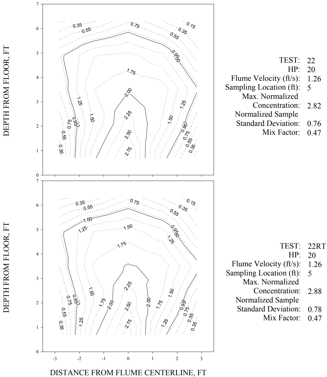
Figure 6-3: Comparison Of Original And Repeat Testing—Non-Dimensional Concentration Distribution For The 20 HP Mixer At 1.25 ft/sec Flume Velocity
