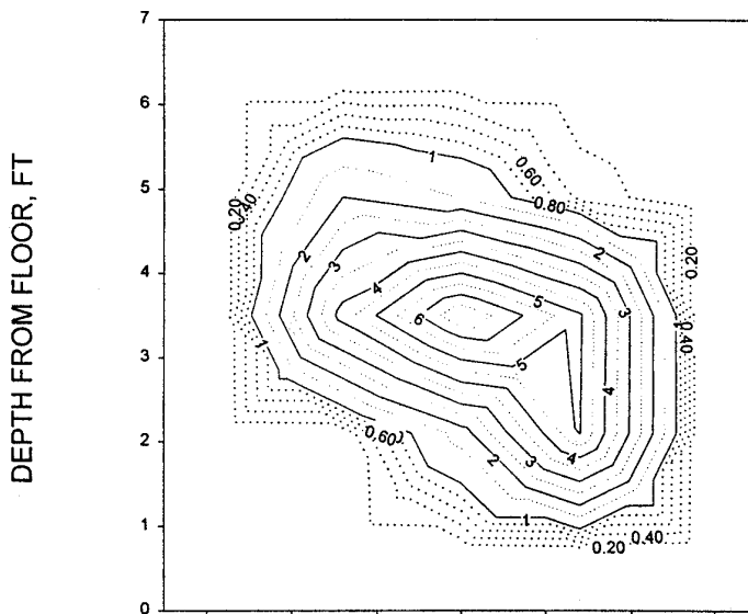
Figure 5-28: Test 11: 10-HP at 10 ft & 3.0 ft/sec
