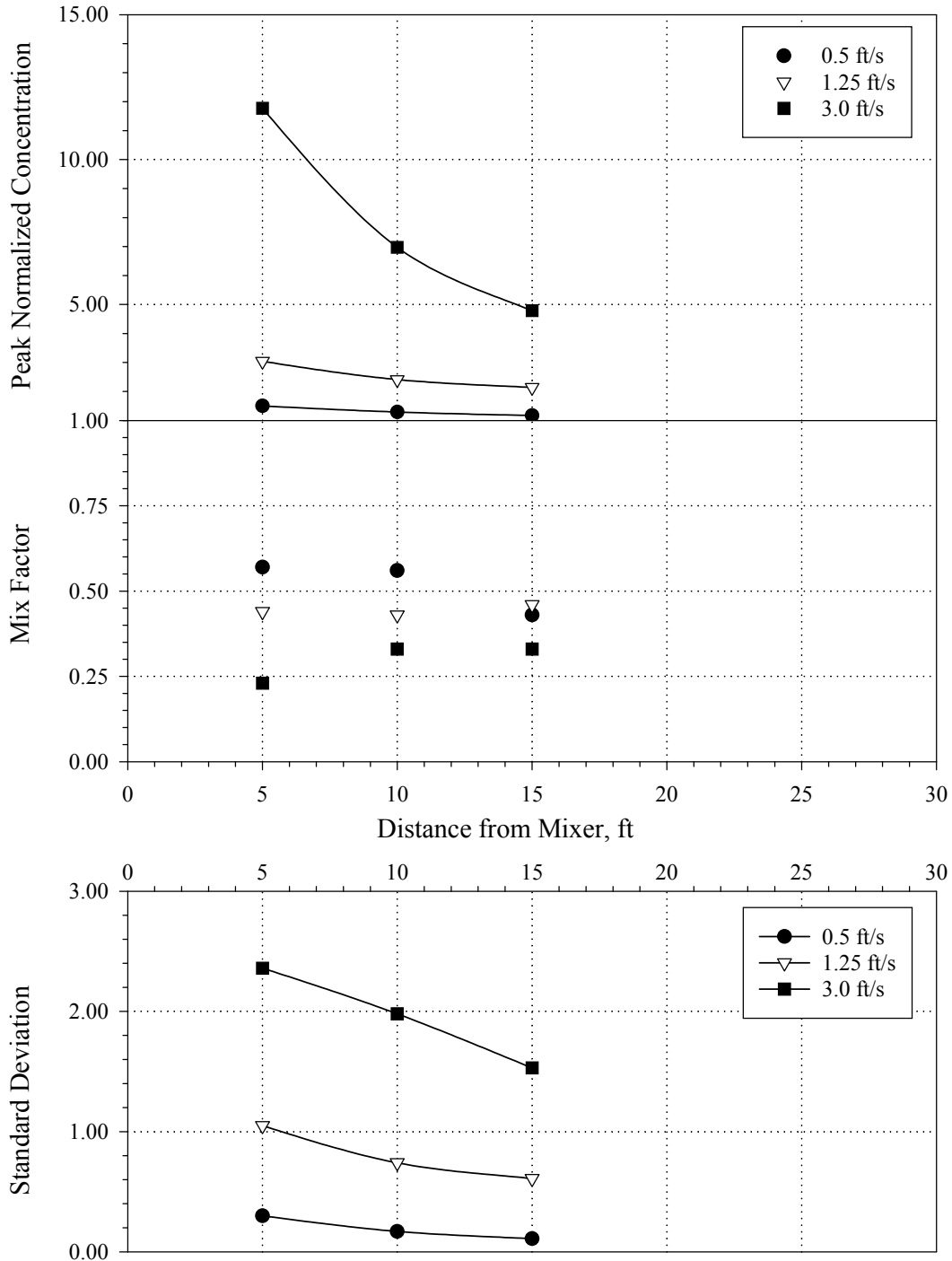
Figure 5-18: Summary Of 10 HP Mixer Performance Data
