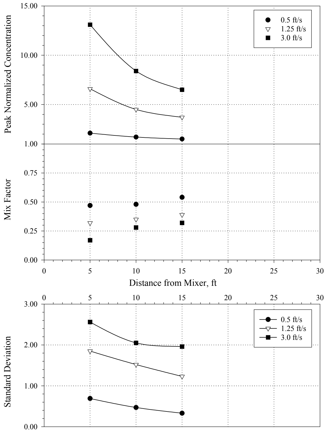
Figure 5-17: Summary Of The 5 HP Mixer Performance Data
