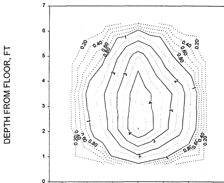
Figure 5-29: Test 26: 20-HP at 10 ft & 3.0 ft/sec
