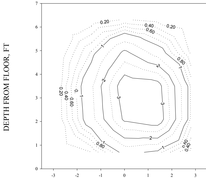
Figure 6-4: Comparison Of Original And Repeat Testing—Non-Dimensional Concentration Distribution For The 5 HP Mixer At 1.25 ft/sec Flume Velocity
