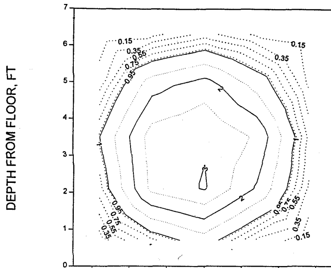
Figure 5-26: Test 13: 10 HP at 5 ft & 1.2 ft/sec
