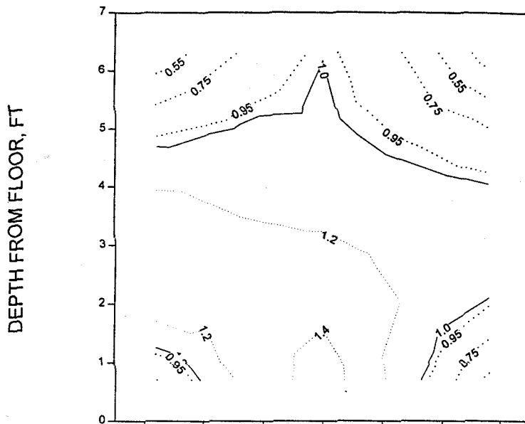
Figure 5-25: Test 16: 10 HP at 5 ft & 0.5 ft/sec
