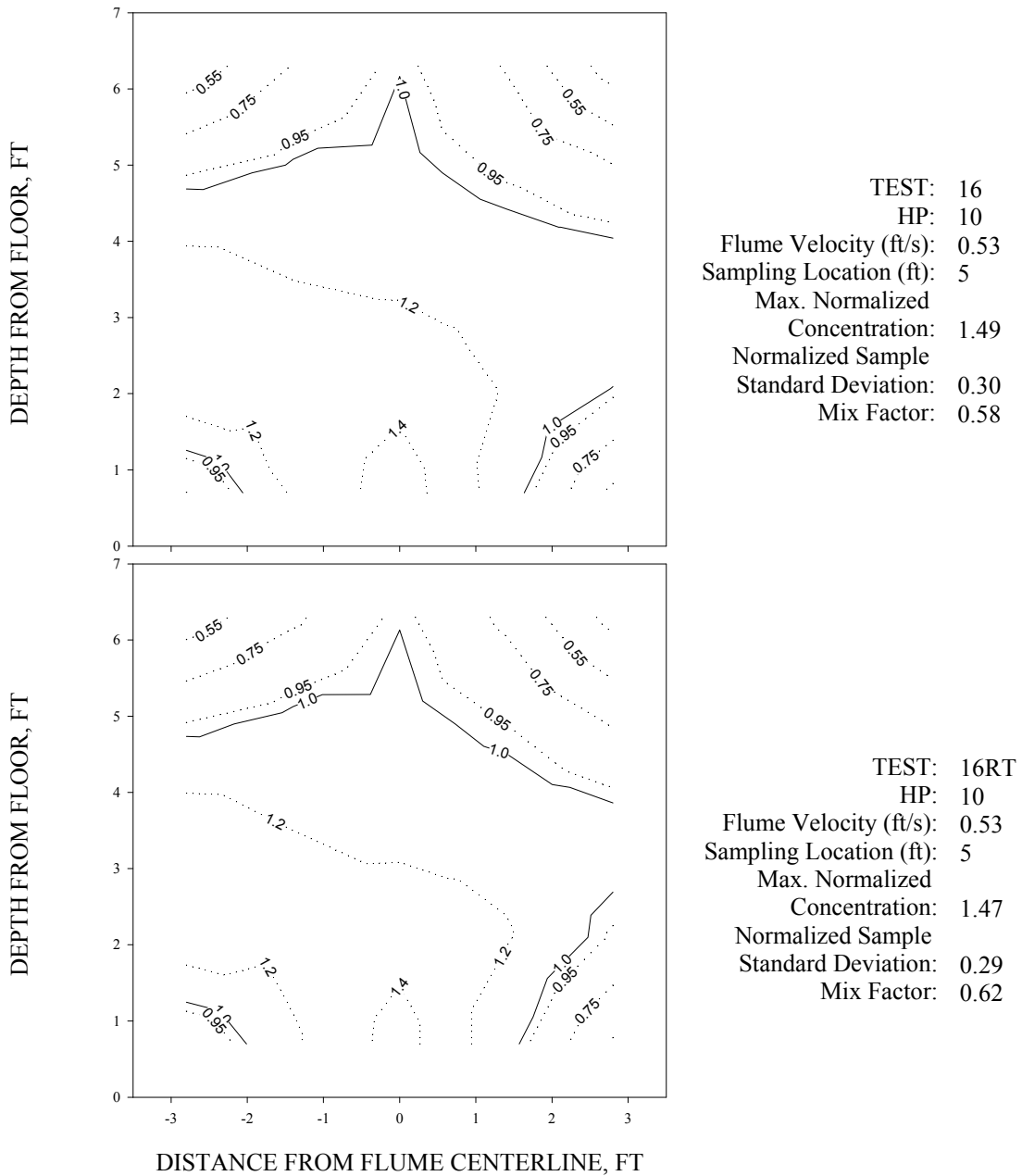
Figure 6-2: Comparison Of Original And Repeat Testing—Non-Dimensional Concentration Distribution For The 10 HP Mixer At 0.5 ft/sec Flume Velocity
