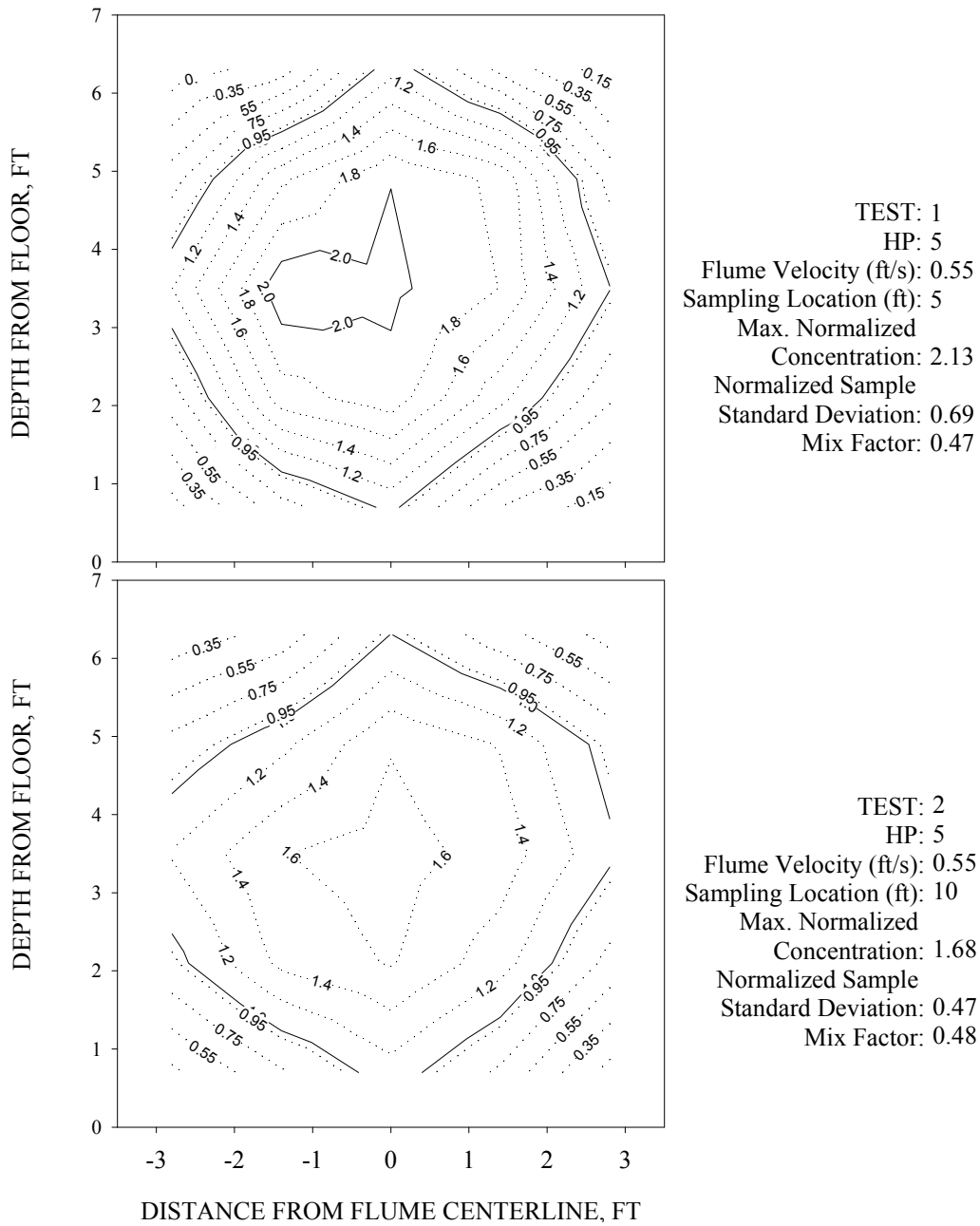
Figure 5-14: Example Of Similar Mix Factors With Differing Maximum (Peak) Concentrations
