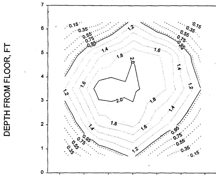
Figure 5-24: Test 1: 5 HP at 5 ft & 0.5 ft/sec
