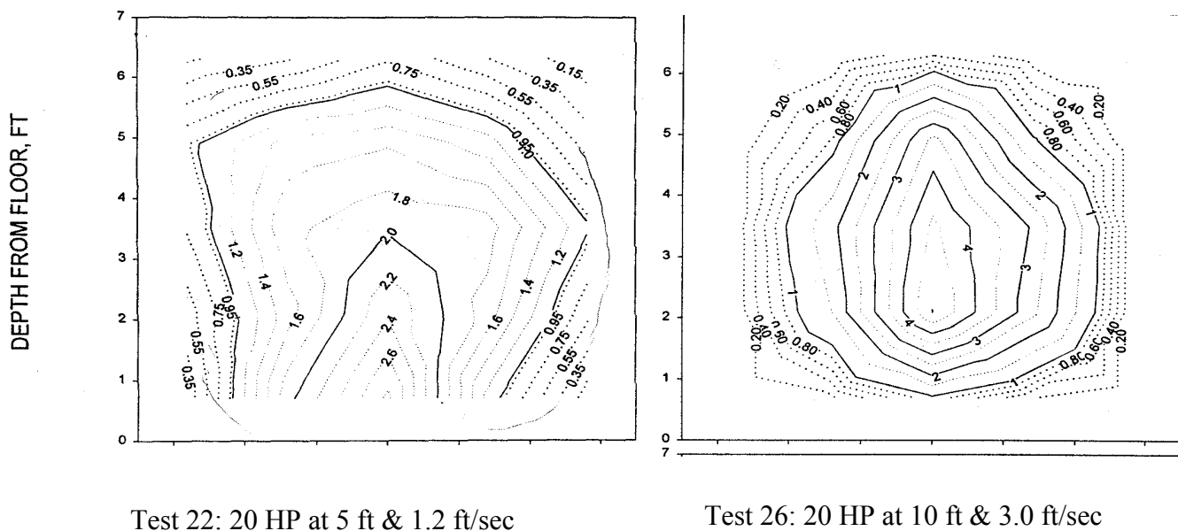
Figure 5-23: Comparison of Uniformity of Mix at Different Flume Velocities
