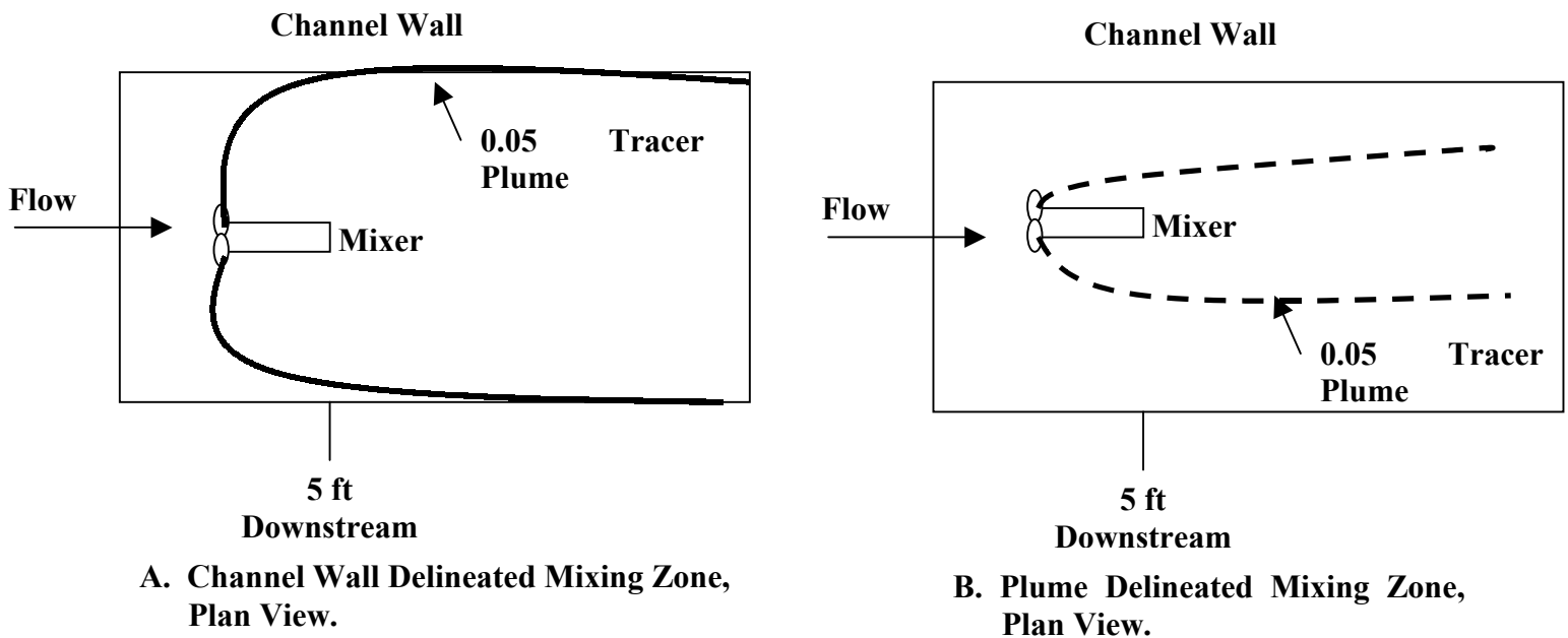
Figure 5-22 : Mixing Zone Patterns
