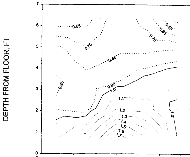
Figure 5-27: Test 19R: 20-HP at 5 ft & 1.2ft/sec
