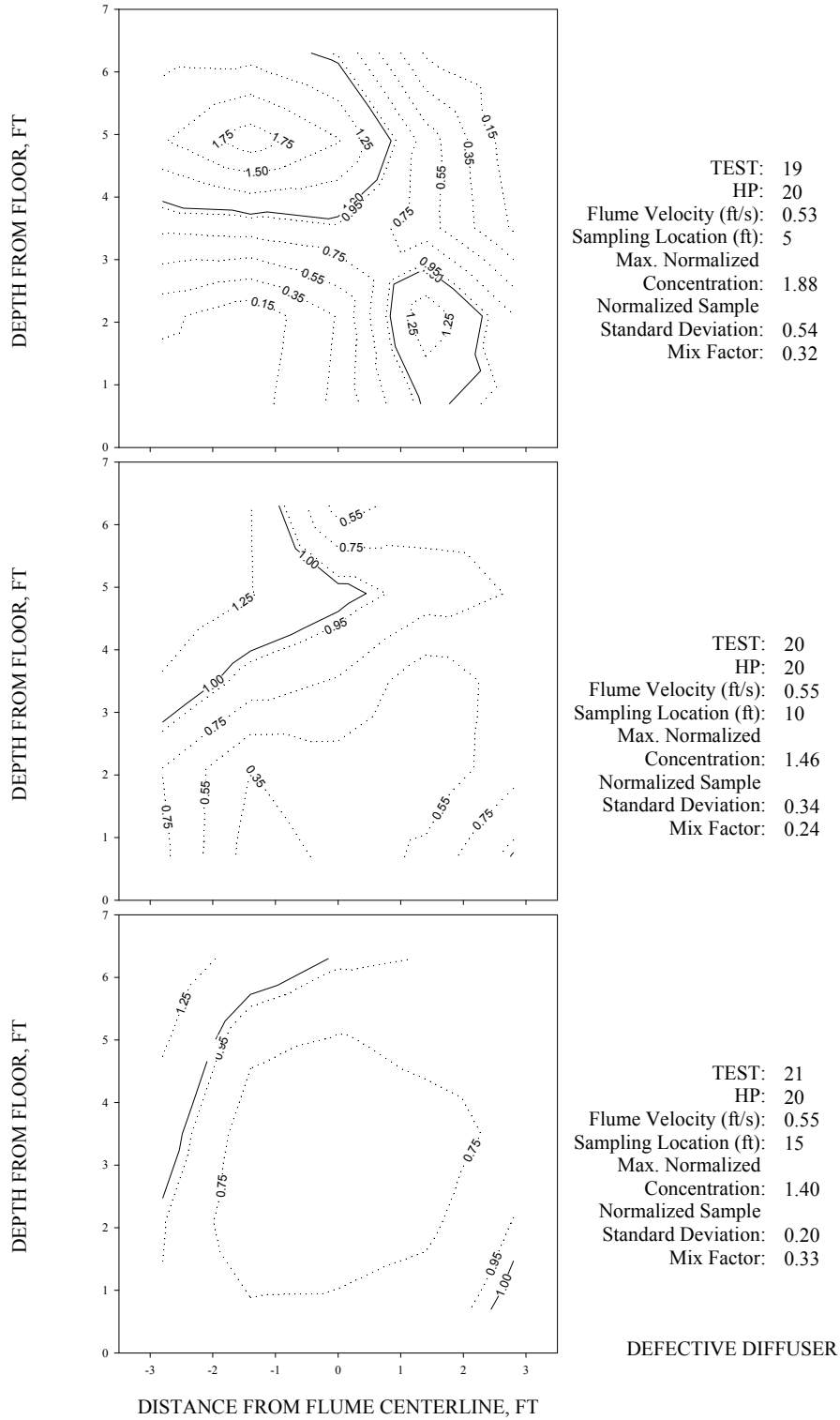
Figure 5-10a: Non-Dimensional Concentration Distribution For The 20 HP Mixer At 0.5 ft/sec Flume Velocity—Rejected Due To Defective Diffuser
