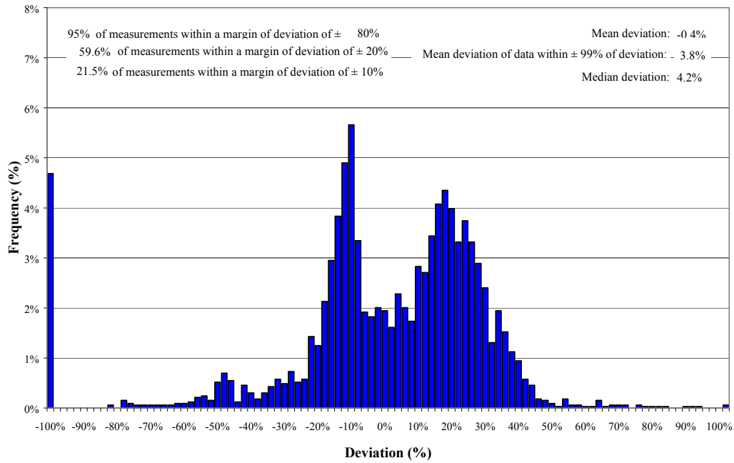
Figure 4-23. Flow deviation distribution—Tests B, C and D.
