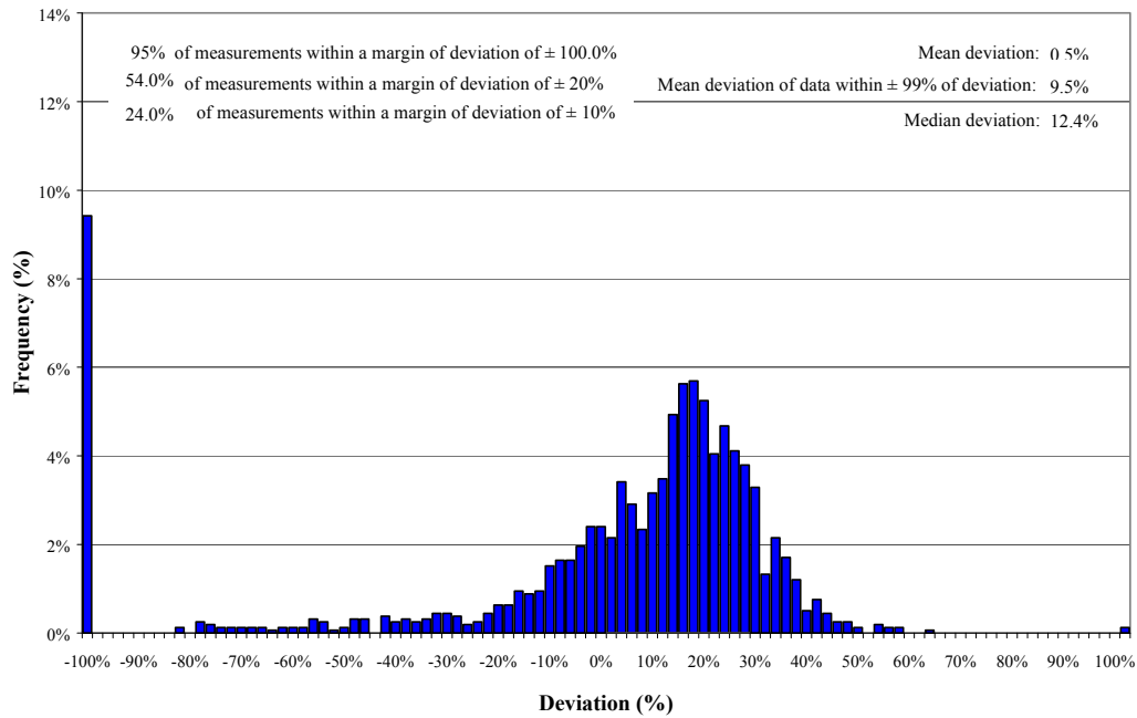
Figure 4-24. Flow deviation distribution—simulated dry weather conditions.
