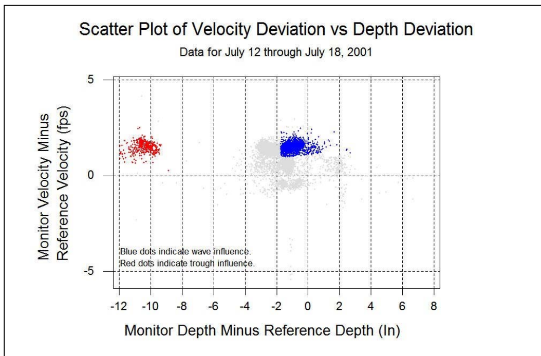
Figure 4-6. Scatter-plot showing possible standing wave and trough influence.
