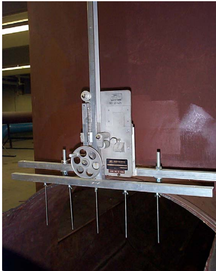
Figure 3-7. Reference depth point gauge.
