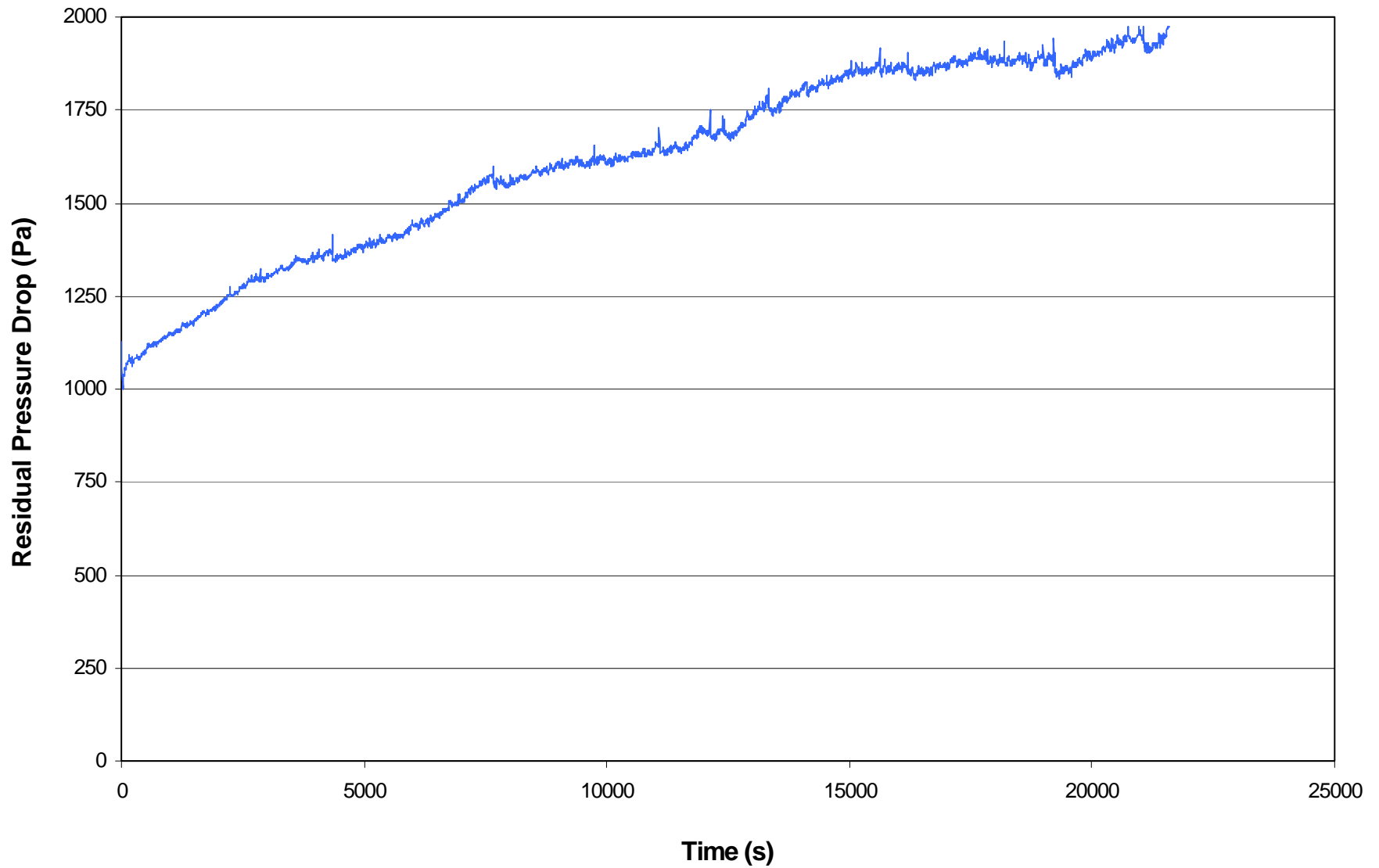
Figure C-8. Residual pressure drop across filter fabric during performance test run V006-5.
