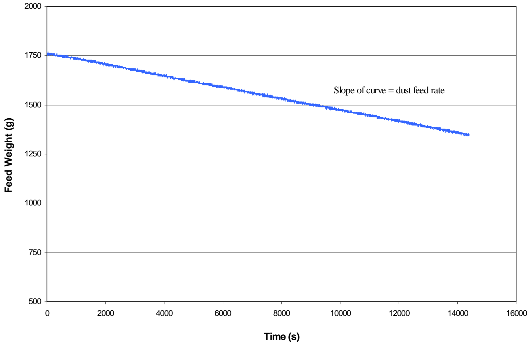
Figure C-1. Change in Pural NF dust scale reading with time during performance test run V006-1.
