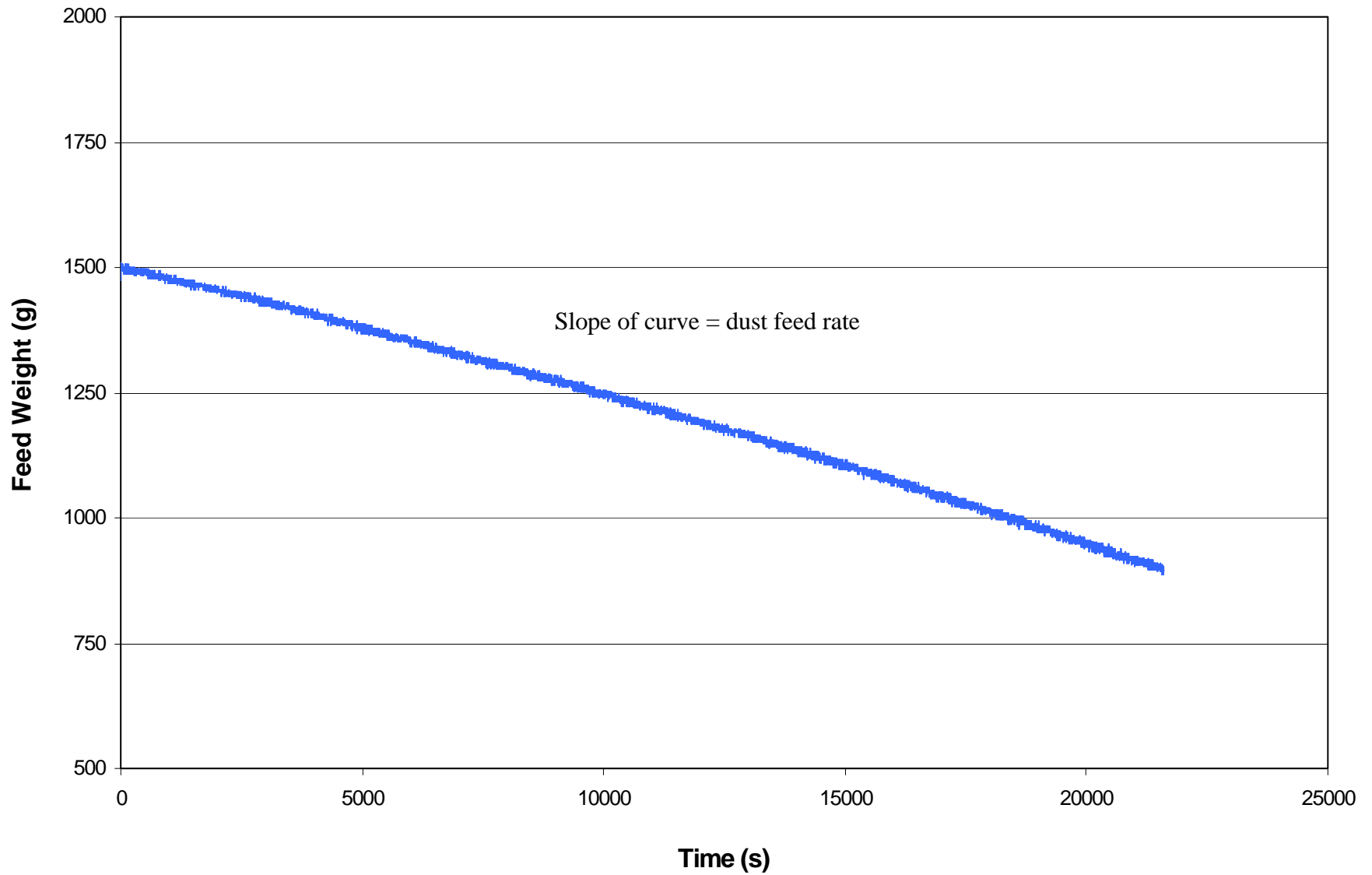
Figure C-3. Change in Pural NF dust scale reading with time during performance test run V006-3.
