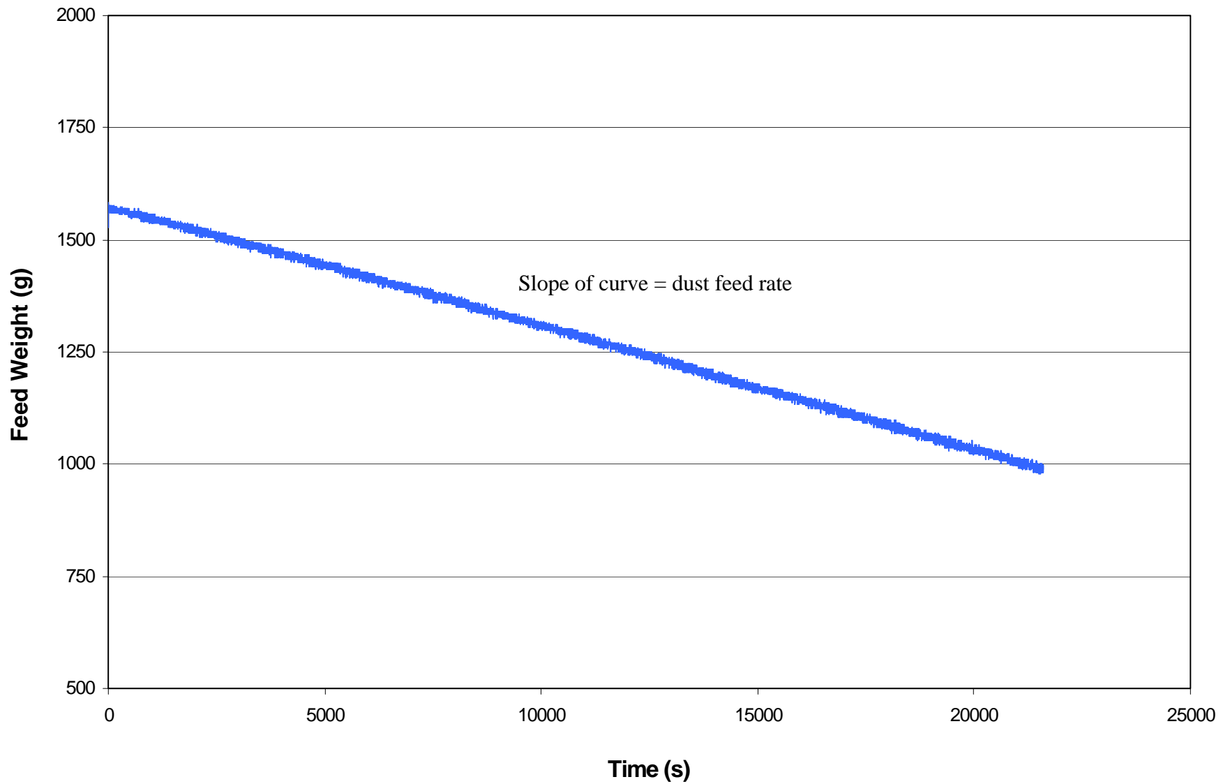
Figure C-7. Change in Pural NF dust scale reading with time during performance test run V006-5.
