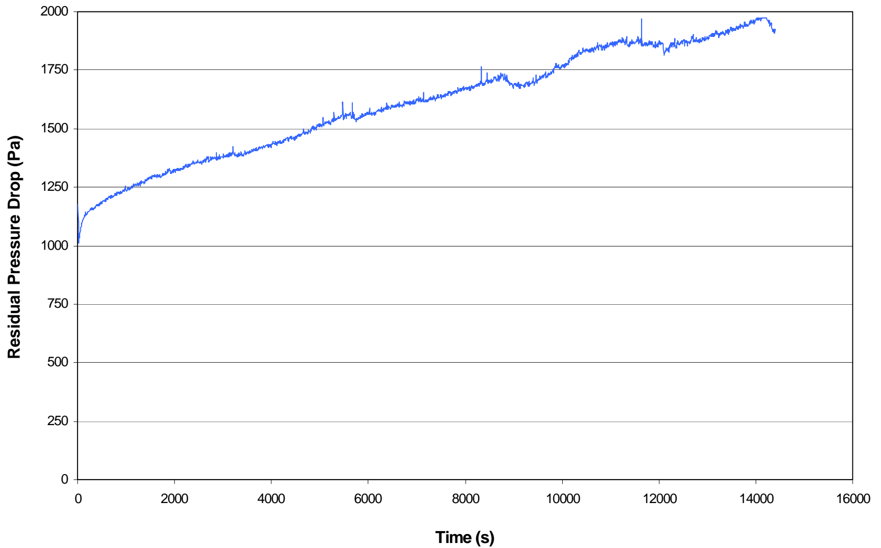
Figure C-2. Residual pressure drop across filter fabric during performance test run V006-1.
