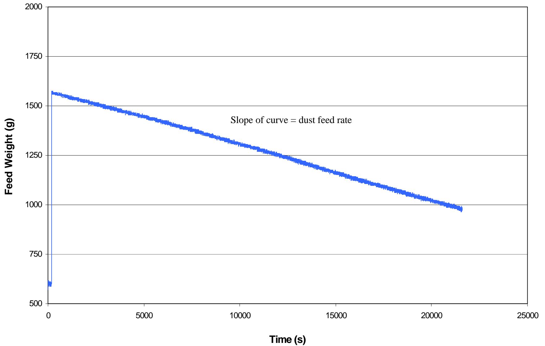
Figure C-5. Change in Pural NF dust scale reading with time during performance test run V006-4.
