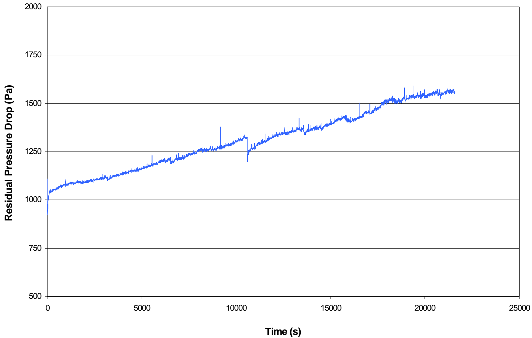
Figure C-4. Residual pressure drop across filter fabric during performance test run V006-3.
