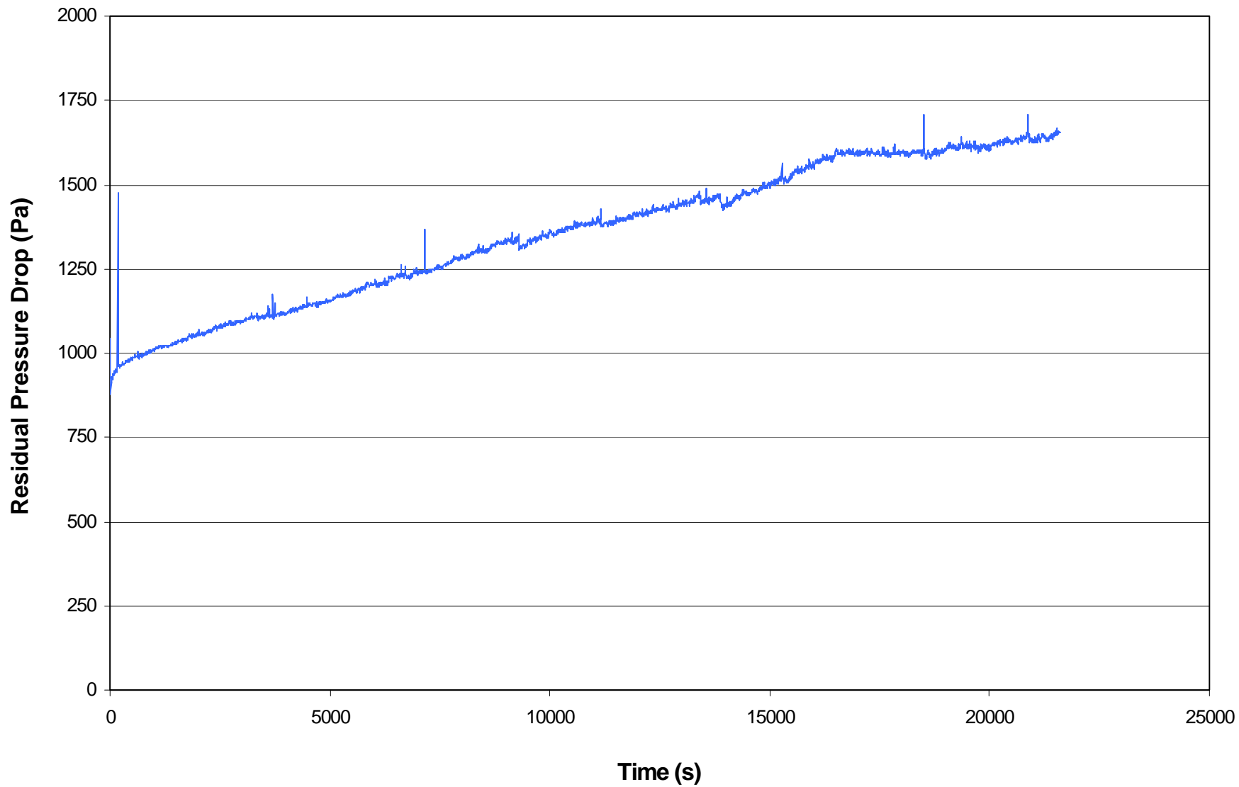
Figure C-6. Residual pressure drop across filter fabric during performance test run V006-4.
