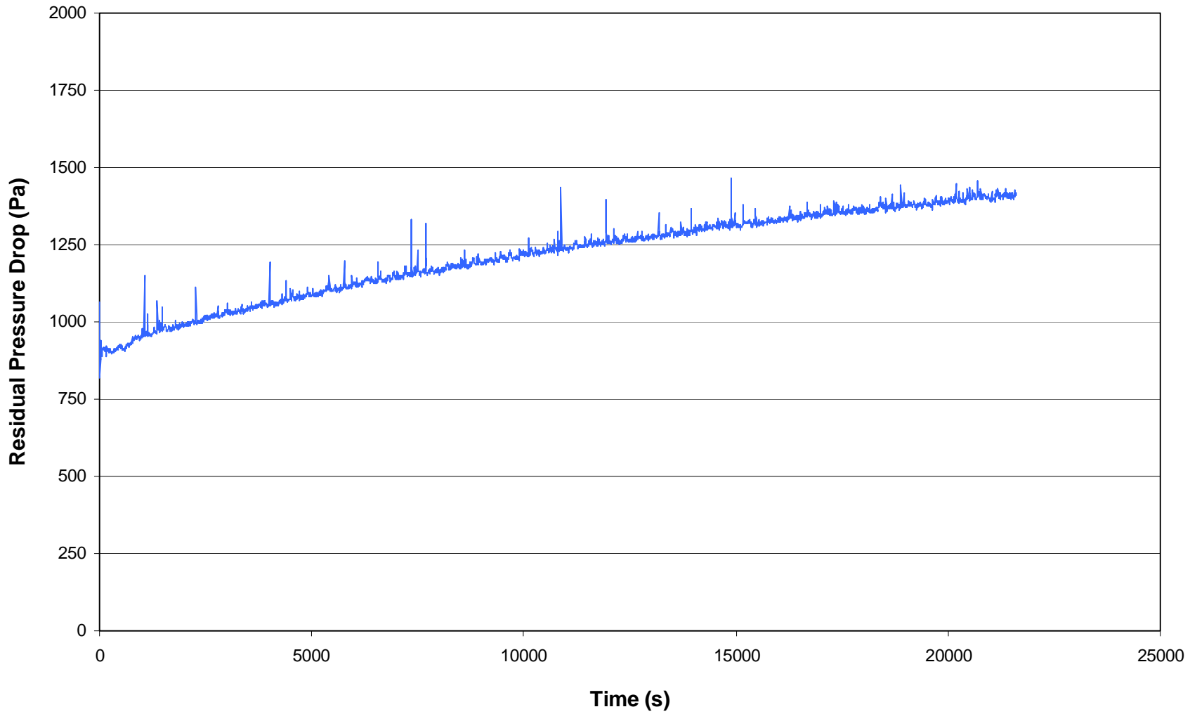
Figure C-4. Residual pressure drop across filter fabric during performance test run V005-2.
