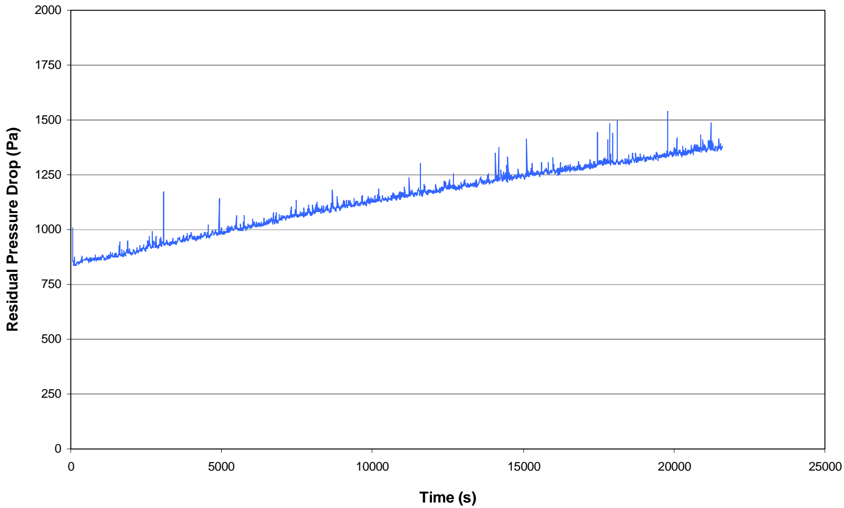
Figure C-6. Residual pressure drop across filter fabric during performance test run V005-3.
