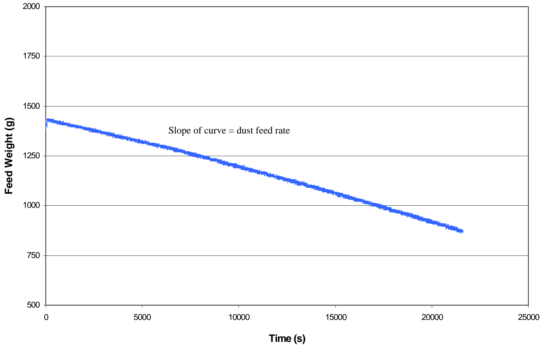
Figure C-5. Change in Pural NF dust scale reading with time during performance test run V005-3.
