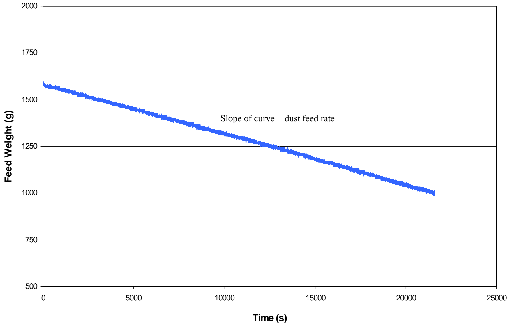
Figure C-3. Change in Pural NF dust scale reading with time during performance test run V005-2.
