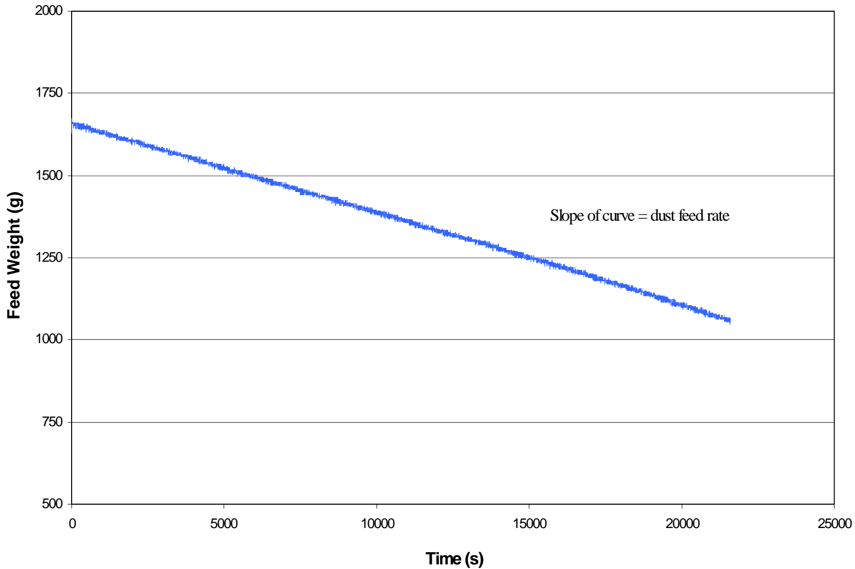
Figure C-1. Change in Pural NF dust scale reading with time during performance test run V005-1.
