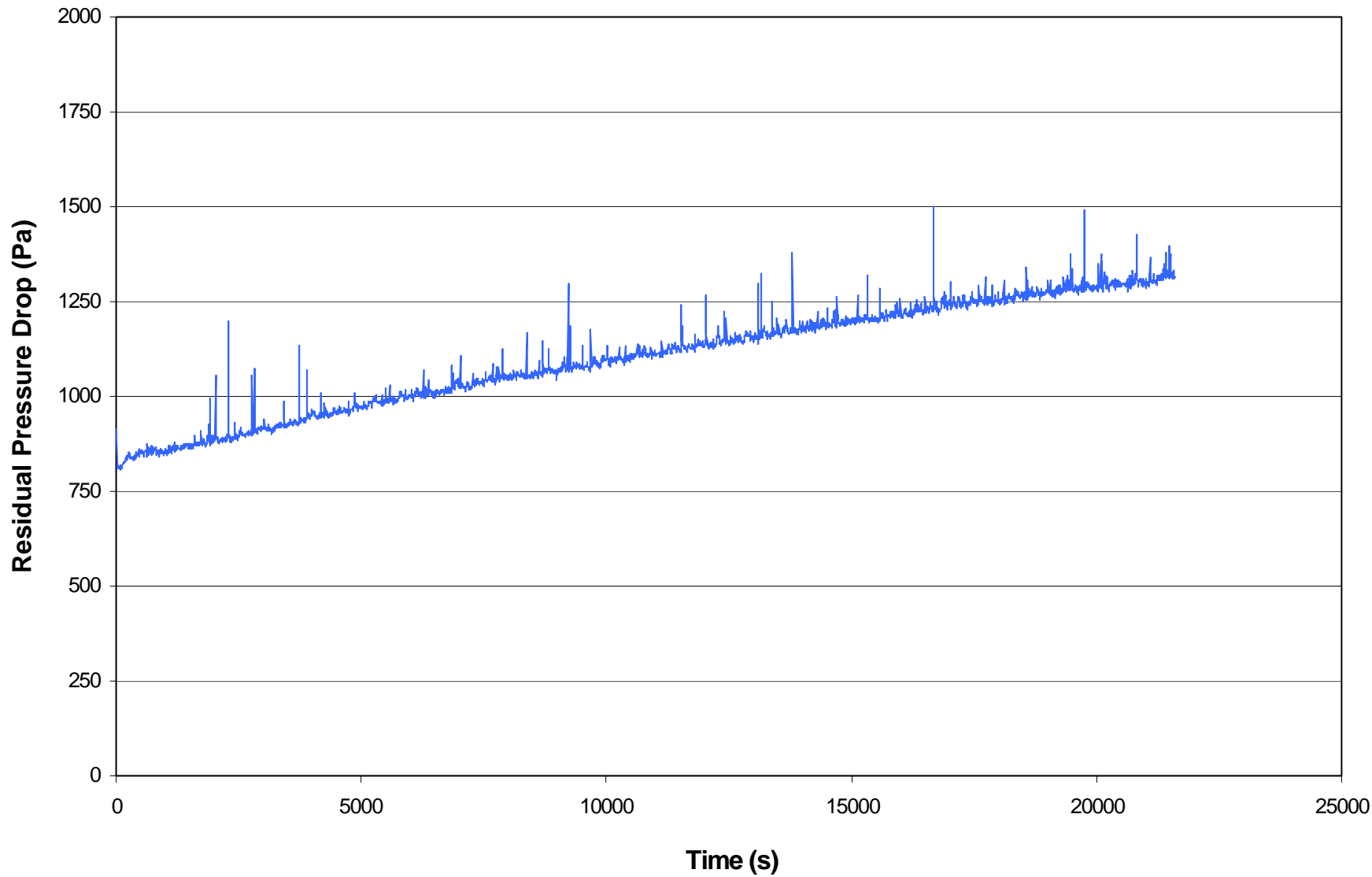
Figure C-2. Residual pressure drop across filter fabric during performance test run V005-1.
