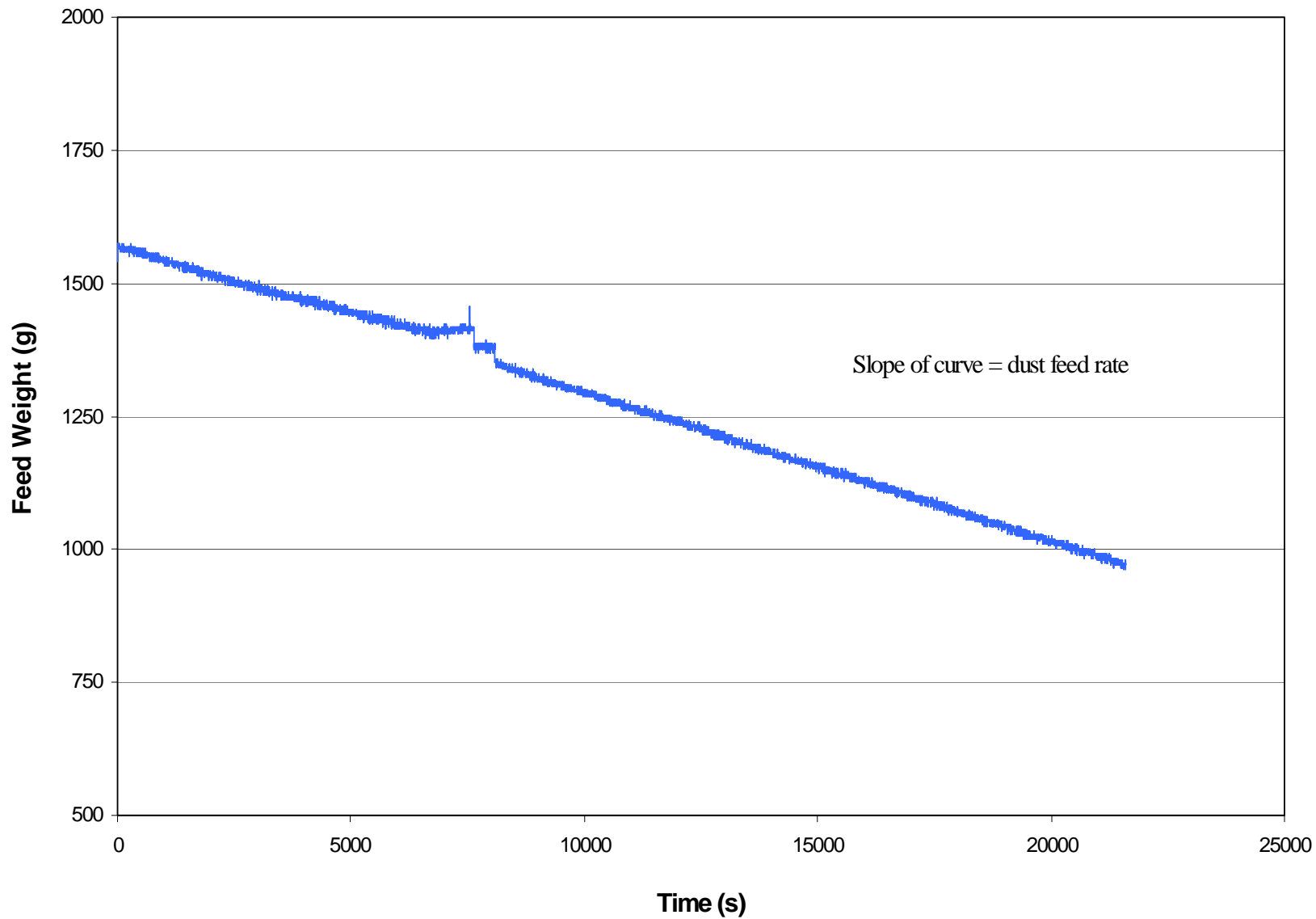
Figure C-5. Change in Pural NF dust scale reading with time during performance test run V003-3.
