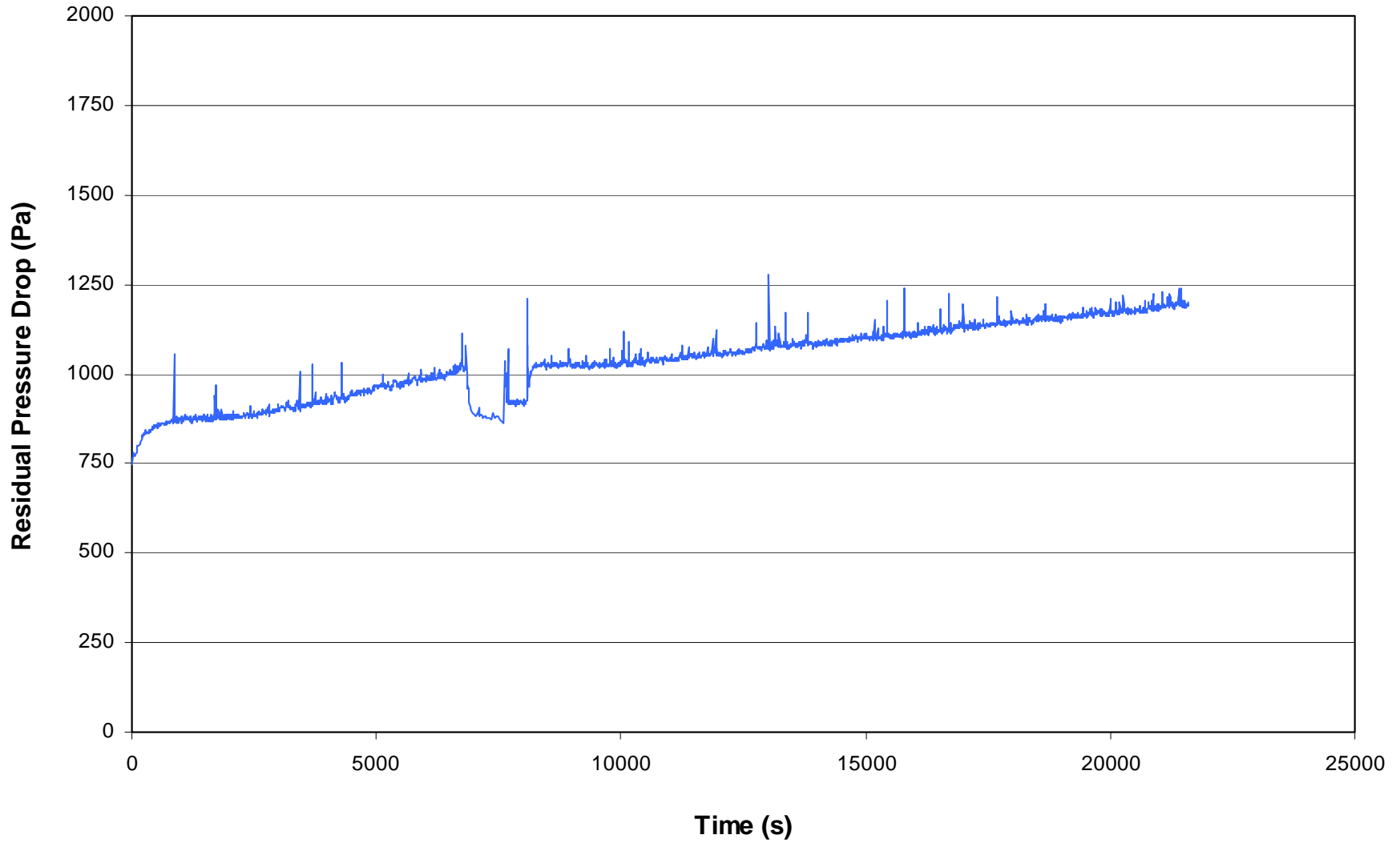
Figure C-6. Residual pressure drop across filter fabric during performance test run V003-3.
