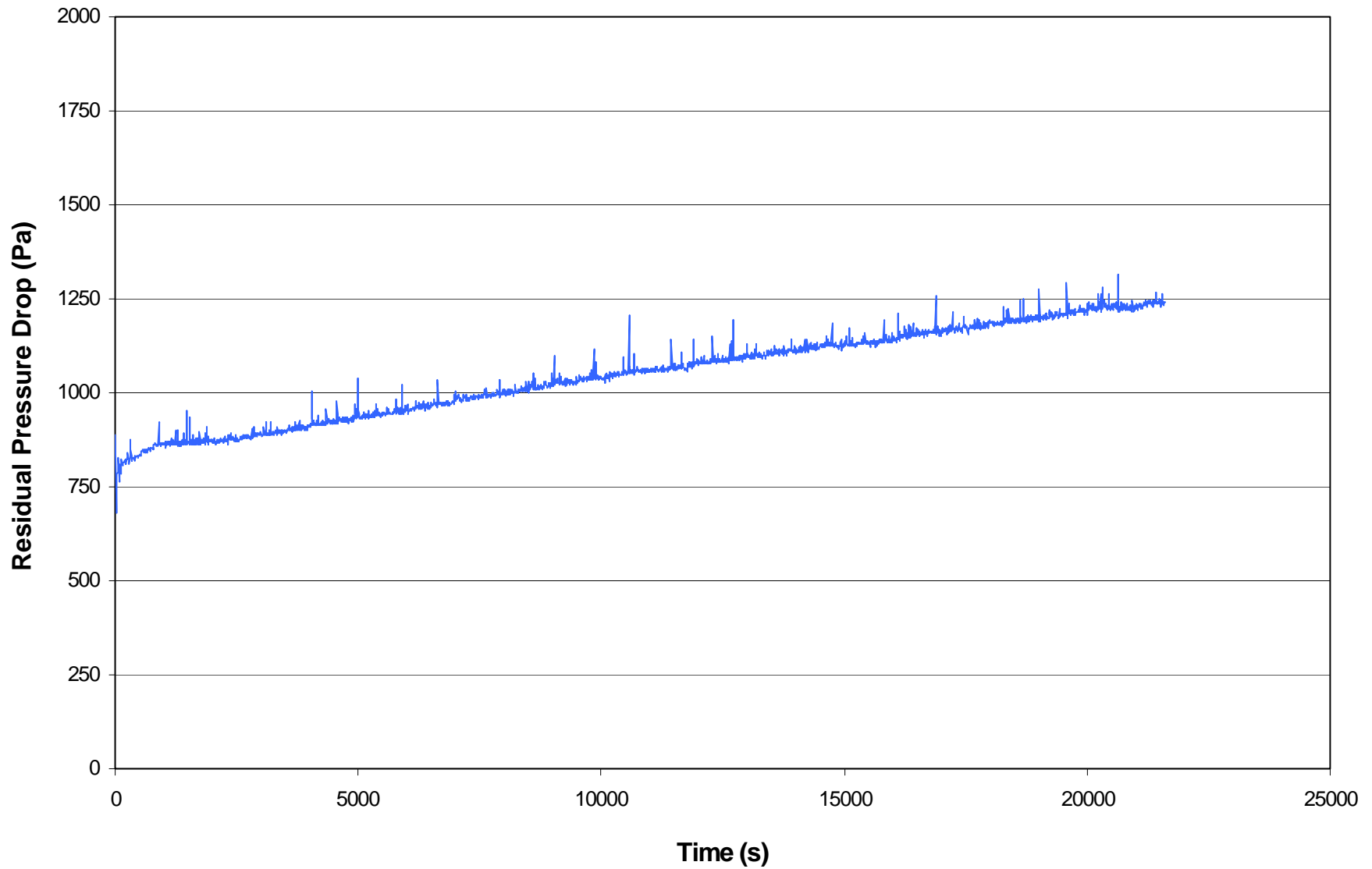
Figure C-2. Residual pressure drop across filter fabric during performance test run V003-1.
