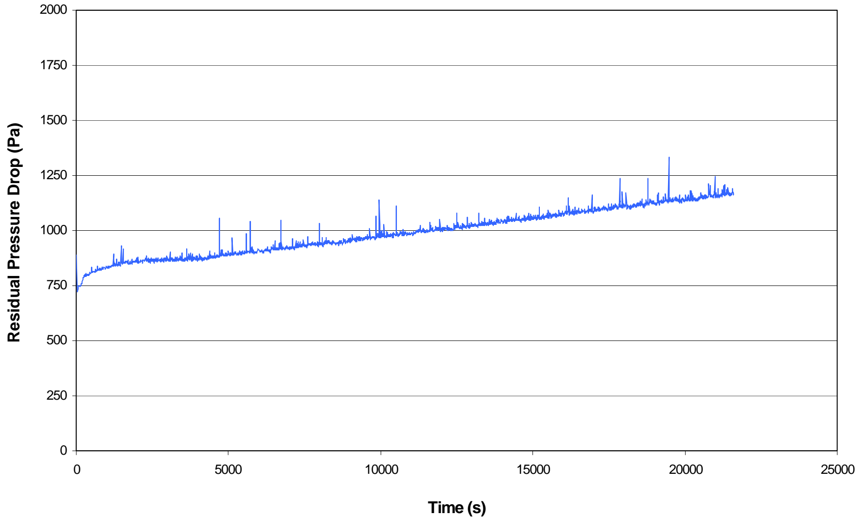
Figure C-4. Residual pressure drop across filter fabric during performance test run V003-2.
