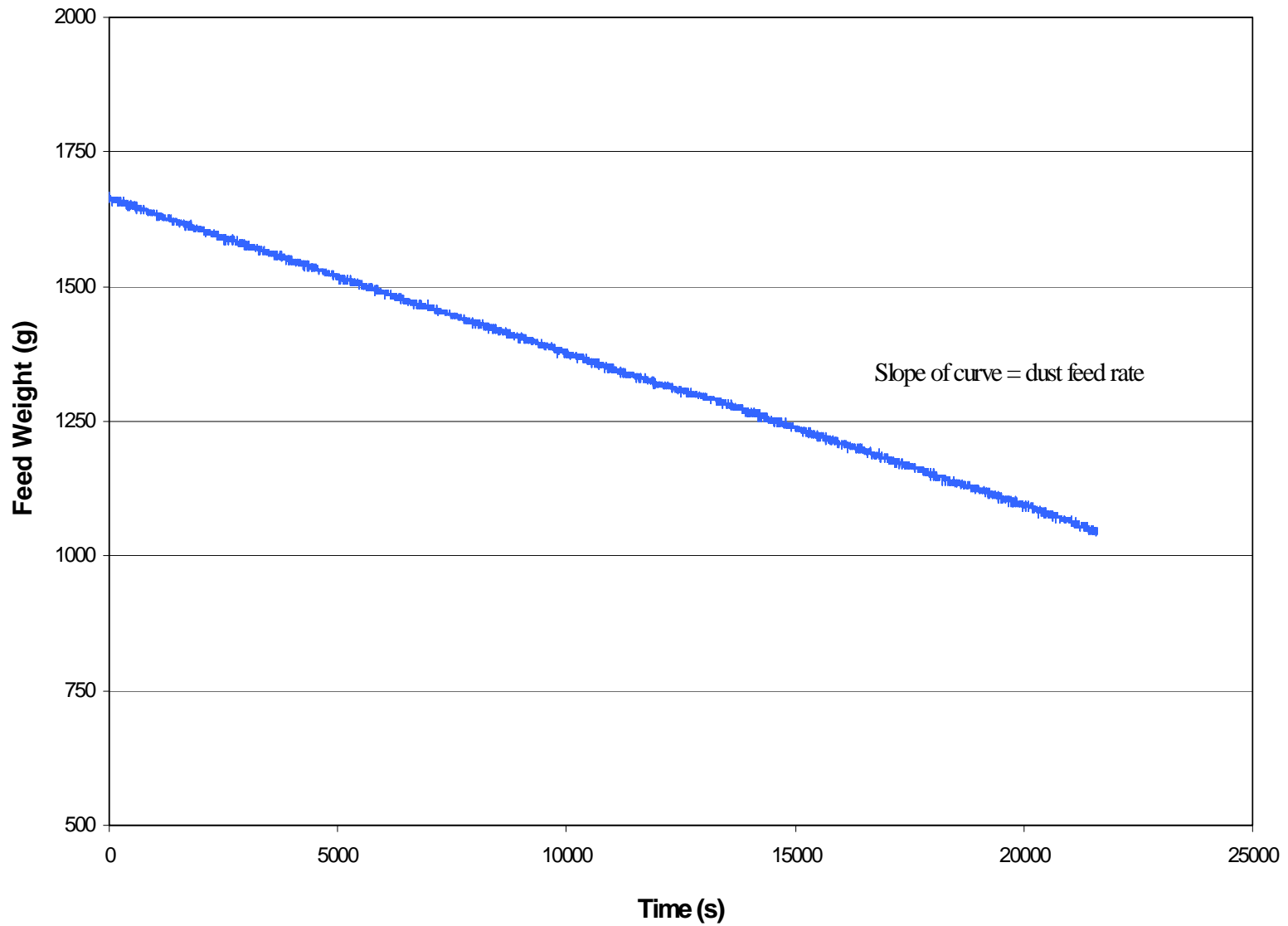
Figure C-1. Change in Pural NF dust scale reading with time during performance test run V003-1.
