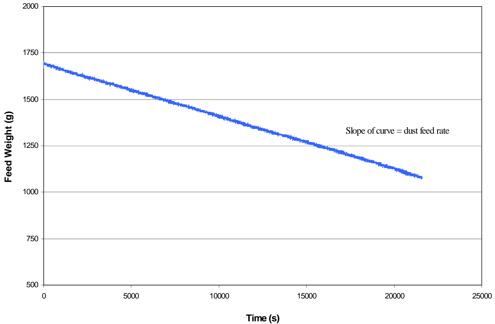
Figure C-3. Change in Pural NF dust scale reading with time during performance test run V003-2.
