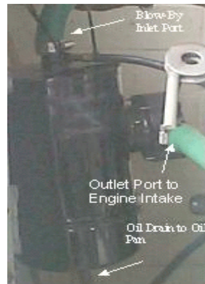
Figure 1. Spiracle™ blow-by filter unit.
