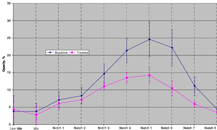
Steady-State Opacity
