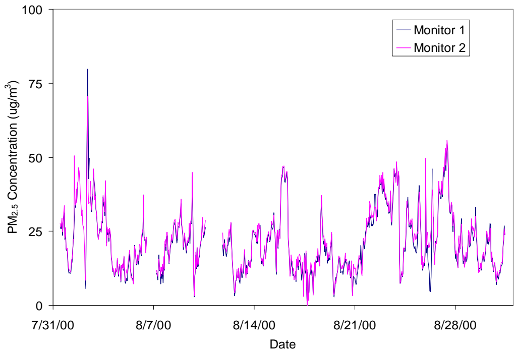
Figure 6-1a. Hourly PM 2.5 Mass Concentrations from the Two Series 1400a SES TEOM Monitors Recorded During Phase I of Verification Testing
