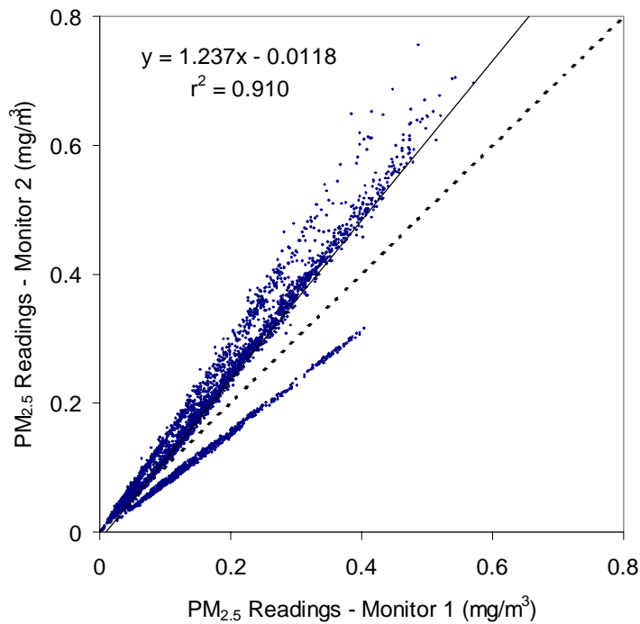
Figure 6-4b. Correlation Plot of 10-Minute PM 2.5 Measurements from Duplicate ELPI™ Monitors During Phase II of Verification Testing
