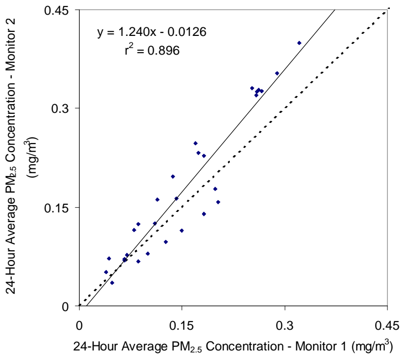
Figure 6-5b. Correlation Plot of 24-Hour Average PM 2.5 Concentrations from Duplicate ELPI TM Monitors During Phase II of Verification Testing
