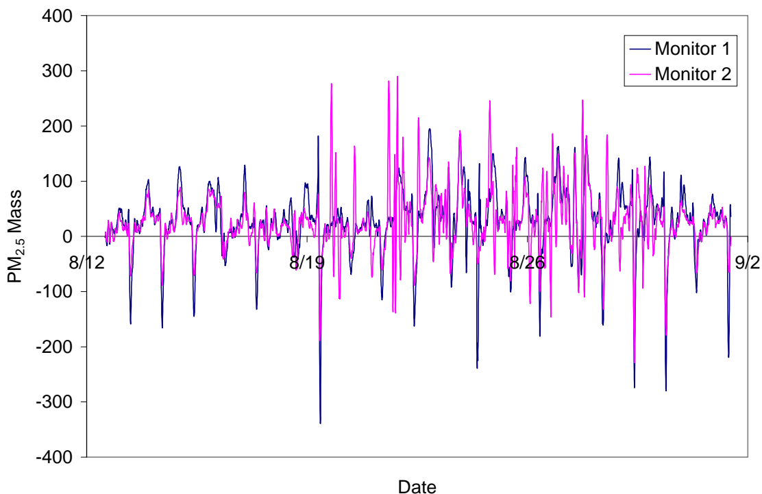
Figure 6-1. PM 2.5 Readings from Duplicate FH 62 C14 Monitors During Phase I of Verification Testing
