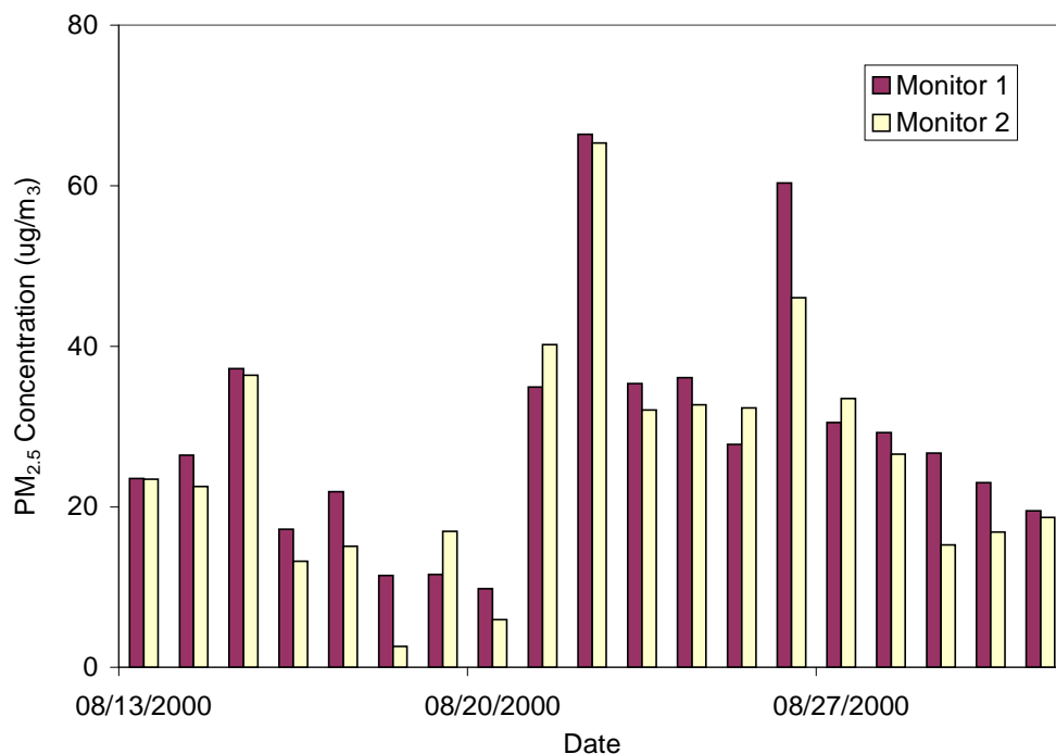
Figure 6-2a. Noon-to-Noon Average PM 2.5 Concentrations from Duplicate FH 62 C14 Monitors Measured During Phase I of Verification Testing
