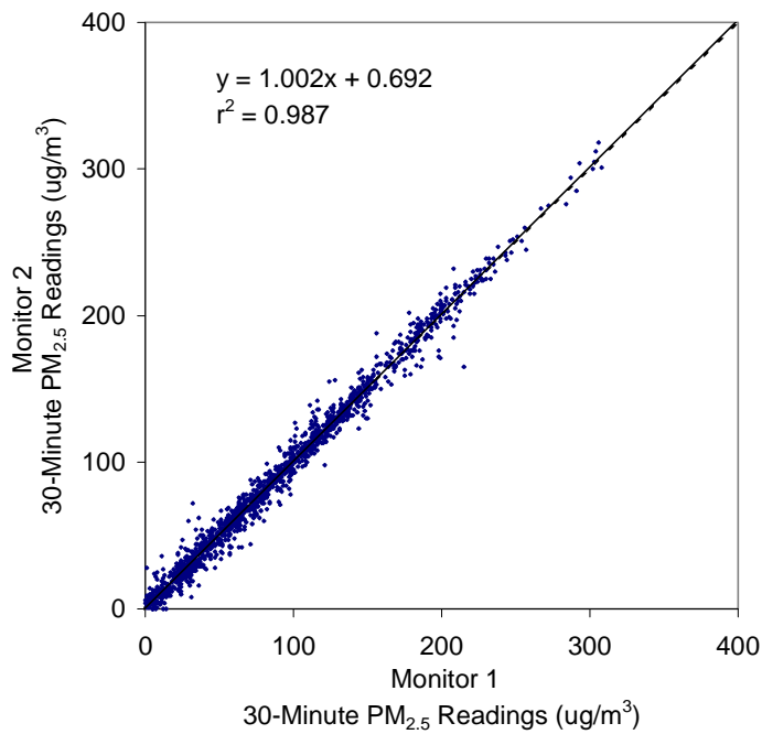
Figure 6-4b. Correlation Plot of the 30-Minute PM 2.5 Data from Duplicate FH 62 C14 Monitors During Phase II of Verification Testing
