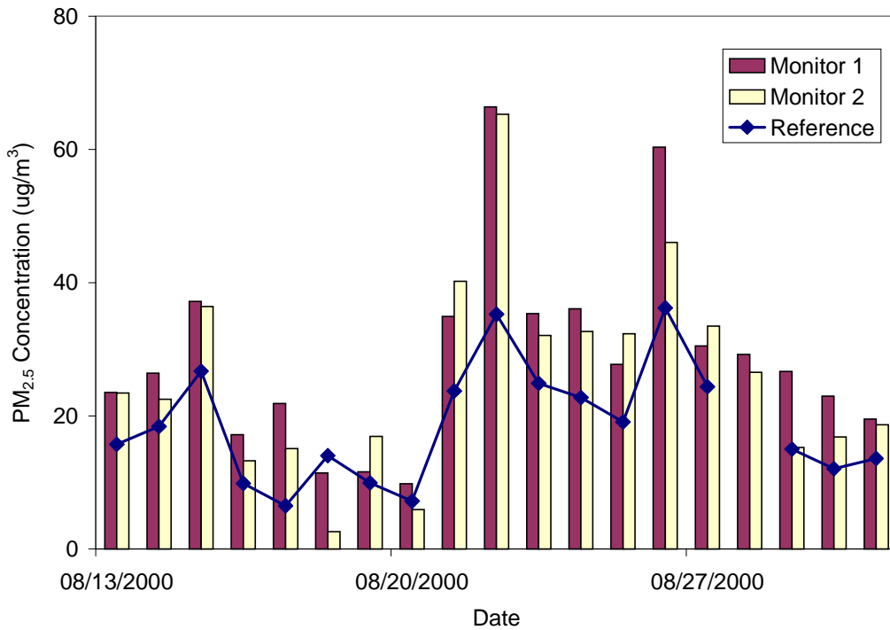
Figure 6-3a. Daily PM 2.5 Concentrations and the 24-Hour PM 2.5 Average Concentrations from Duplicate FH 62 C14 Monitors During Phase I of Verification Testing
