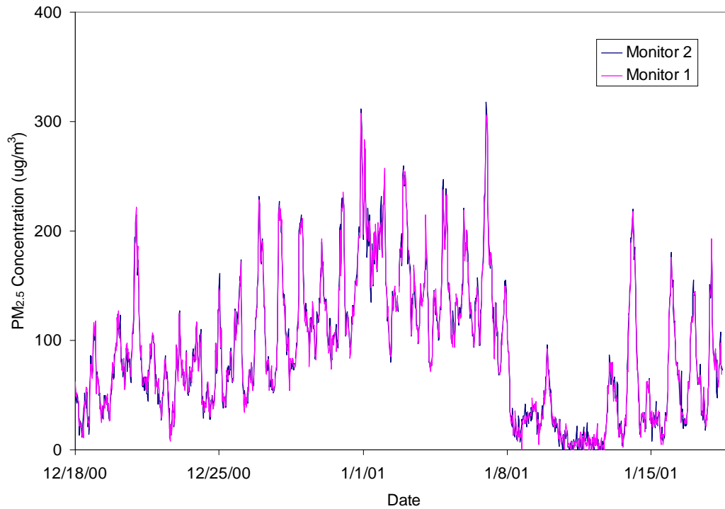
Figure 6-4a. Time Series Plot from Duplicate FH 62 C14 Monitors During Phase II of Verification Testing
