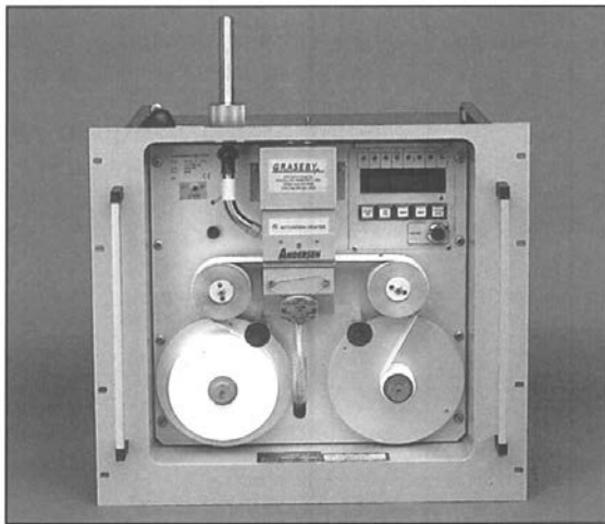
Figure 2-1. Thermo Andersen FH 62 C14 Ambient Dust Monitor
