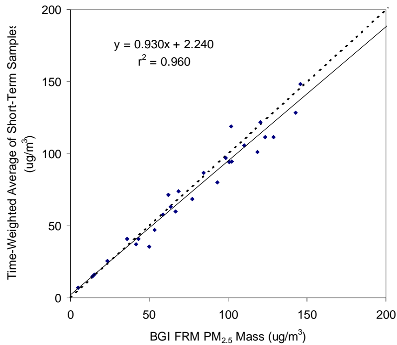
Figure 6-7. Correlation Plot for the Time-Weighted Average of the Short-Term Samples and the \text{PM}_{2.5} FRM for Phase II
