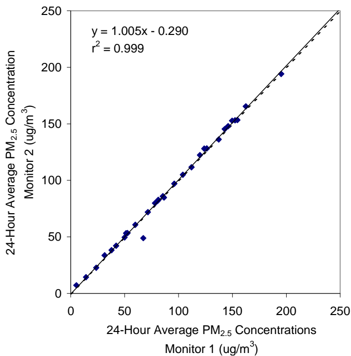
Figure 6-5b. Correlation Plot of the 24-Hour Average PM 2.5 Concentrations from Duplicate FH 62 C14 Monitors During Phase II of Verification Testing
