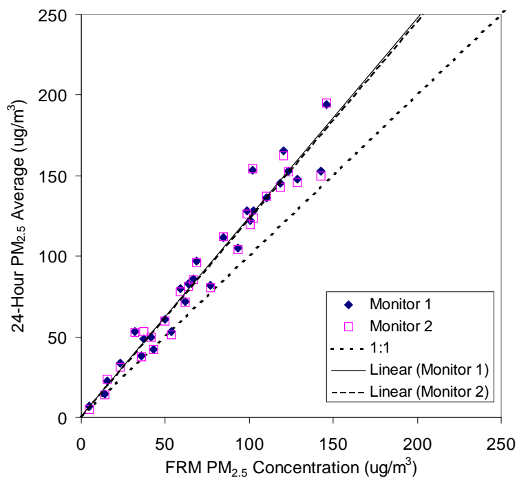
Figure 6-6b. Correlation Plot of 24-Hour Average Concentrations from Duplicate FH 62 C14 Monitors and the PM 2.5 FRM During Phase II of Verification Testing
