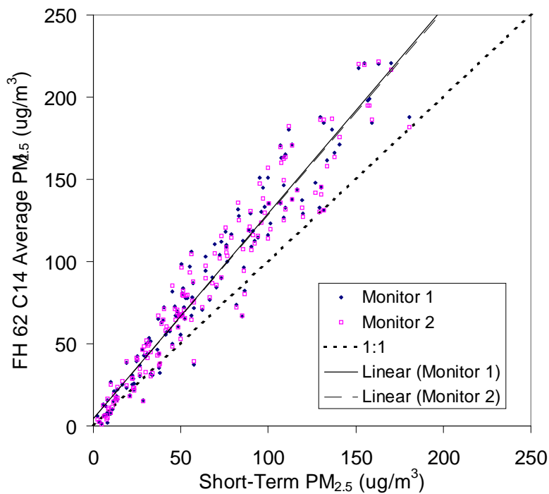
Figure 6-8. Correlation Plot of Short-Term Monitoring Results and the Corresponding Averages from the Duplicate FH 62 C14 Monitors During Phase II of Verification Testing
