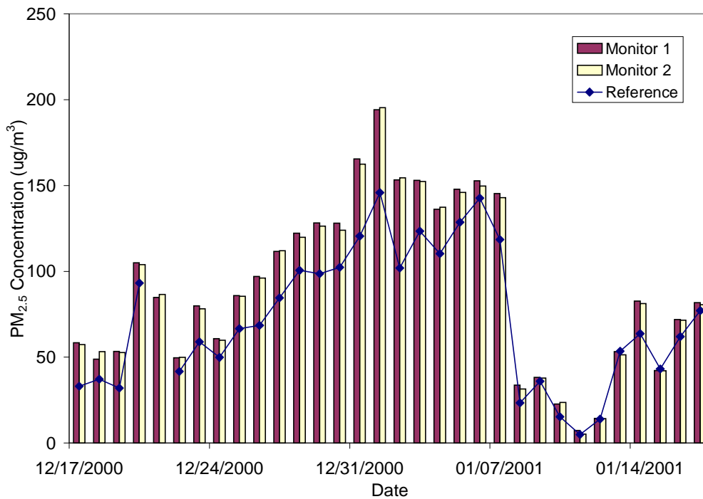
Figure 6-6a. Midnight-to-Midnight Average Concentrations from Duplicate FH 62 C14 Monitors and the PM 2.5 FRM Results During Phase II of Verification Testing
