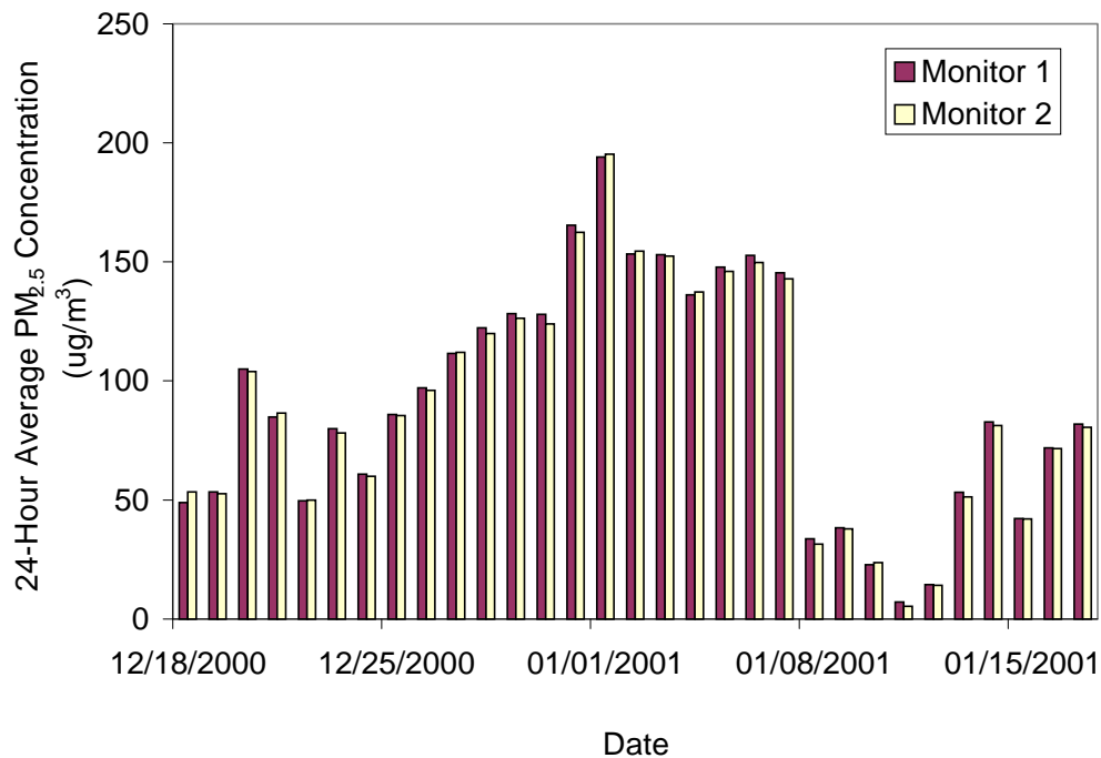
Figure 6-5a. 24-Hour Average PM 2.5 Concentrations from Duplicate FH 62 C14 Monitors During Phase II of Verification Testing
