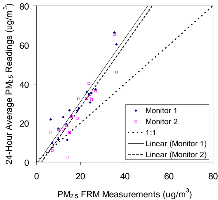
Figure 6-3b. Correlation Plot of the 24-Hour Averages from Duplicate FH 62 C14 Monitors and the PM 2.5 FRM Results During Phase I of Verification Testing
