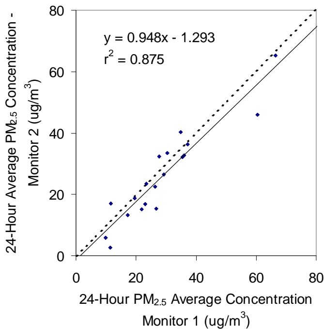
Figure 6-2b. Correlation Plot of 24-Hour PM 2.5 Concentrations from Duplicate FH 62 C14 Monitors During Phase I of Verification Testing
