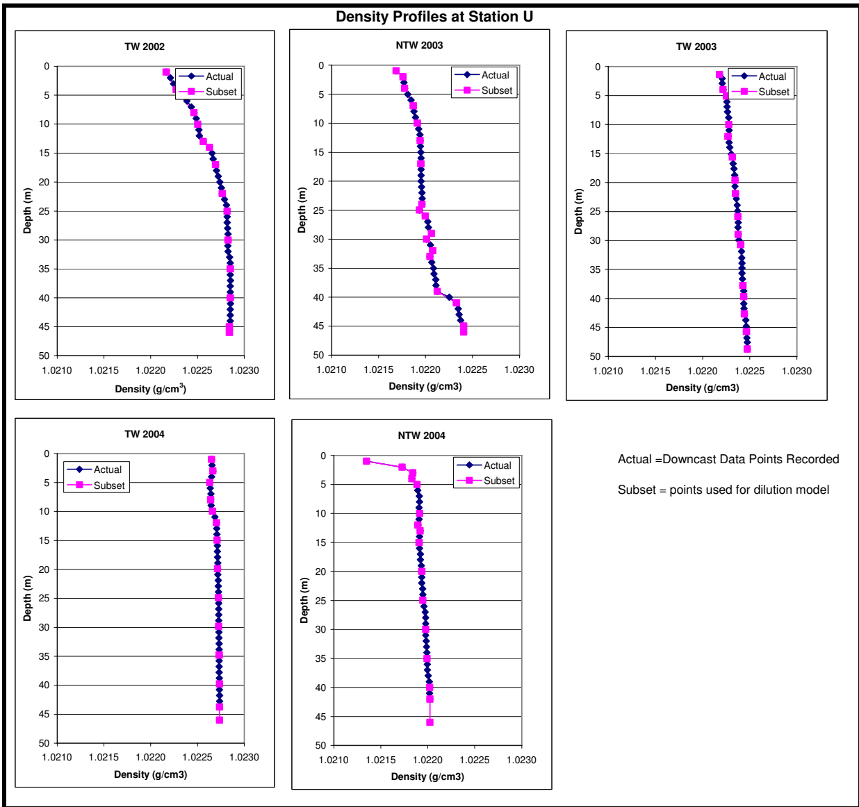
Density Profile Data Used in Model Runs to Determine Critical Conditions
