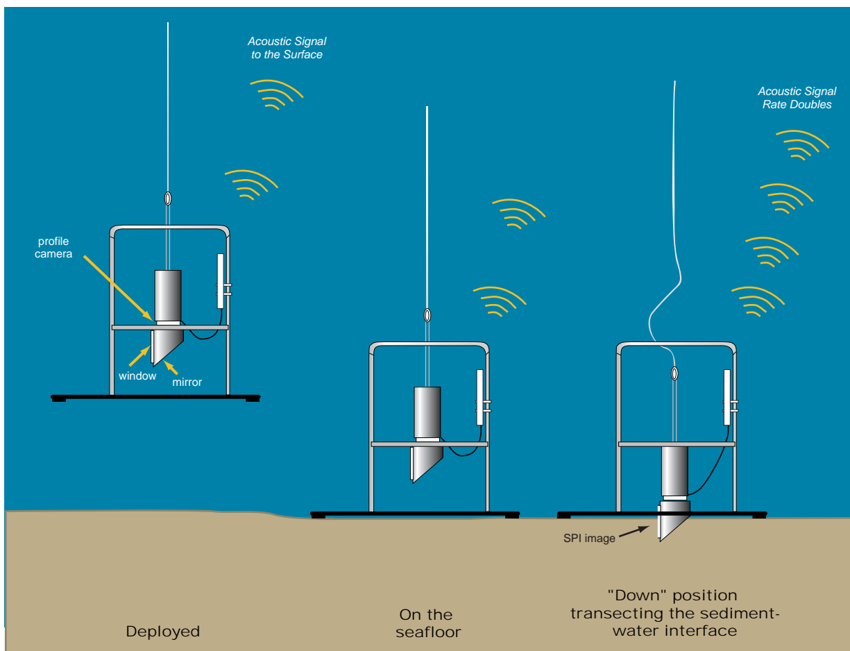
Figure 3: Deployment and operation of the sediment profile imaging (SPI) system; acoustic pinger signal doubles for 10 seconds after strobe is fired to signal successful image acquisition in deep-water operations.
