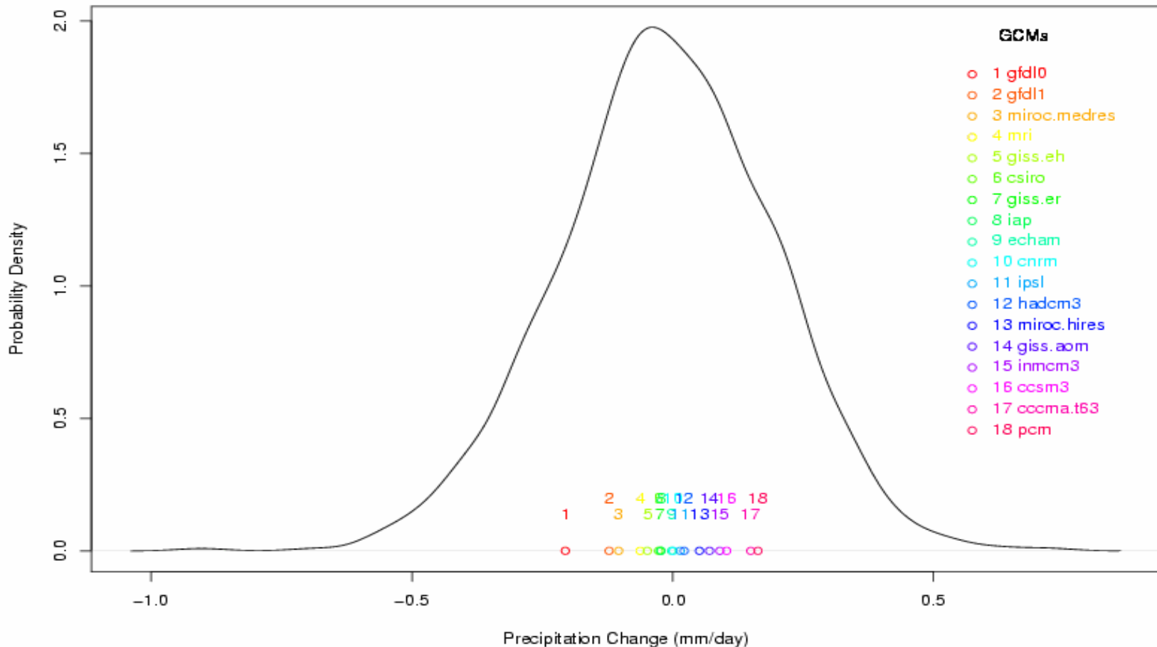
Probability Density Function – a1b_precip_2030_annual
