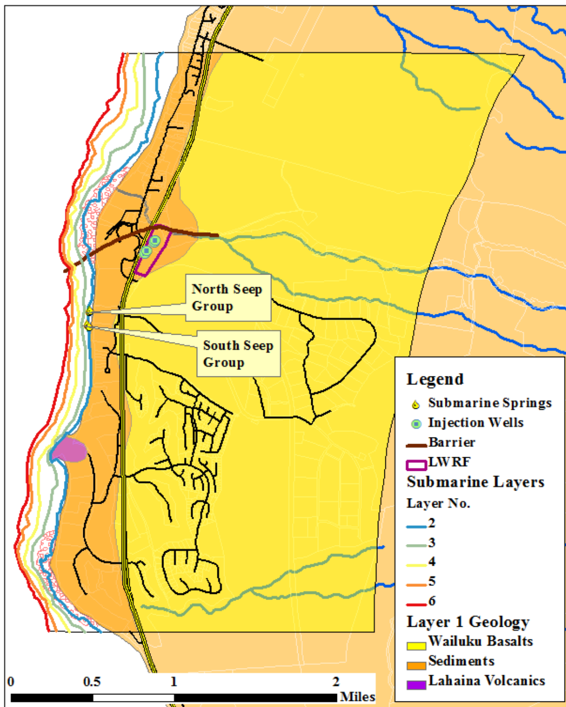
Figure ES-13: The conceptual model for the Lahaina Groundwater Study showing the extent of the submarine layers Western boundaries of layers 2 through 6 followed the 6.6, 18, 29.5, 41, and 54 ft depth contours respectively.
