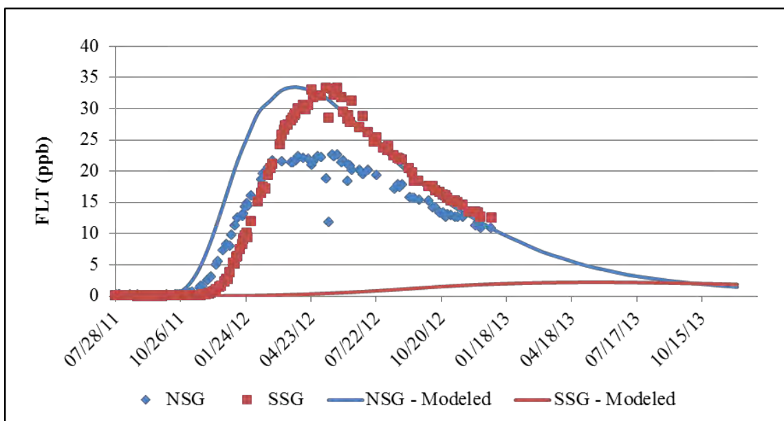
Figure 5-9: The measured BTCs compare the model results when a horizontal flow barrier was included in the model.
