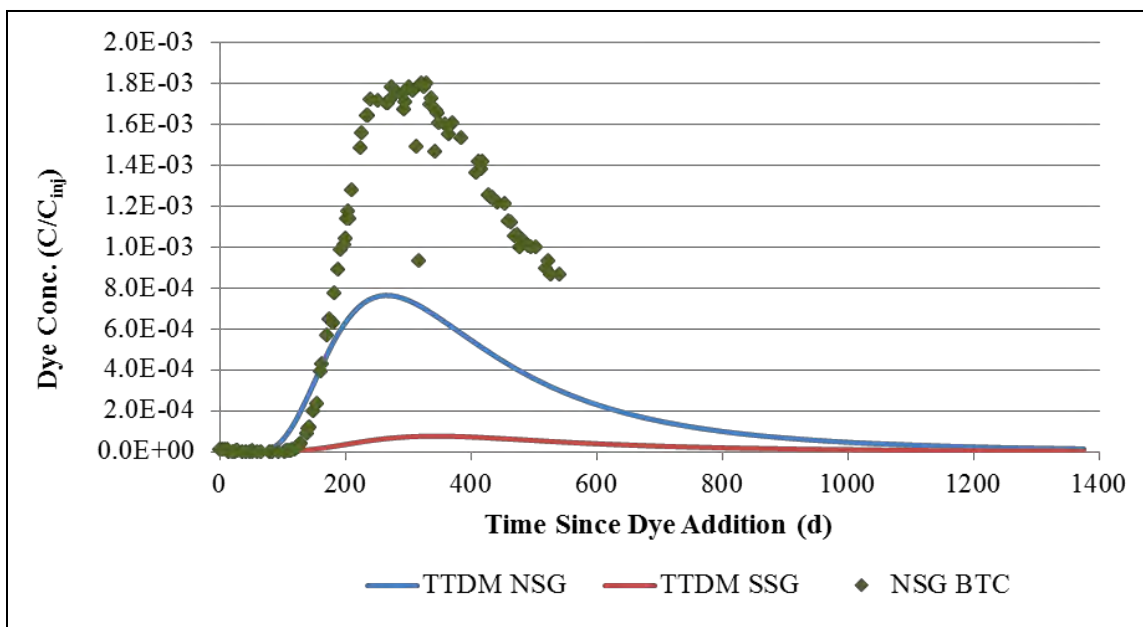
Figure 5-3: Results of the Tracer Test Design Model shown as the ratio of the submarine spring concentration to that at injection wells on the day of dye addition.
