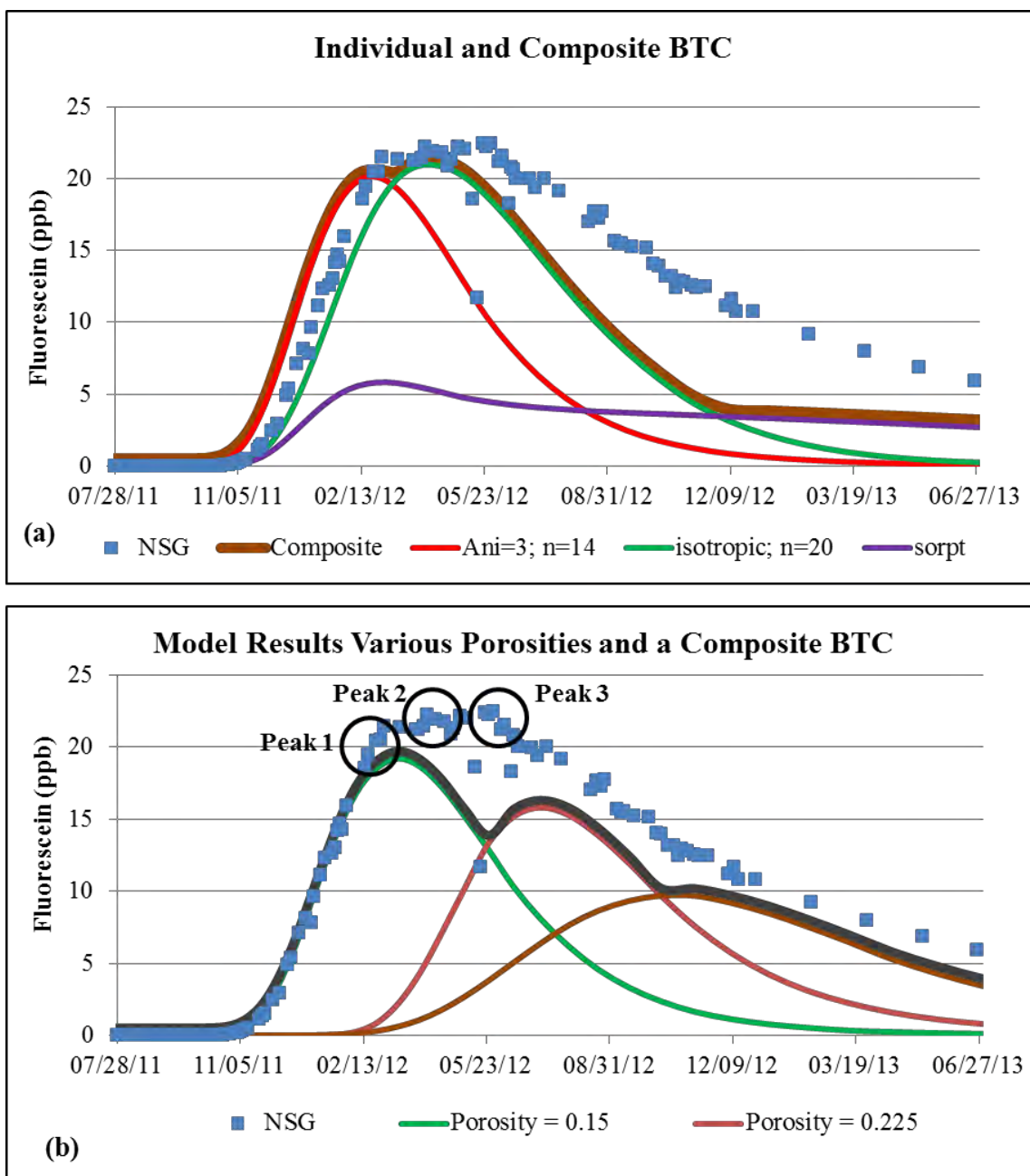
Figure 5-23: Individual simulated individual BTCs and composites showing a possible resulting BTC with multiple peaks and a plateau.
