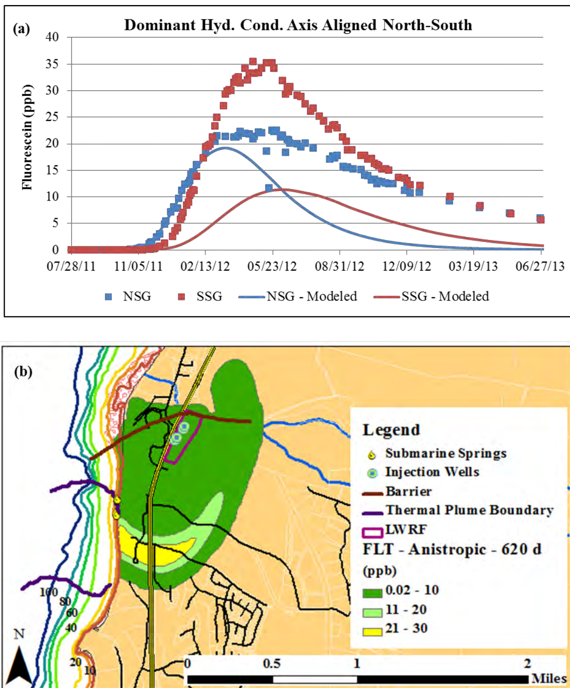
Figure ES-15: The FLT model results showing (a) the measured and simulated BTCs; and (b) simulated plume 620 days after dye addition.
