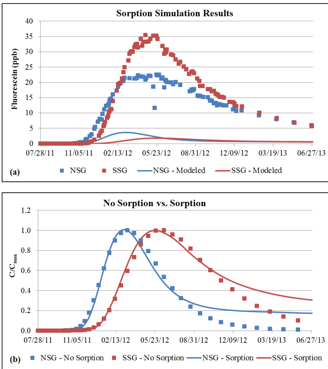
Figure 5-14: Modeled BTC when sorption of FLT was simulated. Figure 5-14a shows the measured and simulated BTCs when sorption was simulated.
