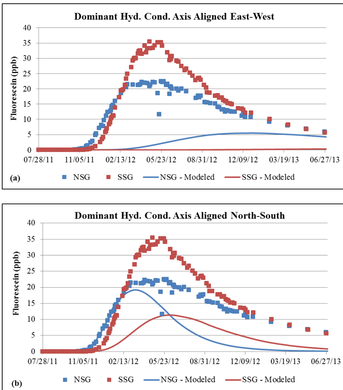
Figure 5-15: The simulated and measured BTCs with differing anisotropy ellipse alignments. When the dominant axis of the hydraulic conductivity is aligned east-west (Figure 15a), the simulated BTCs are severely attenuated. A much better agreement between the simulated and measure BTCs results when the dominant axis of hydraulic conductivity is aligned north-south.
