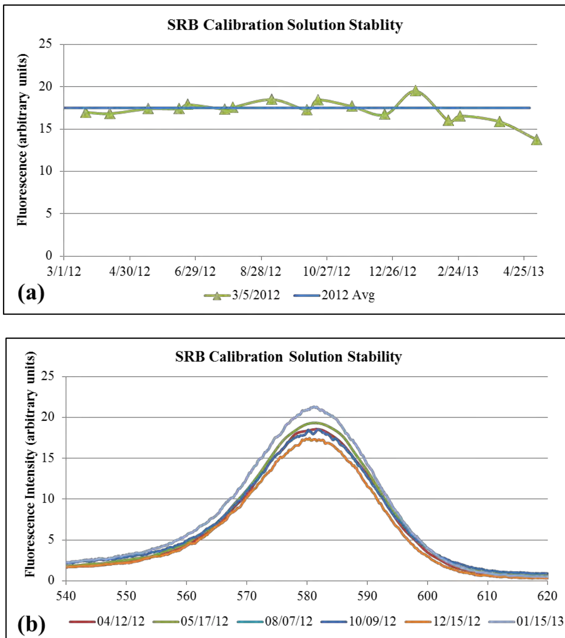
Figure 4-33: Time series graphs showing fluorescence intensity measurements and emission wavelength synchronous scans of the 1 ppb SRB calibration solution.
