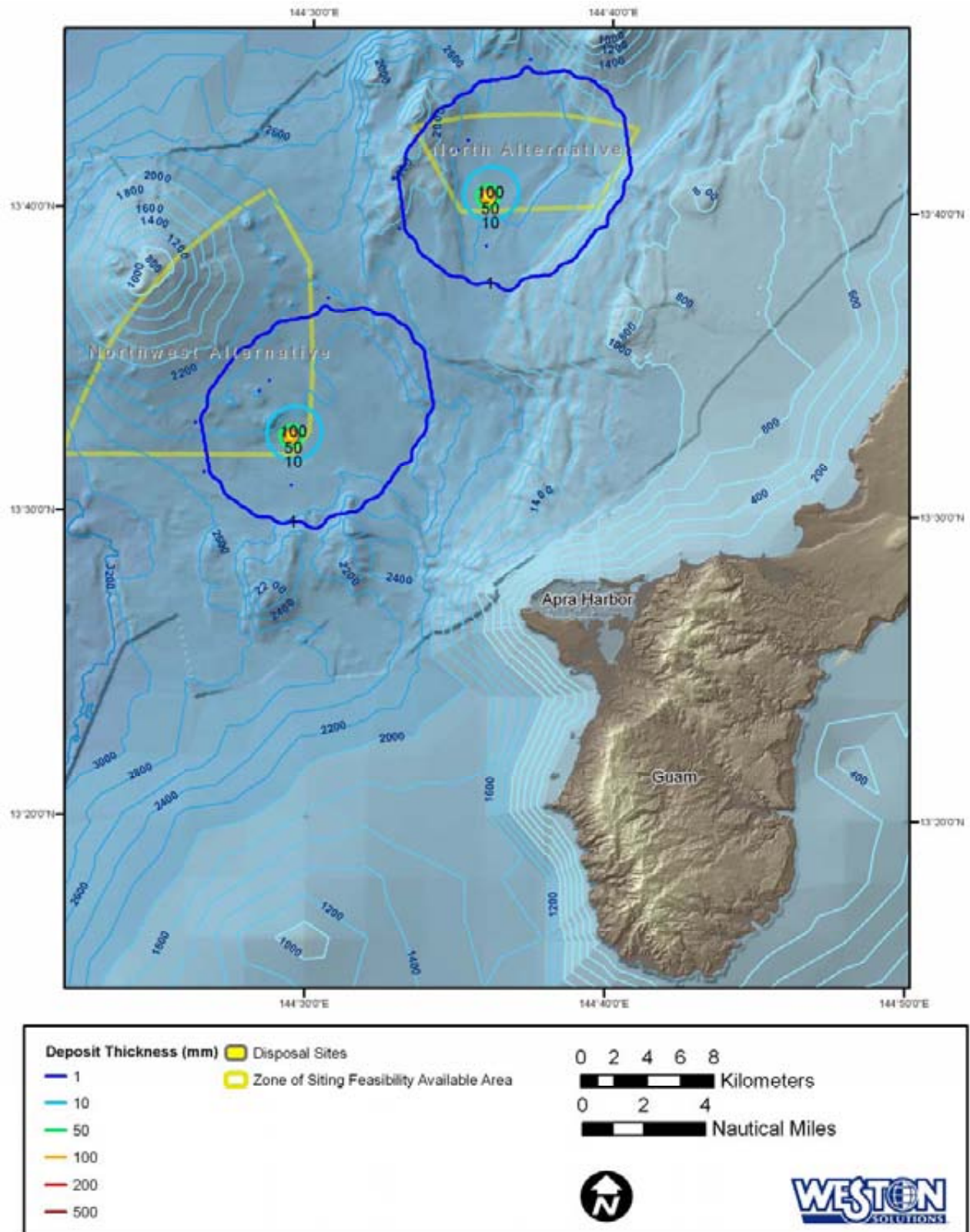
Figure 46. Expanded View of Isopachs Showing Increasing Deposit Thickness for the Disposal of 1 mcyc of Predominantly Fine-Grained Material
