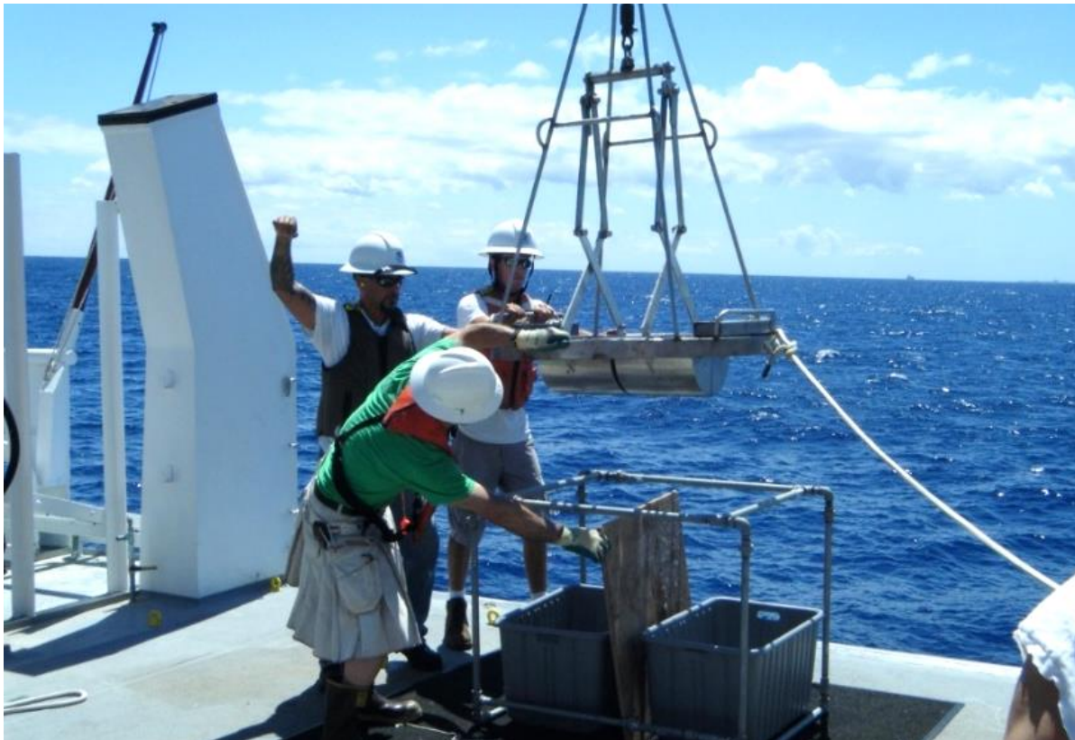
Figure 9. Double Van Veen sediment sampler deployed from the Hi'ialakai.
