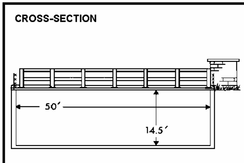
Figure 6. Typical Channel Cross-Section for Walnut Creek
