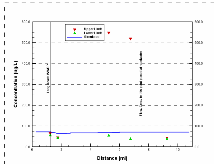
Figure 47. Simulated vs. observed Lower Total Zinc of Coyote Creek in September 2003 (zero for non-detects)
