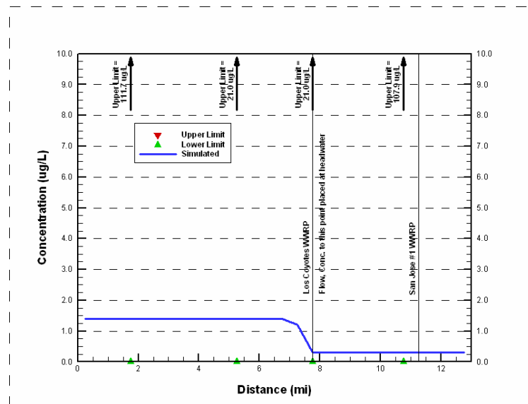
Figure 27. Simulated vs. observed Total Lead of San Gabriel River in September 2003 (zero for non-detects)
