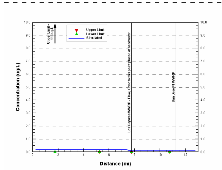
Figure 26. Simulated vs. observed Total Lead of San Gabriel River in September 2002 (zero for non-detects)
