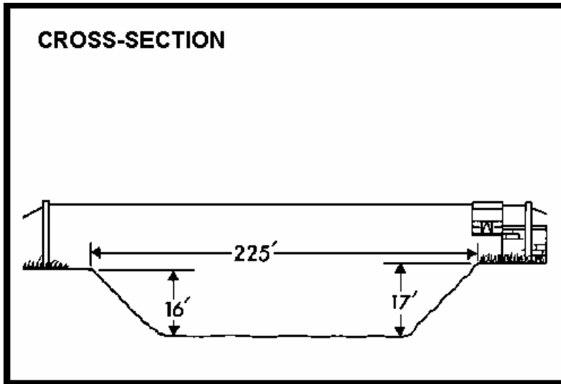
Figure 5. Typical Channel Cross-Section for San Jose River
