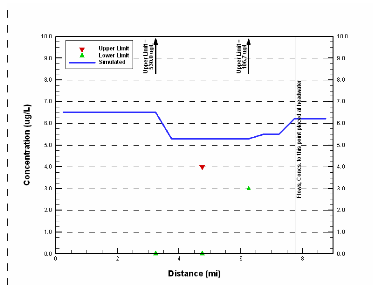
Figure 39. Simulated vs. observed Total Lead of Walnut Creek in September 2003 (zero for non-detects)
