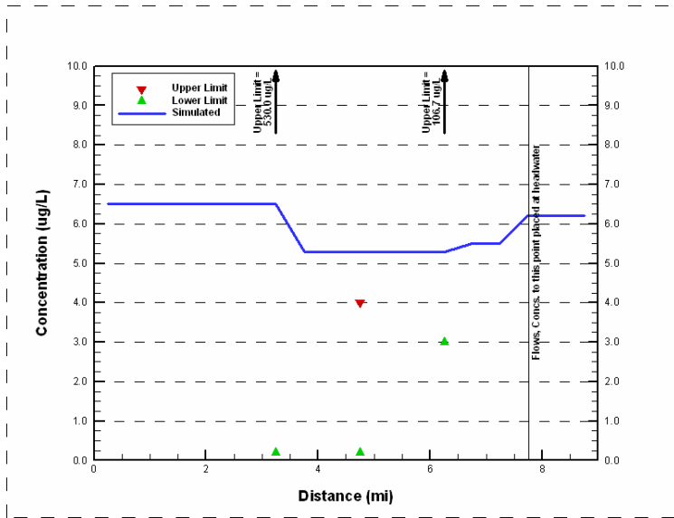
Figure 37. Simulated vs. observed Total Lead of Walnut Creek in September 2003 (1/2 detection limit for non-detects)
