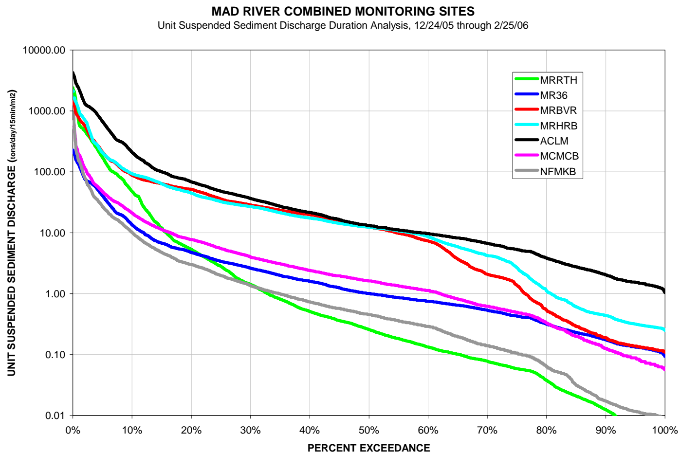
Figure 7. Mad River Unit SSD Duration Analysis, 12/24/05 through 2/25/06
