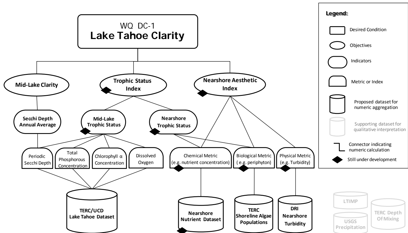
Figure 17-2. Lake Tahoe Clarity Indicator Framework Diagram.
