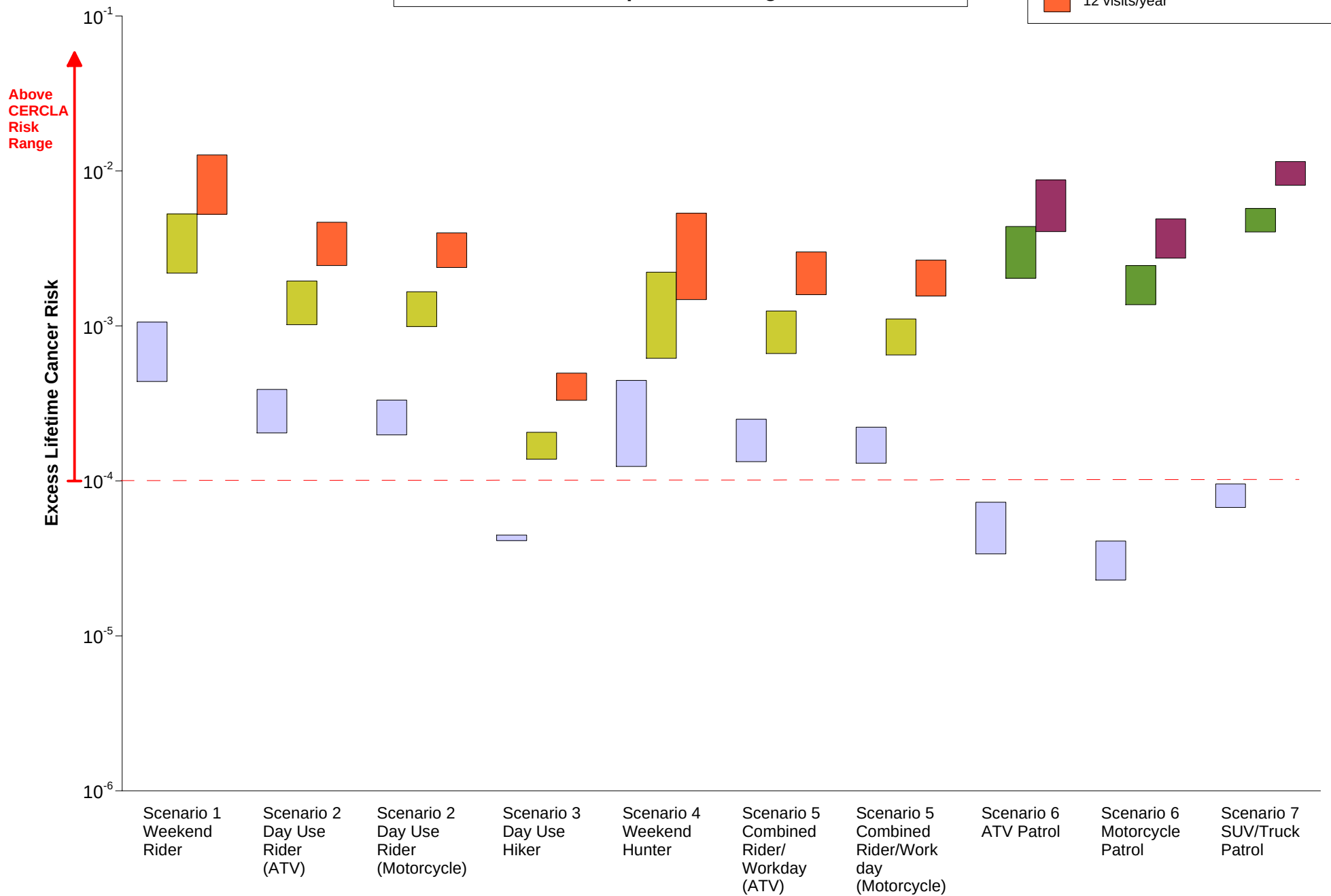
Figure 11: Adult Cancer Risk, Scenarios 1 – 7 Mean and 95%UCL Exposures Using OEHA Unit Risk
