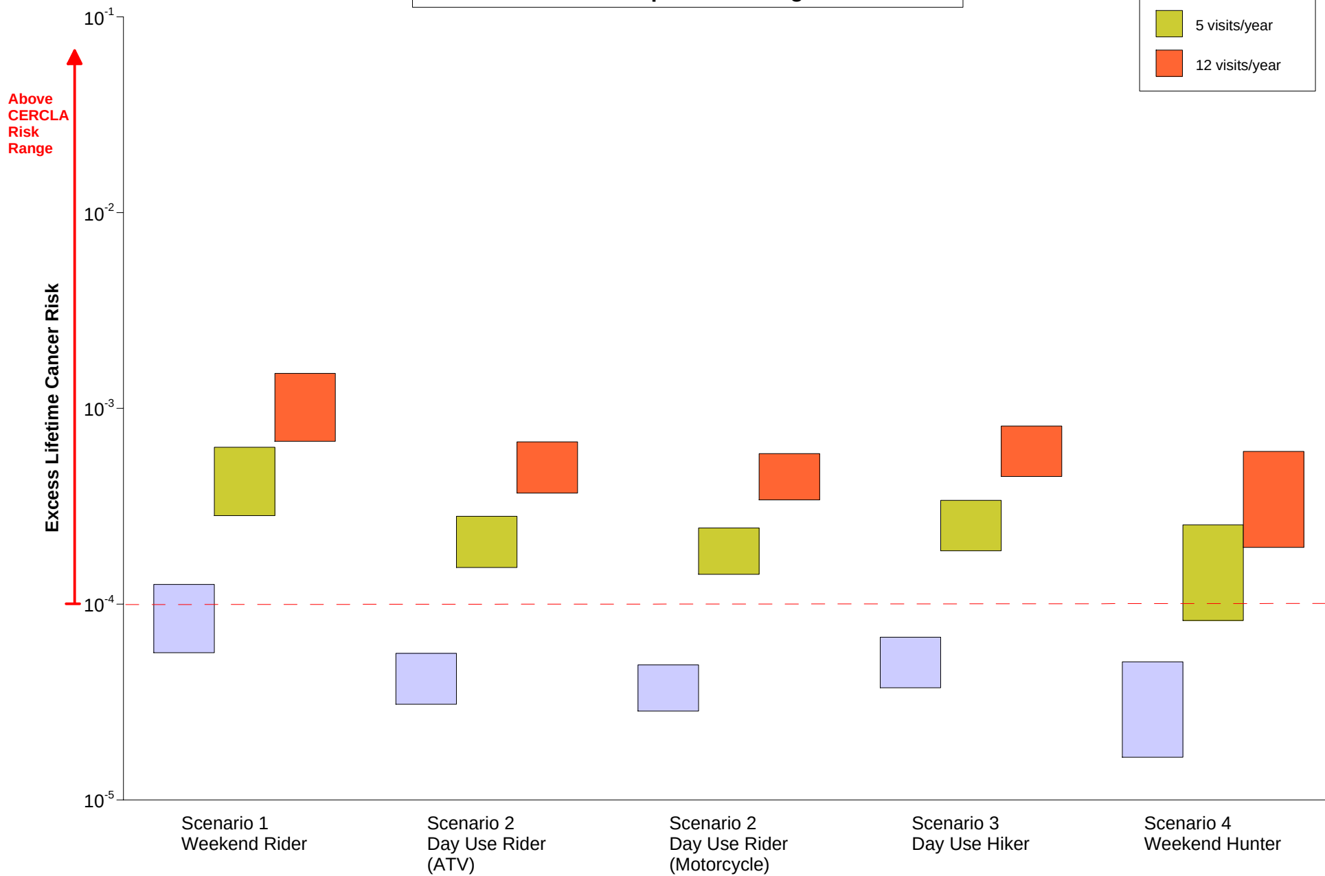
Figure 12: Child/Adult Cancer Risk, Scenarios 1 – 4 Mean and 95%UCL Exposures Using IRIS Unit Risk
