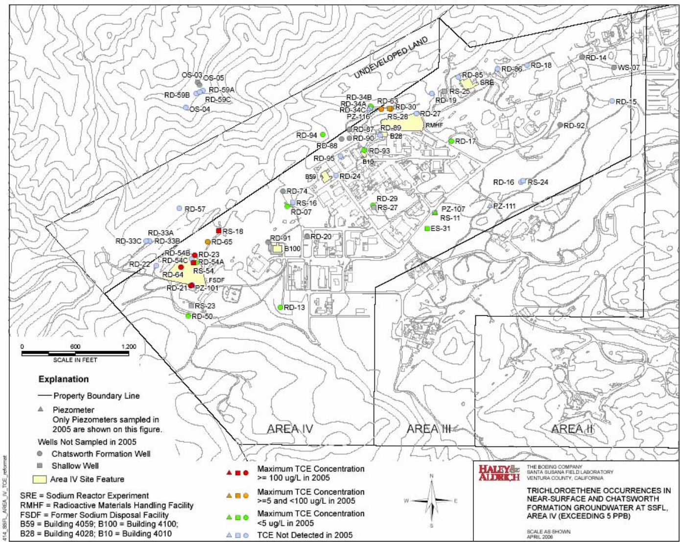
Figure 6-3. TCE Occurrences in Groundwater at SSFL, Area IV (exceeding 5 ppb)
