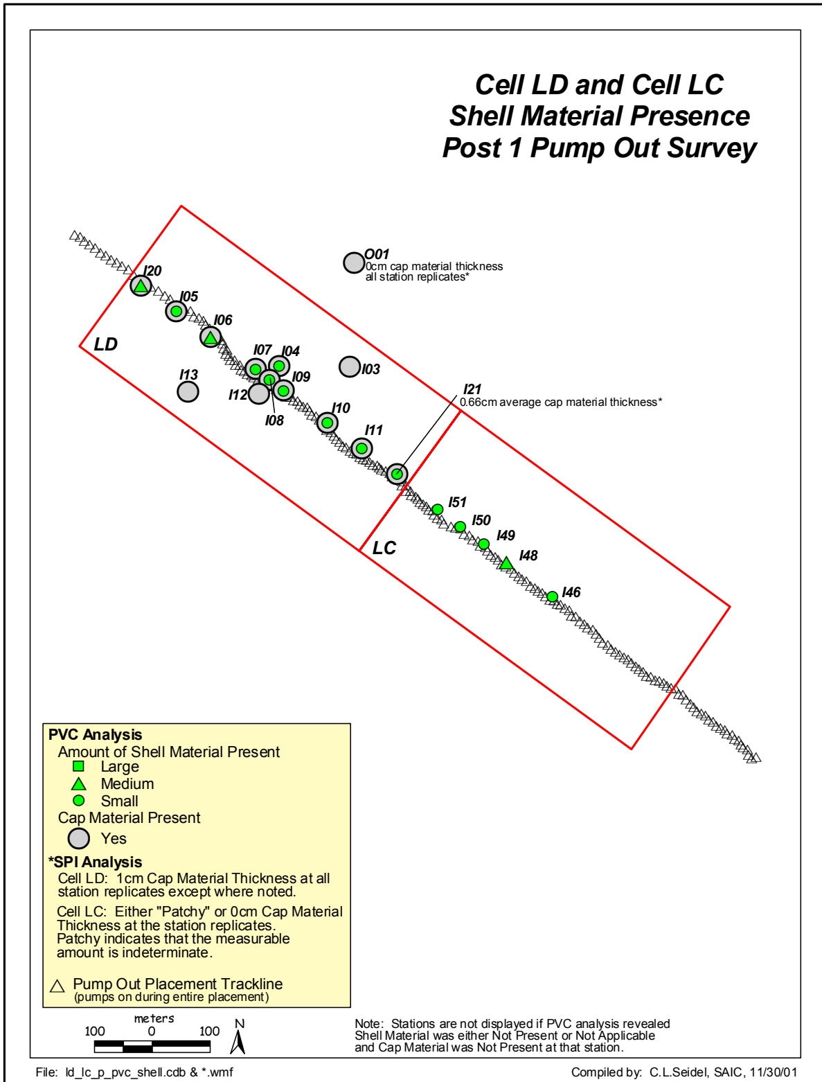
Figure 3-71. Extent of cap and shell material based on plan view camera (PVC) analysis – Post 1 survey in Cells LD and LC
