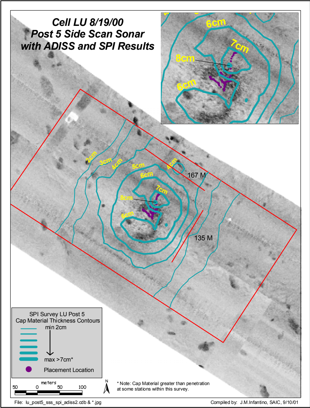
Figure 3-49. Results of the side-scan sonar survey after five cap placement events with SPI contours overlaid
