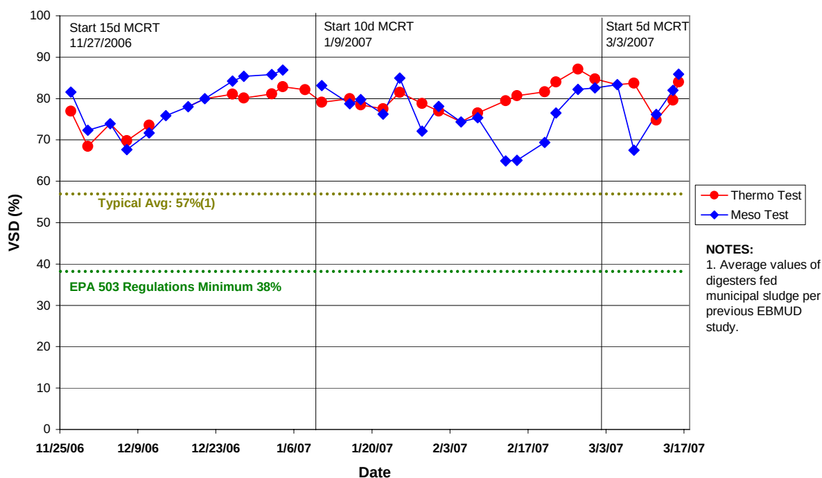
Figure 3.11 Anaerobic Food Waste Digester Volatile Solids Destruction
