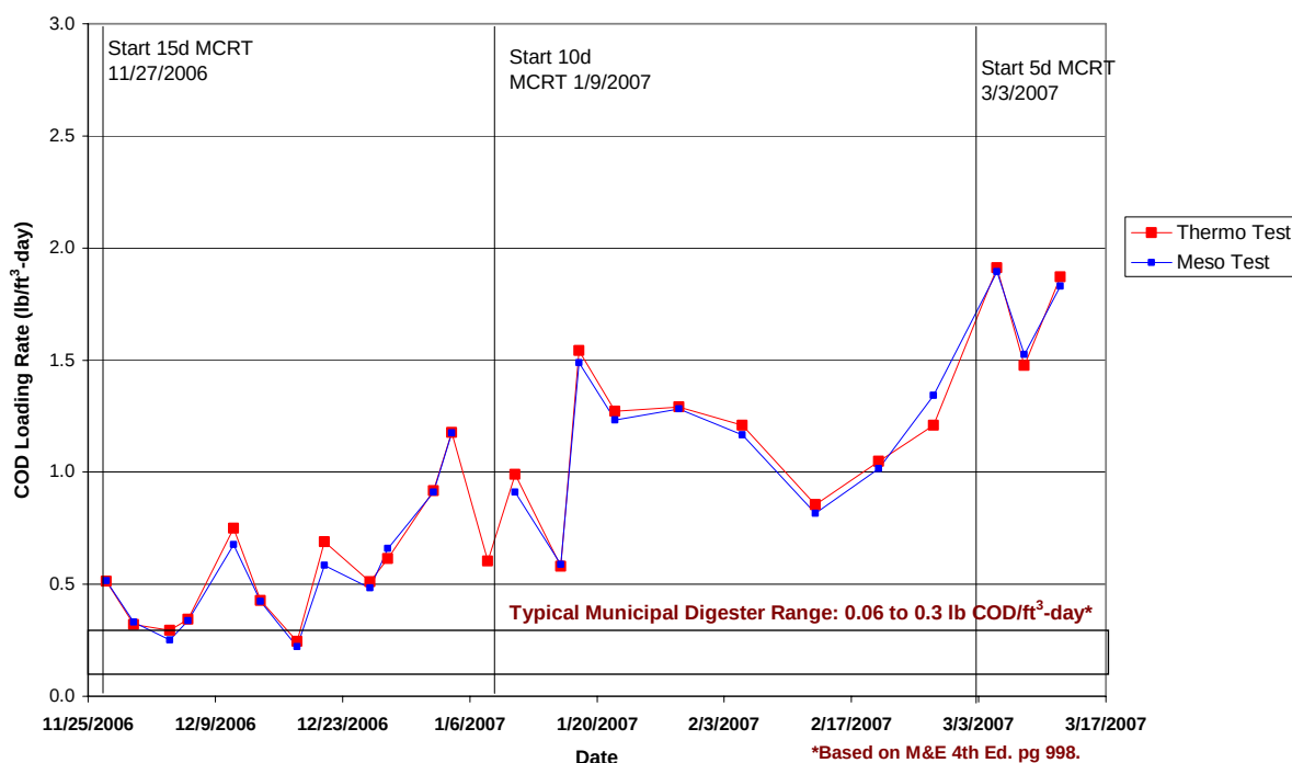
Figure 3.15 Anaerobic Food Waste Digester COD Loading Rate
