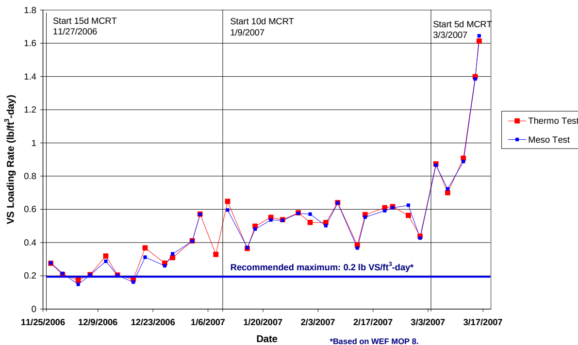
Figure 3.10 Anaerobic Food Waste Digester Volatile Solids Loading Rate
