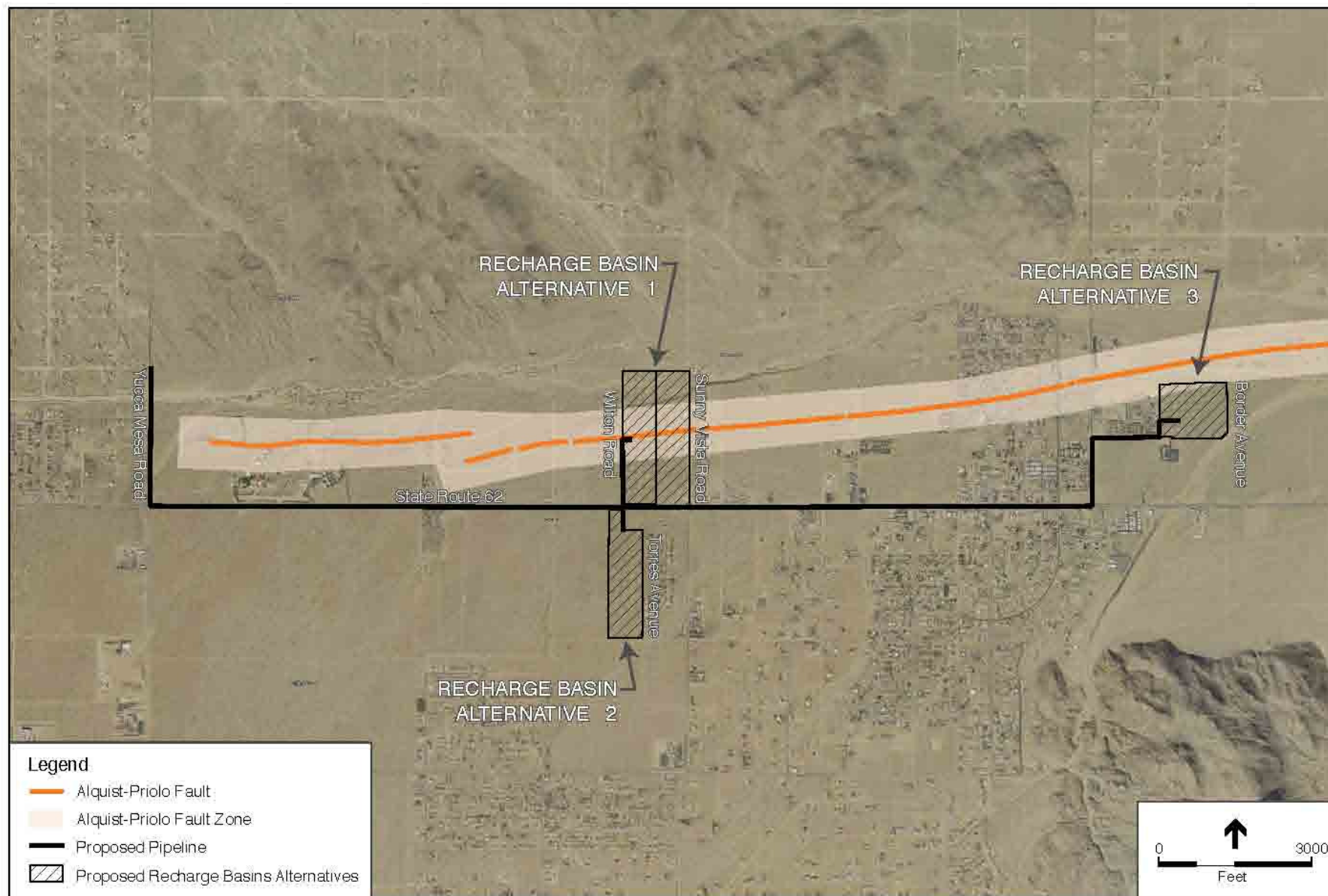
Figure 3.4-2 Alquist-Priolo Fault Zones
