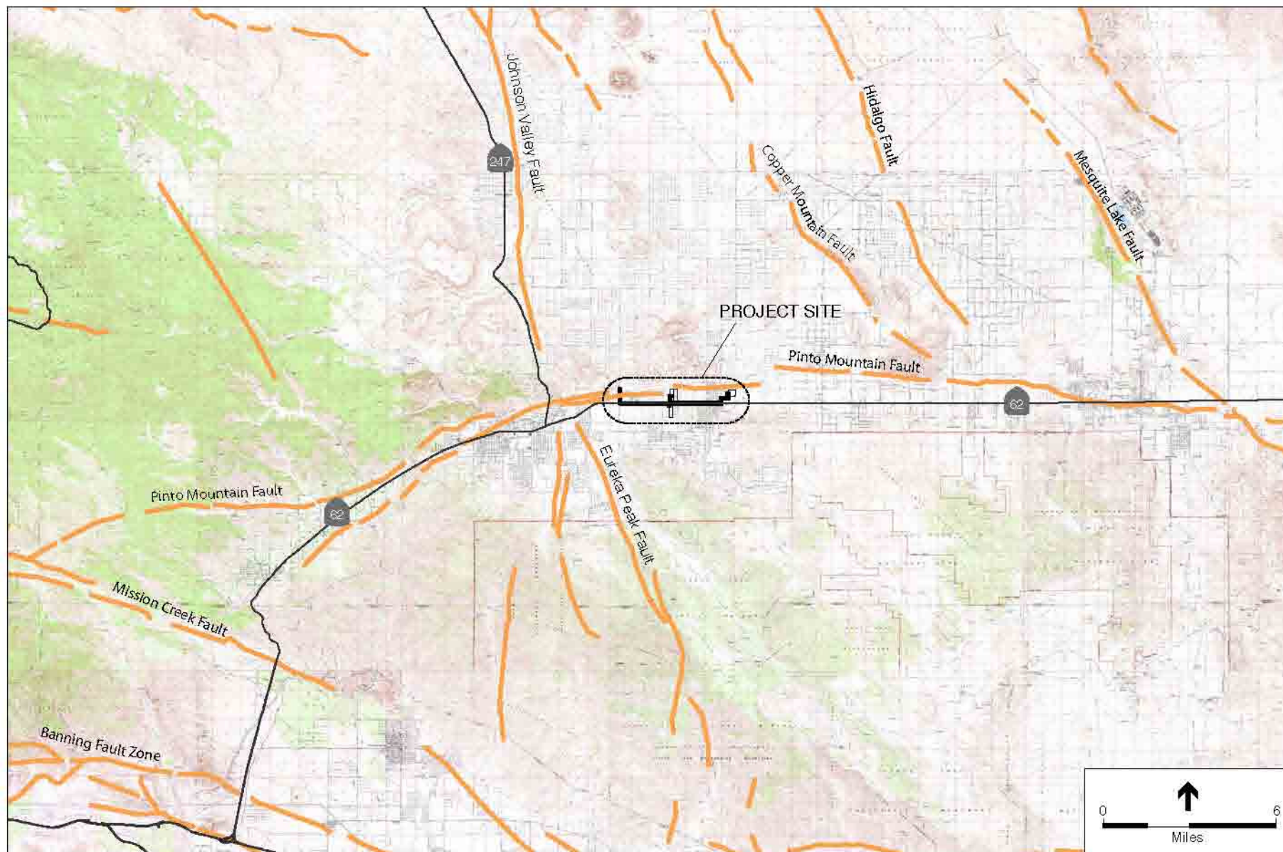
Figure 3.4-1 Regional Fault Zones
