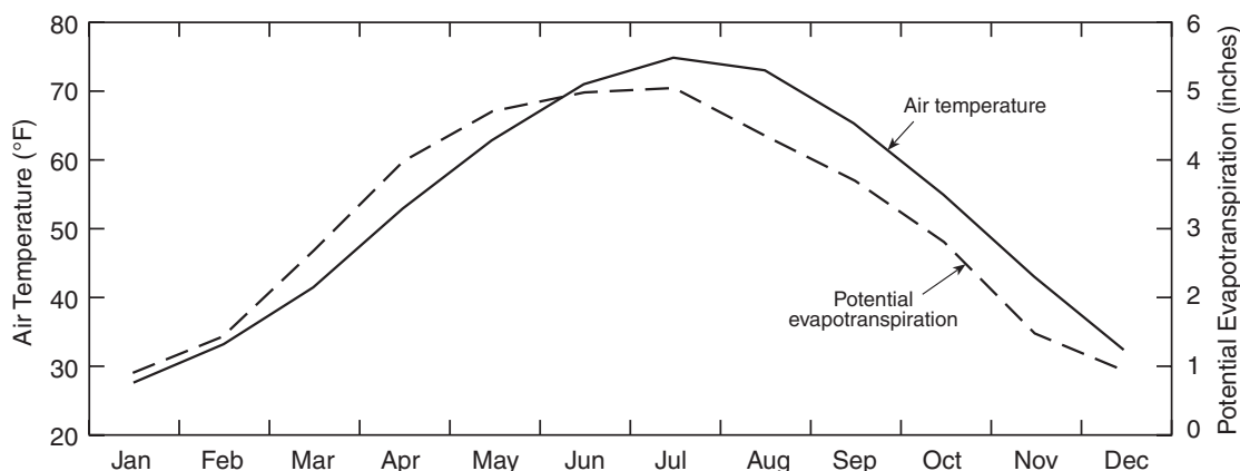
Figure A-6. Statewide Average Monthly Air Temperature and Potential Evaporation in Illinois, 1992-2004.
