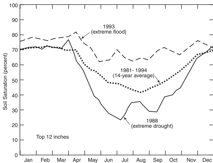
Figure 12. Annual Average Soil-Saturation Cycles in Illinois for the Top 12 in. for 1981-1994 (Thick Dotted Line); 1988 Extreme Drought (Solid Line); and 1993 Extreme Flood (Dashed Line) (from Findell and Eltahir, 1997).
