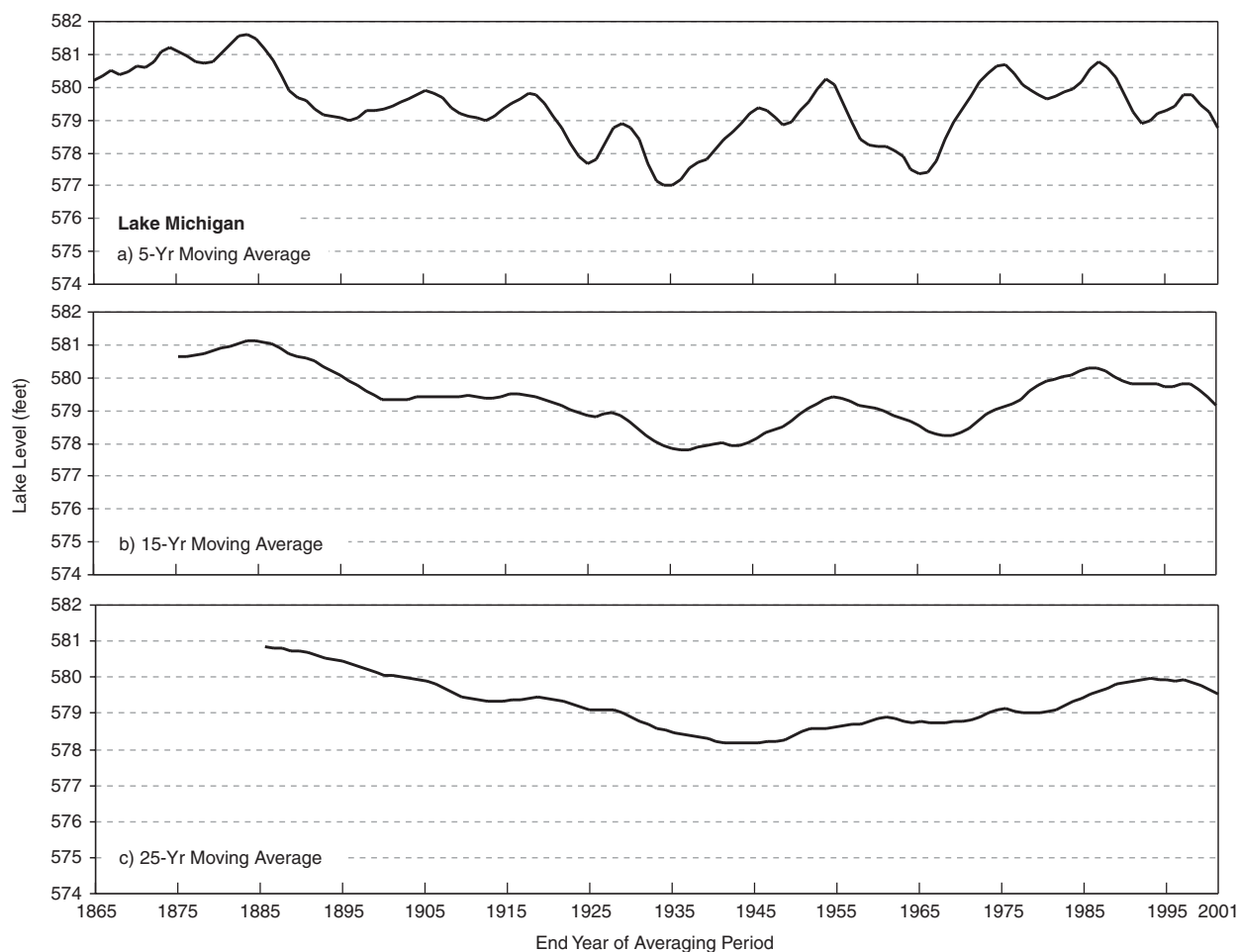
Figure B-1. The 5-, 15-, and 25-year Moving Averages of the Level of Lake Michigan, 1861-2001, with the Value Placed in the End Year of each Averaging Period, (from Changnon and Burroughs, 2003).
