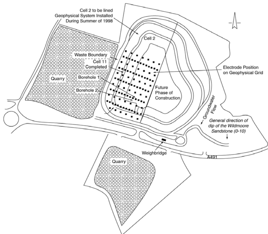
Figure 11. Sandy Hill Landfill geophysical electrode grid and borehole installation.
