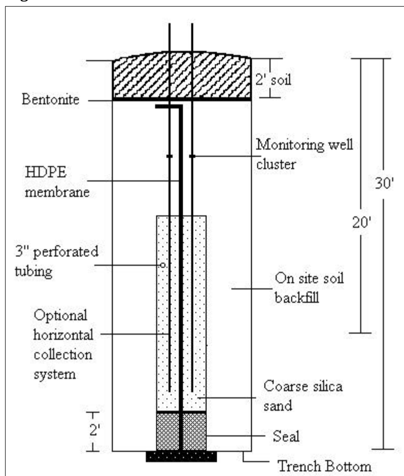
Figure 3: EnviroWall Barrier
