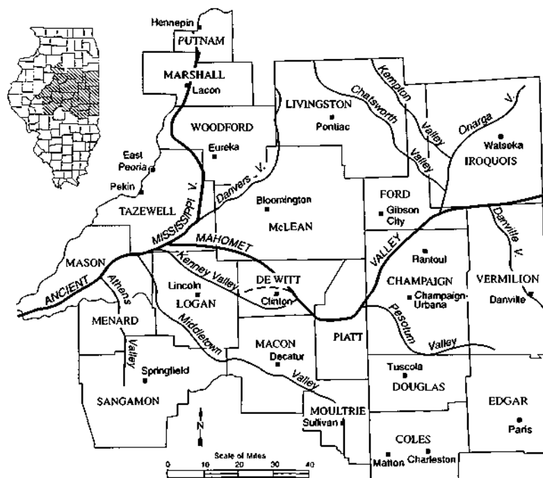
Figure 2. Thalweg of principal bedrock valleys and important tributaries in east-central Illinois (modified from Burch and Kelly, 1993)
