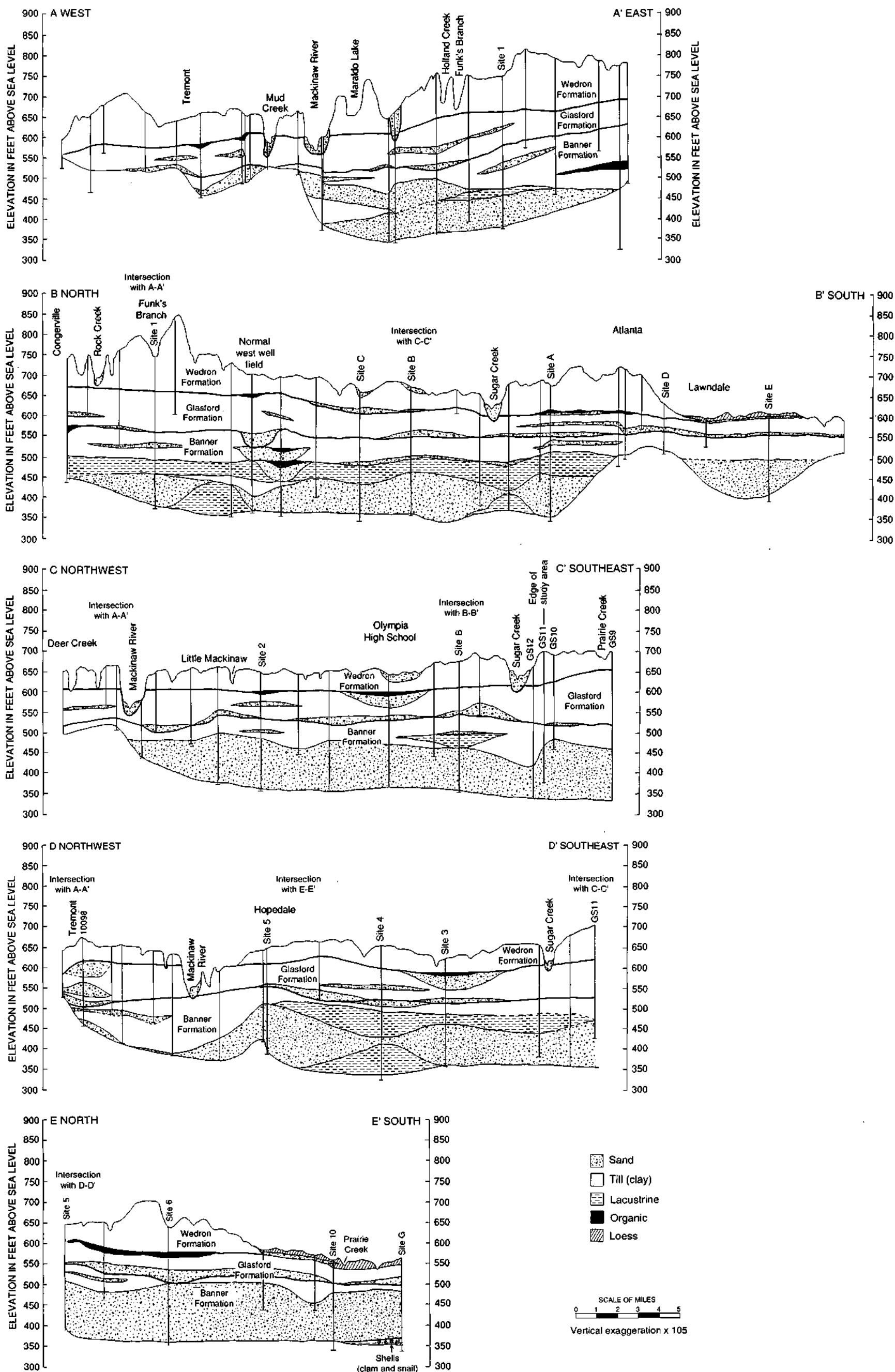
Figure 7. a) Northern east-west cross section A-A', b) Eastern north-south cross section B-B', c) Northern northwest-southeast cross section C-C', d) Southern northwest-southeast cross section D-D', and e) Western north-south cross section E-E' (see figure 5 for locations)
