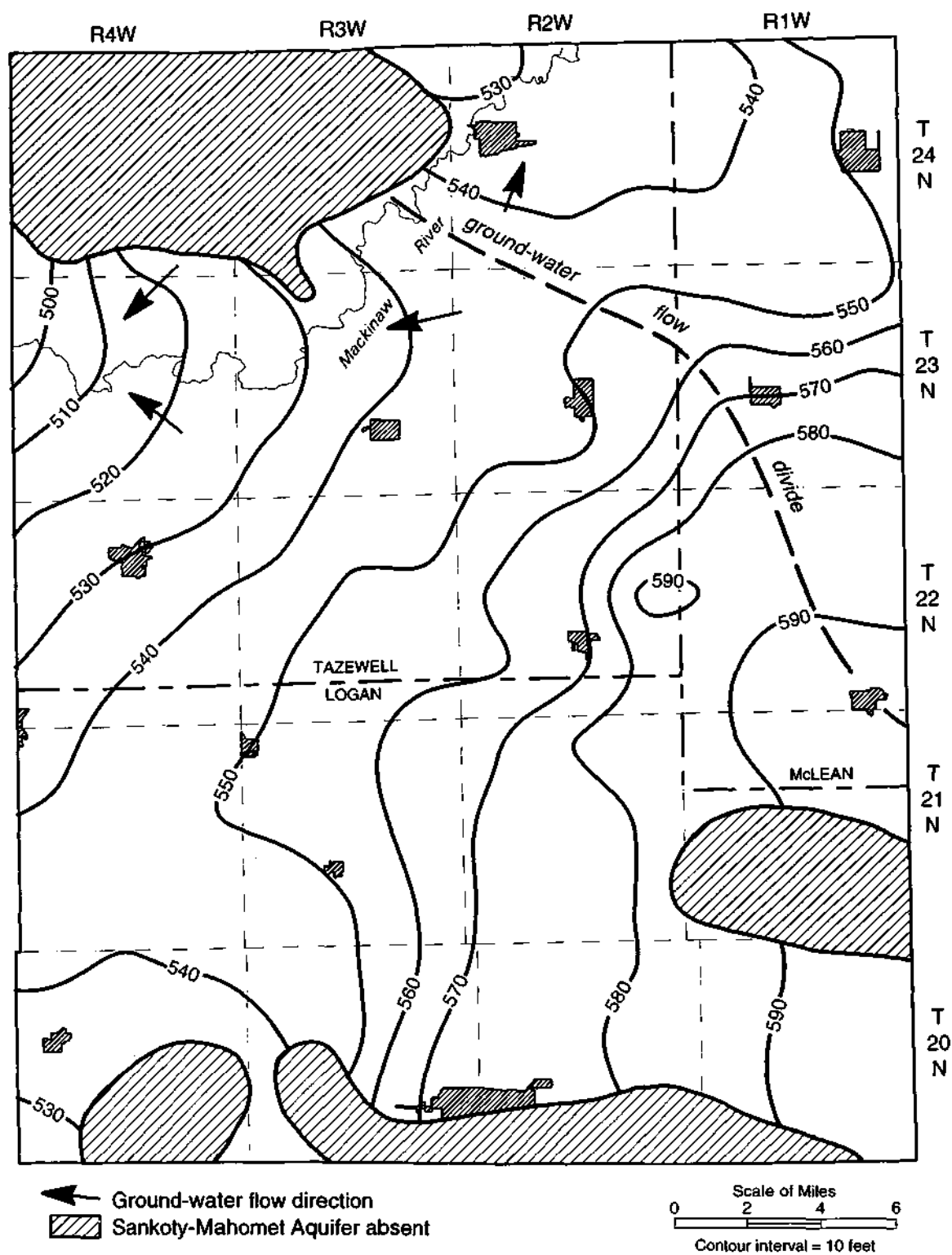
Figure 13. Potentiometric surface of the Sankoty-Mahomet aquifer system during spring 1993
