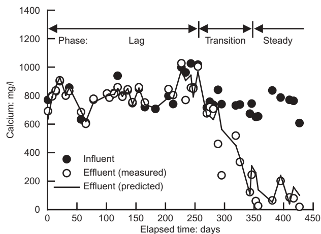
Fig. 8. Observed and calculated variation in effluent calcium concentration with time for a column test using 6 mm glass beads (data from VanGulck, 2003)
