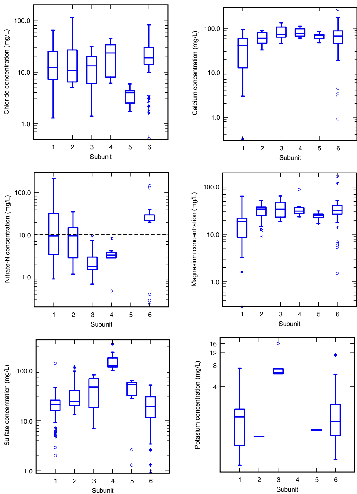
Figure 5.15 Box plot of chloride, nitrate-N, sulfate, calcium, magnesium, and potassium concentrations (excluding censored values) for the time-series samples.
