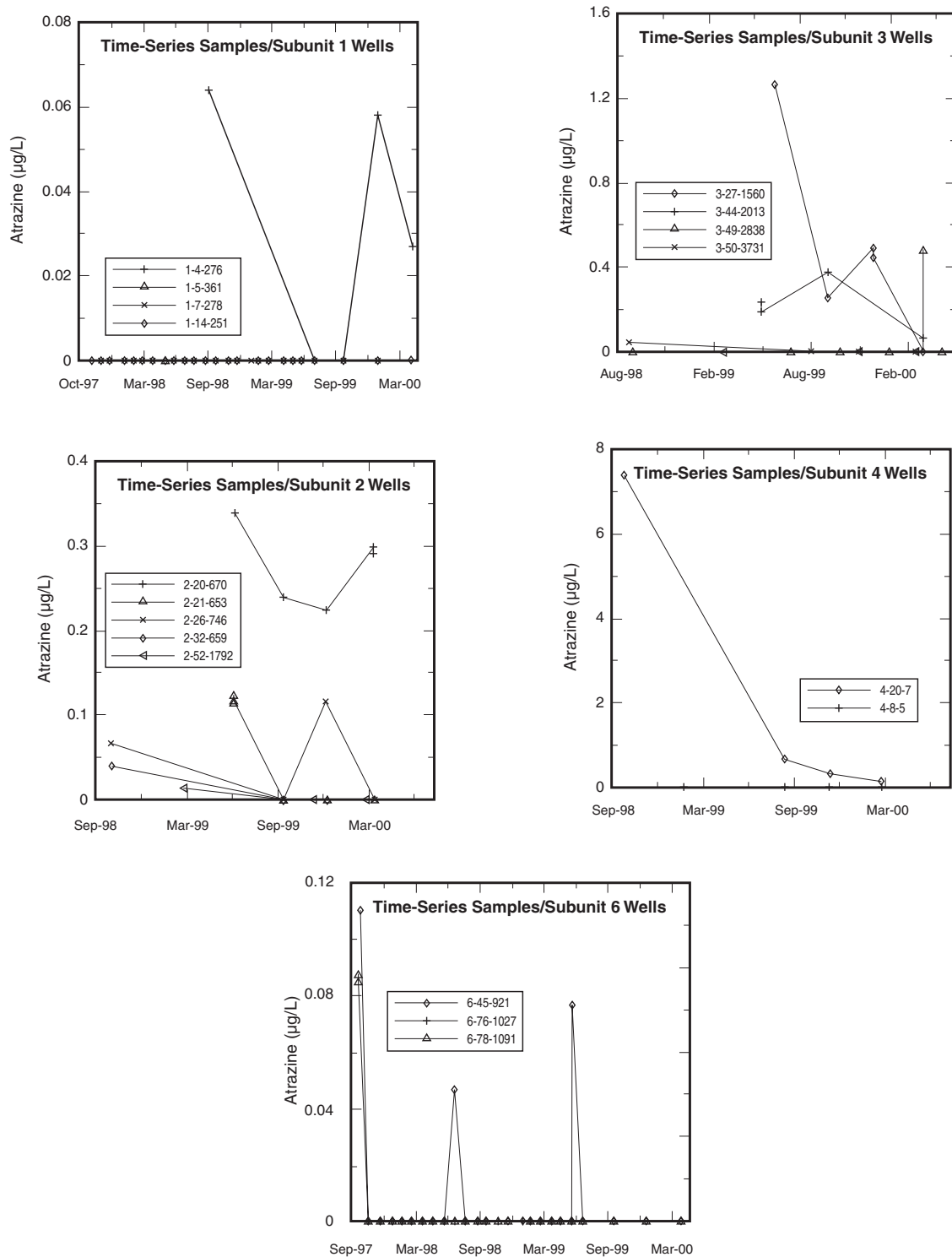
Figure 5.7 Atrazine concentration in the time-series wells. Samples with concentrations less than the method detection limit were plotted as 0.
