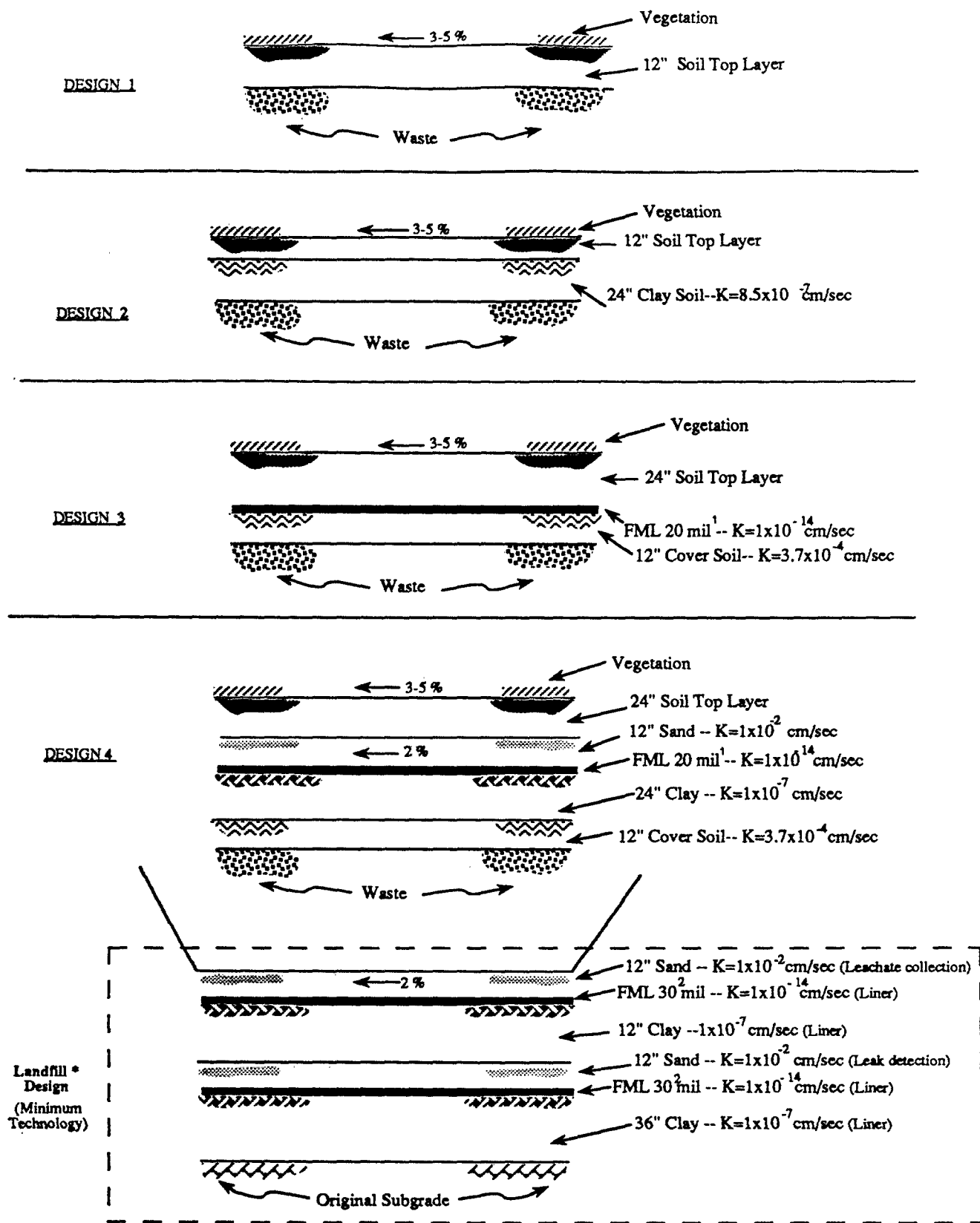
Figure C-1 Cap Design Details
